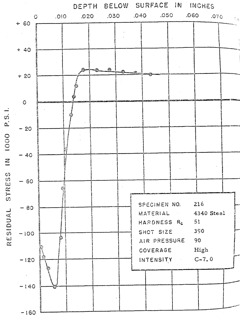
FIGURE 249. RESIDUAL STRESS DISTRIBUTION
