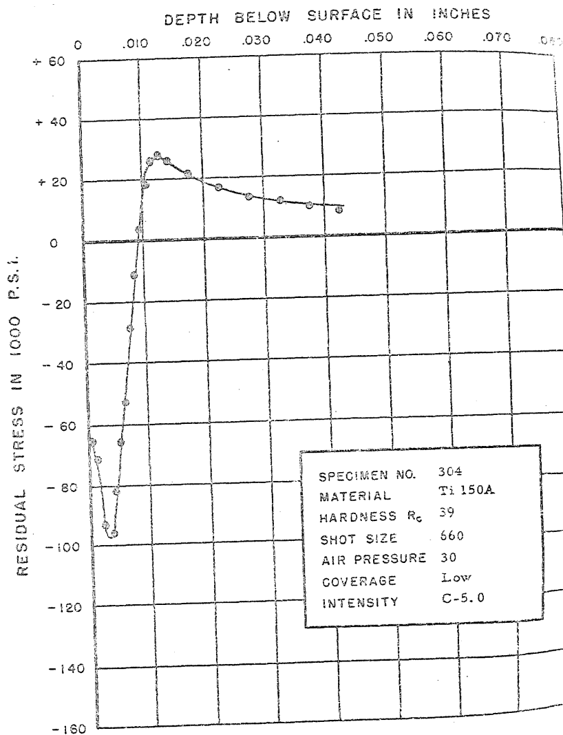
FIGURE 337. RESIDUAL STRESS DISTRIBUTION
