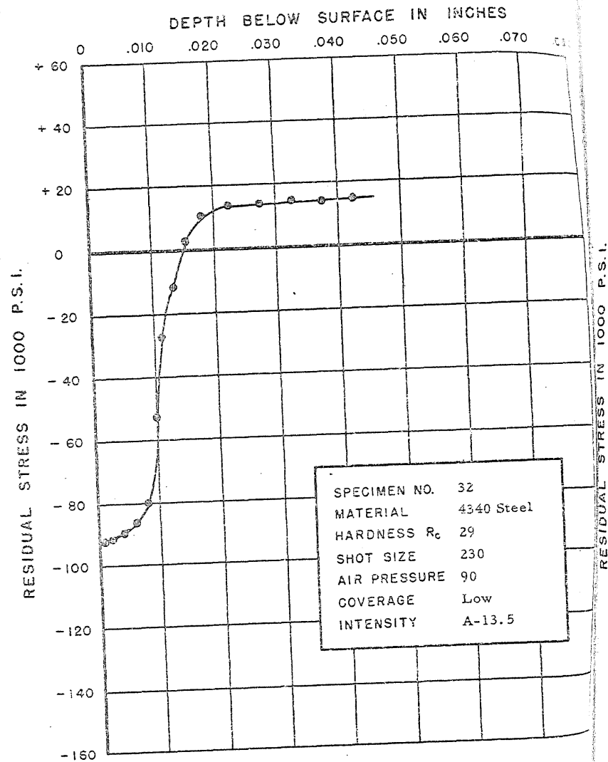
FIGURE 65. RESIDUAL STRESS DISTRIBUTION
