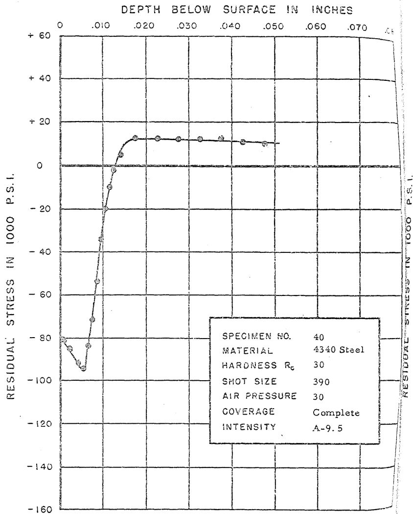
FIGURE 73. RESIDUAL STRESS DISTRIBUTION
