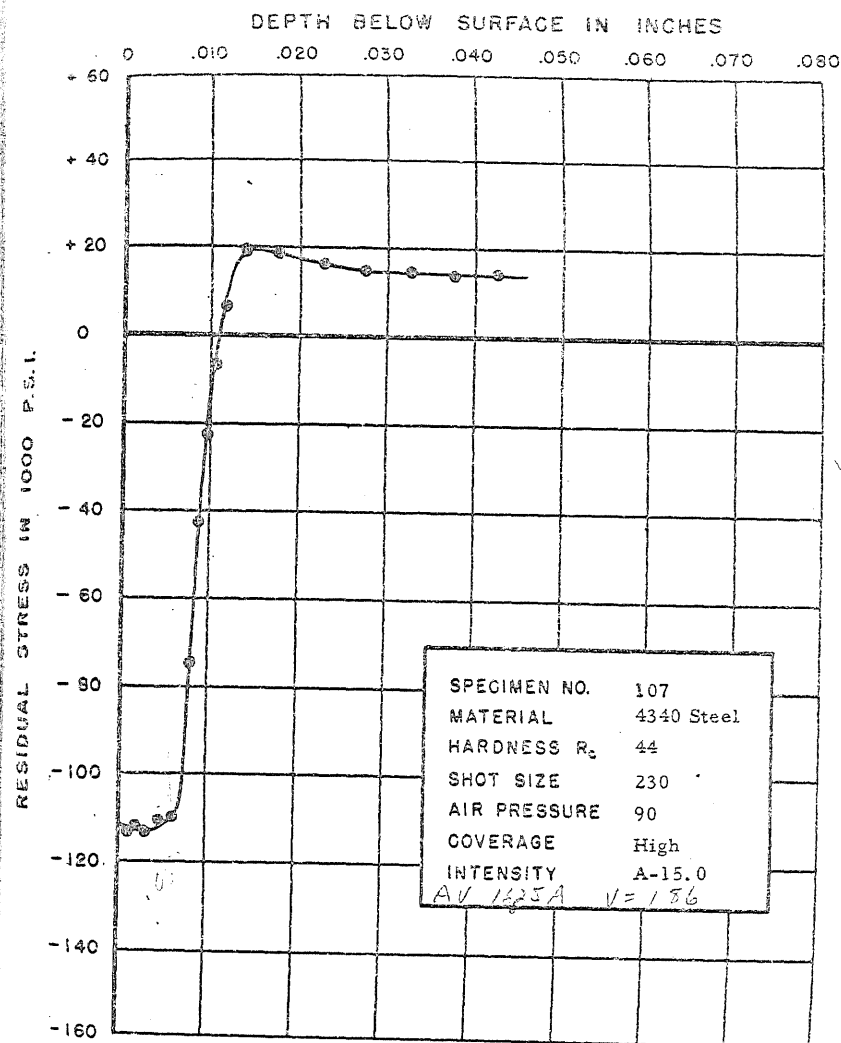
FIGURE 140. RESIDUAL STRESS DISTRIBUTION
