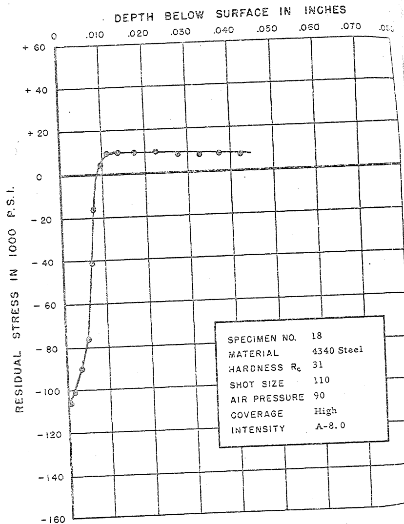
FIGURE 51. RESIDUAL STRESS DISTRIBUTION
