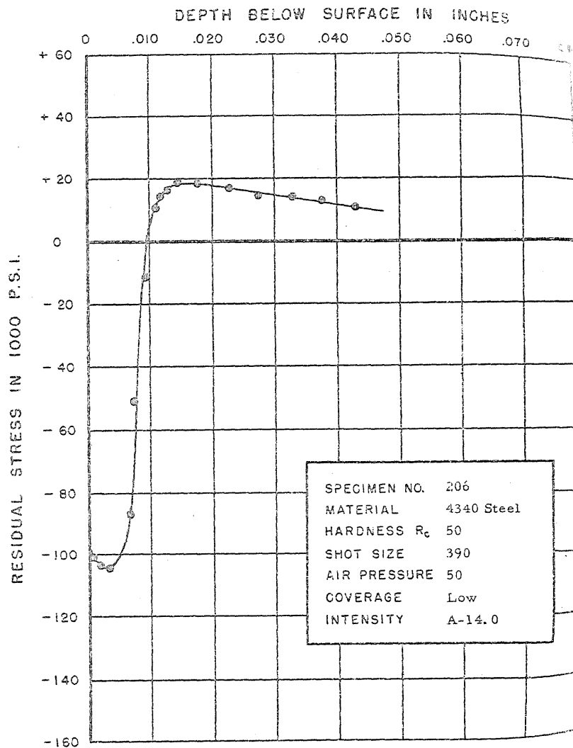
FIGURE 239. RESIDUAL STRESS DISTRIBUTION
