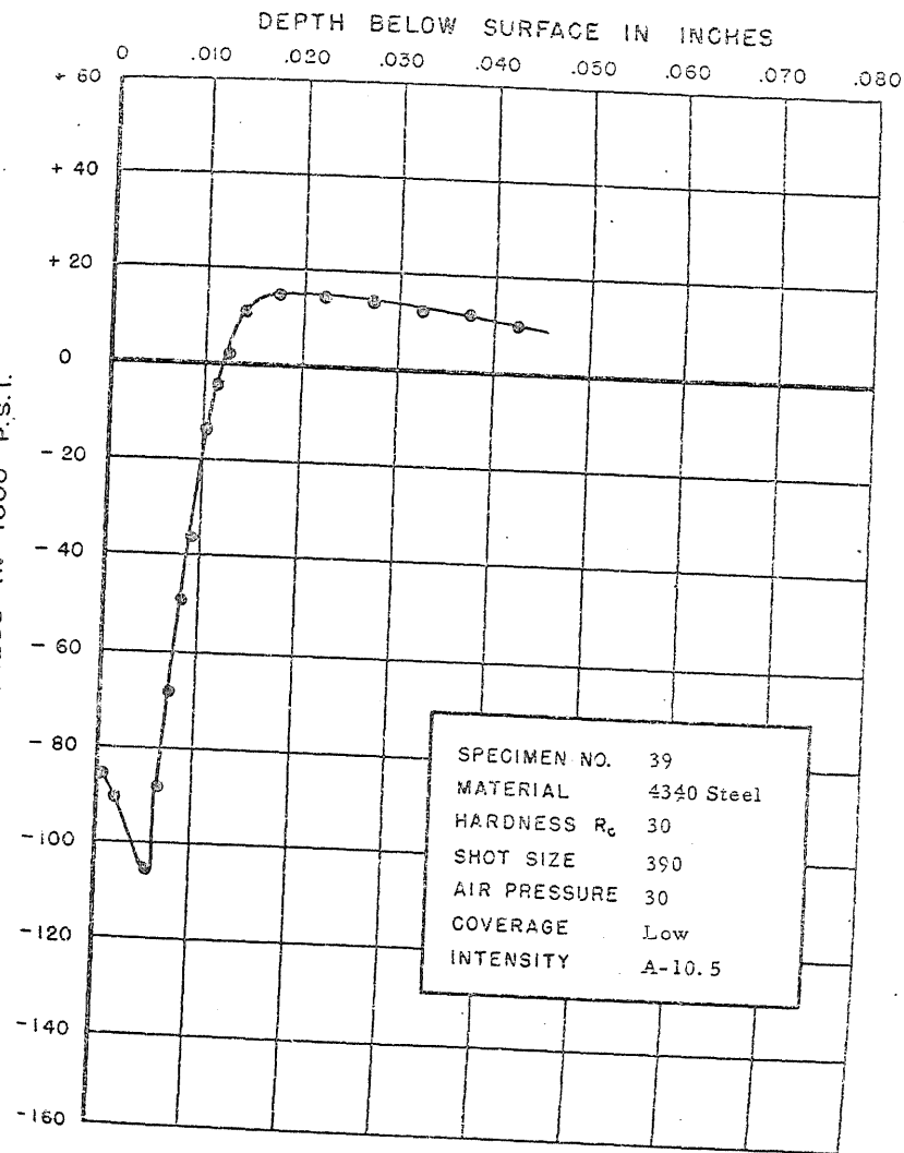
FIGURE 72. RESIDUAL STRESS DISTRIBUTION
