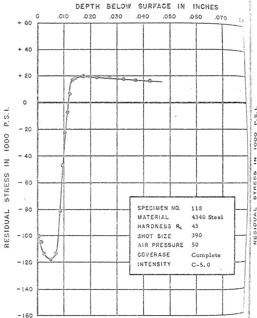
FIGURE 151. RESIDUAL STRESS DISTRIBUTION
