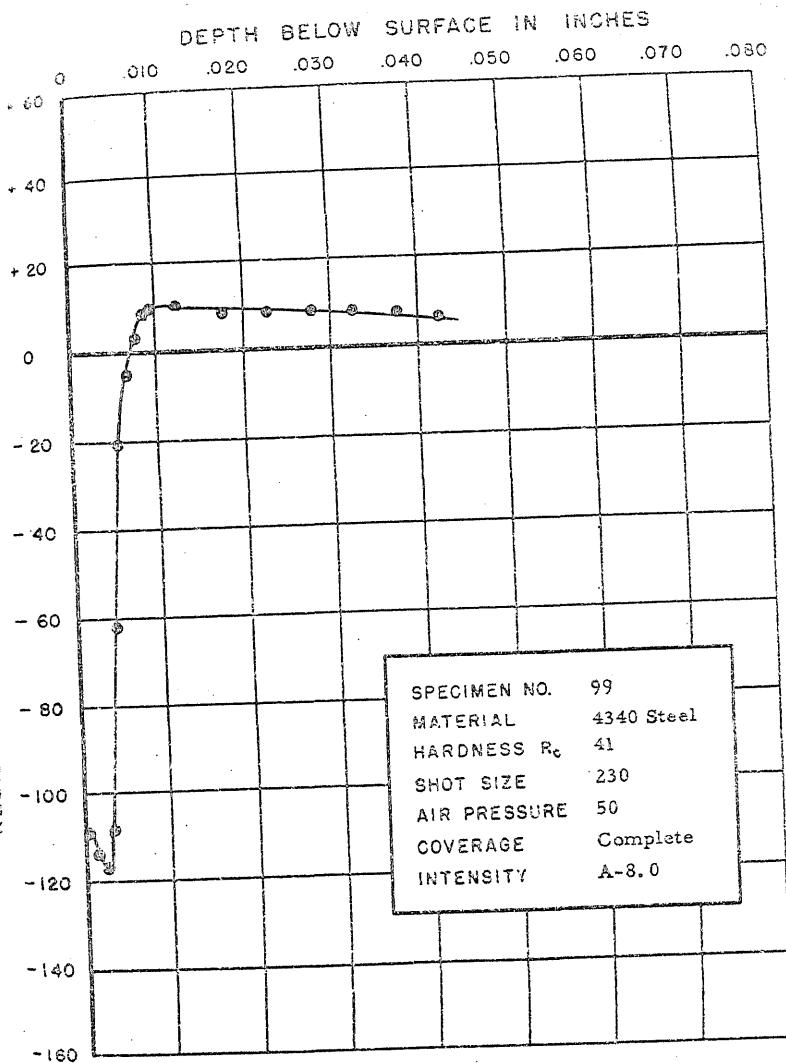
FIGURE 132. RESIDUAL STRESS DISTRIBUTION
