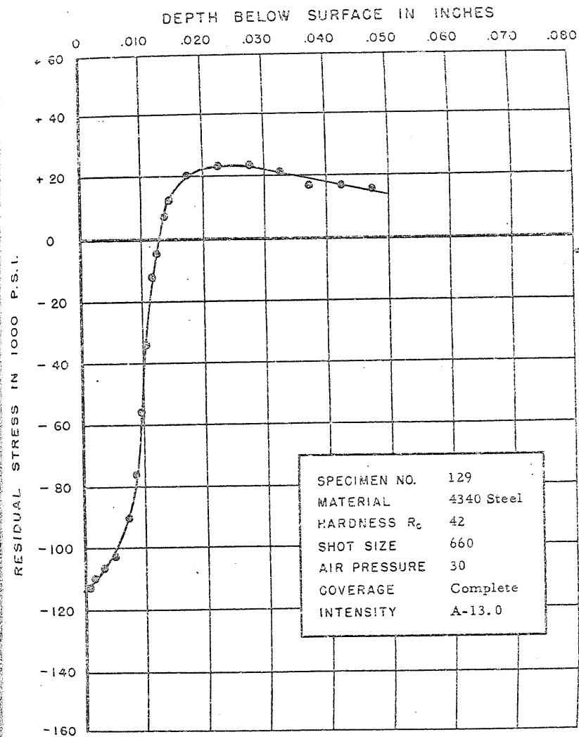
FIGURE 162. RESIDUAL STRESS DISTRIBUTION
