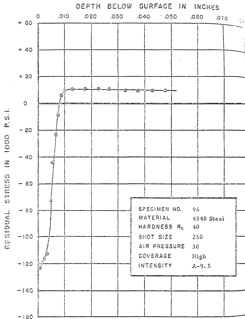
FIGURE 129. RESIDUAL STRESS DISTRIBUTION
