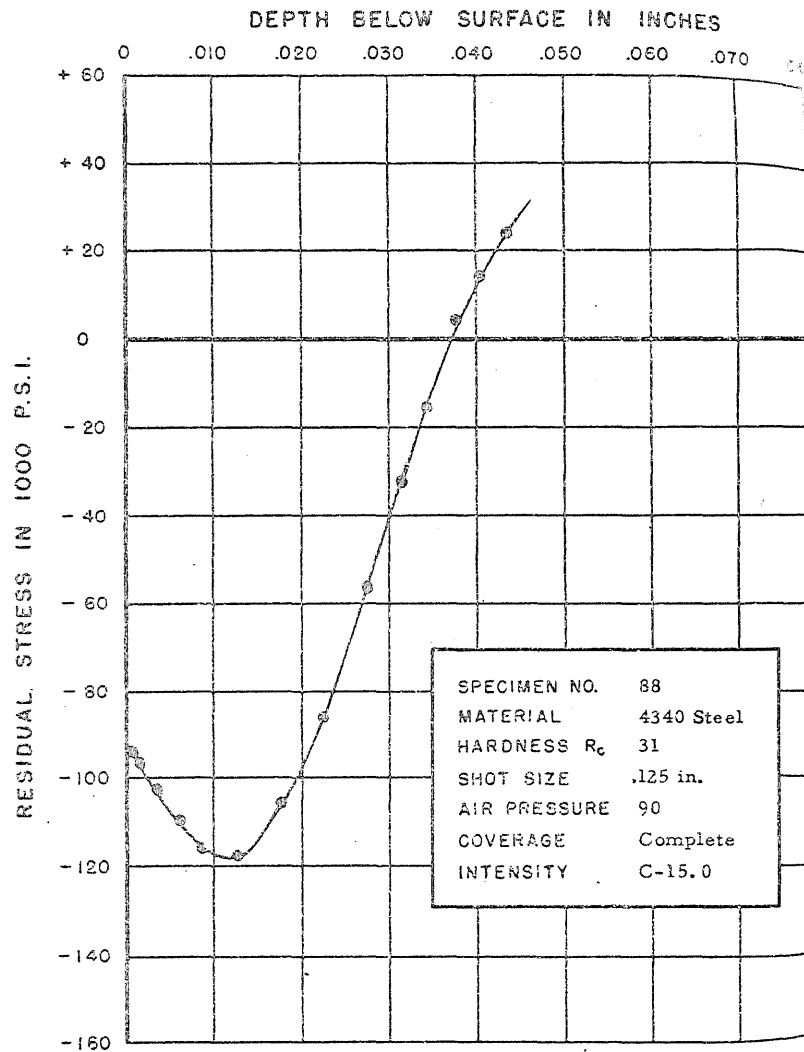
FIGURE 121. RESIDUAL STRESS DISTRIBUTION
