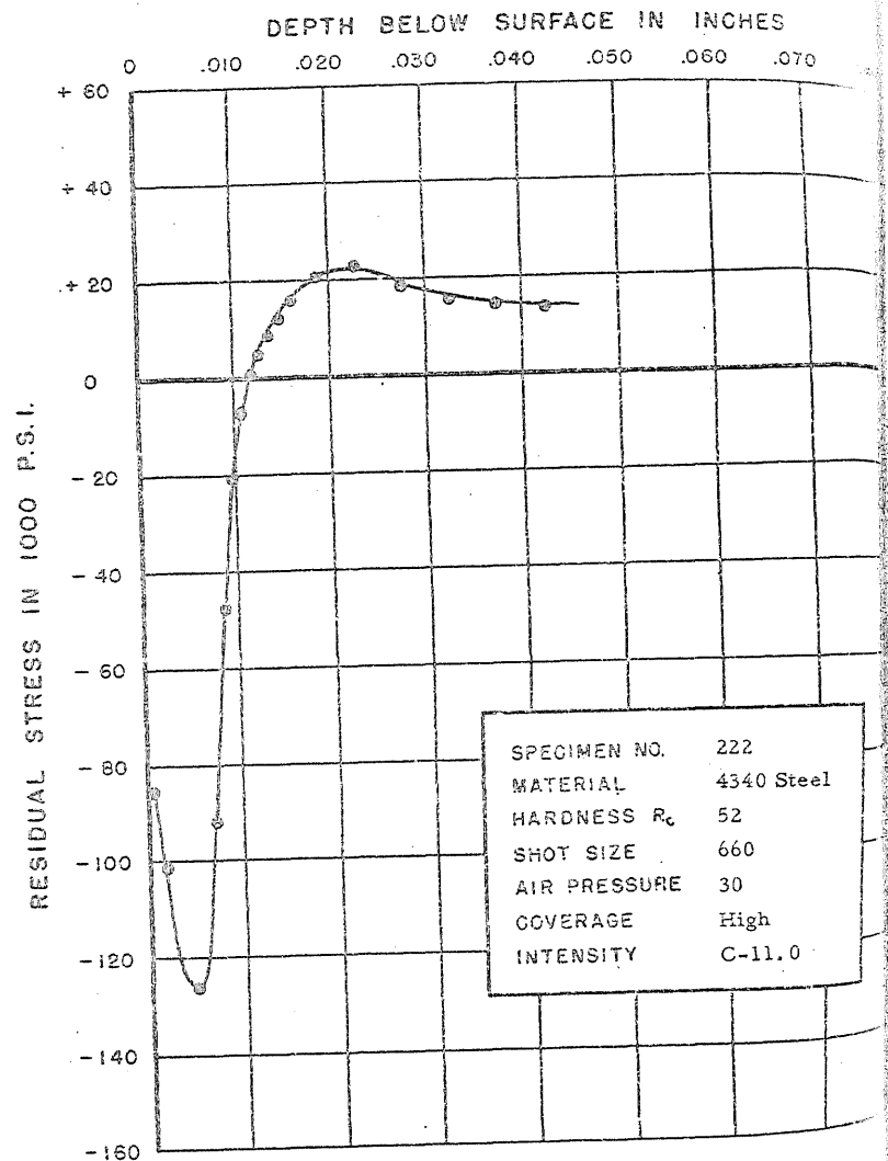
FIGURE 255. RESIDUAL STRESS DISTRIBUTION
