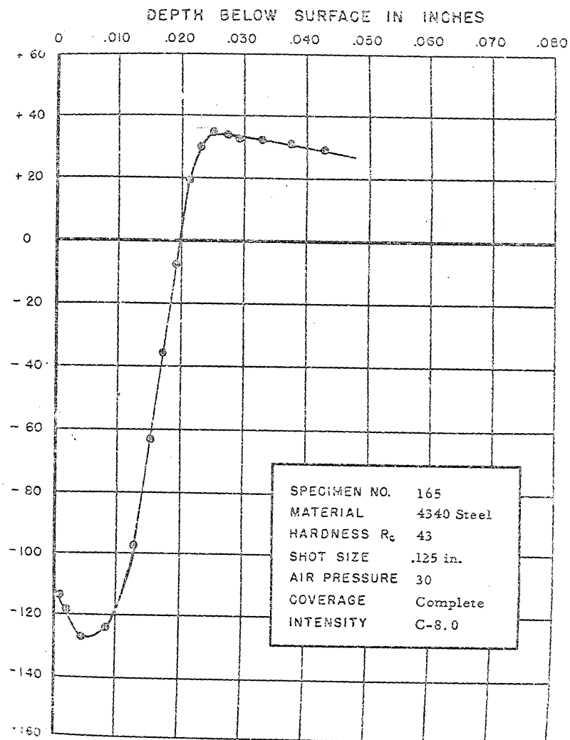
FIGURE 198. RESIDUAL STRESS DISTRIBUTION
