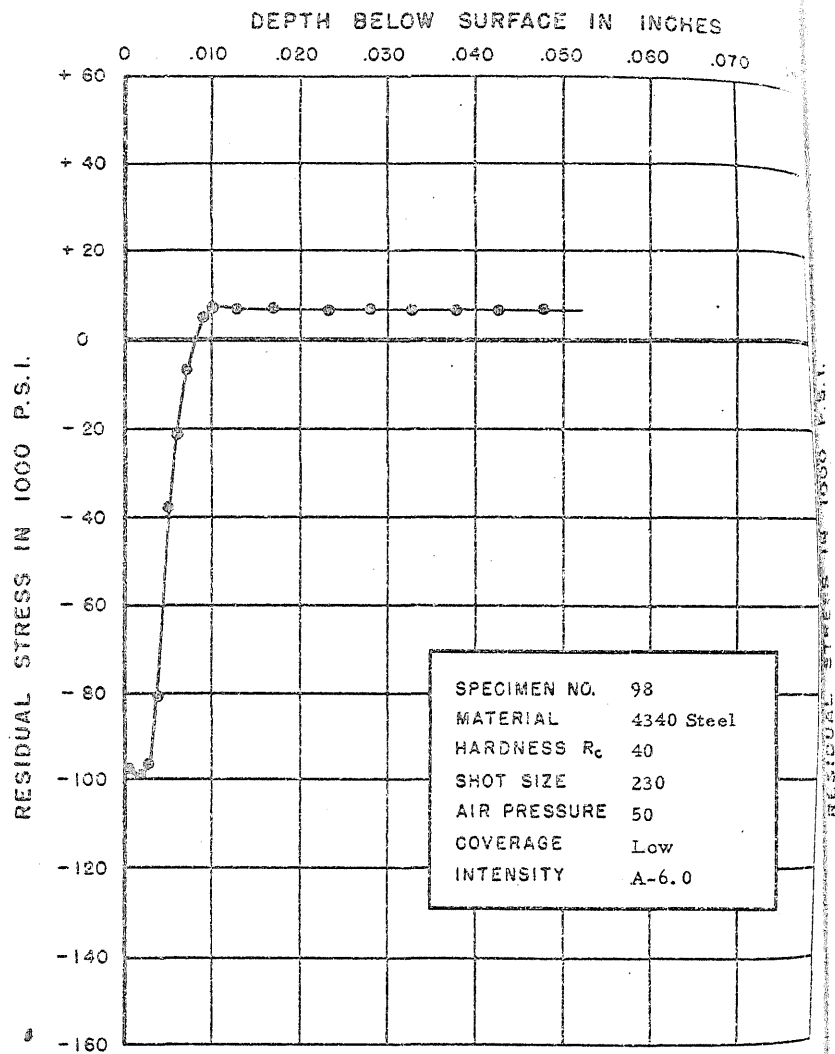
FIGURE 131. RESIDUAL STRESS DISTRIBUTION
