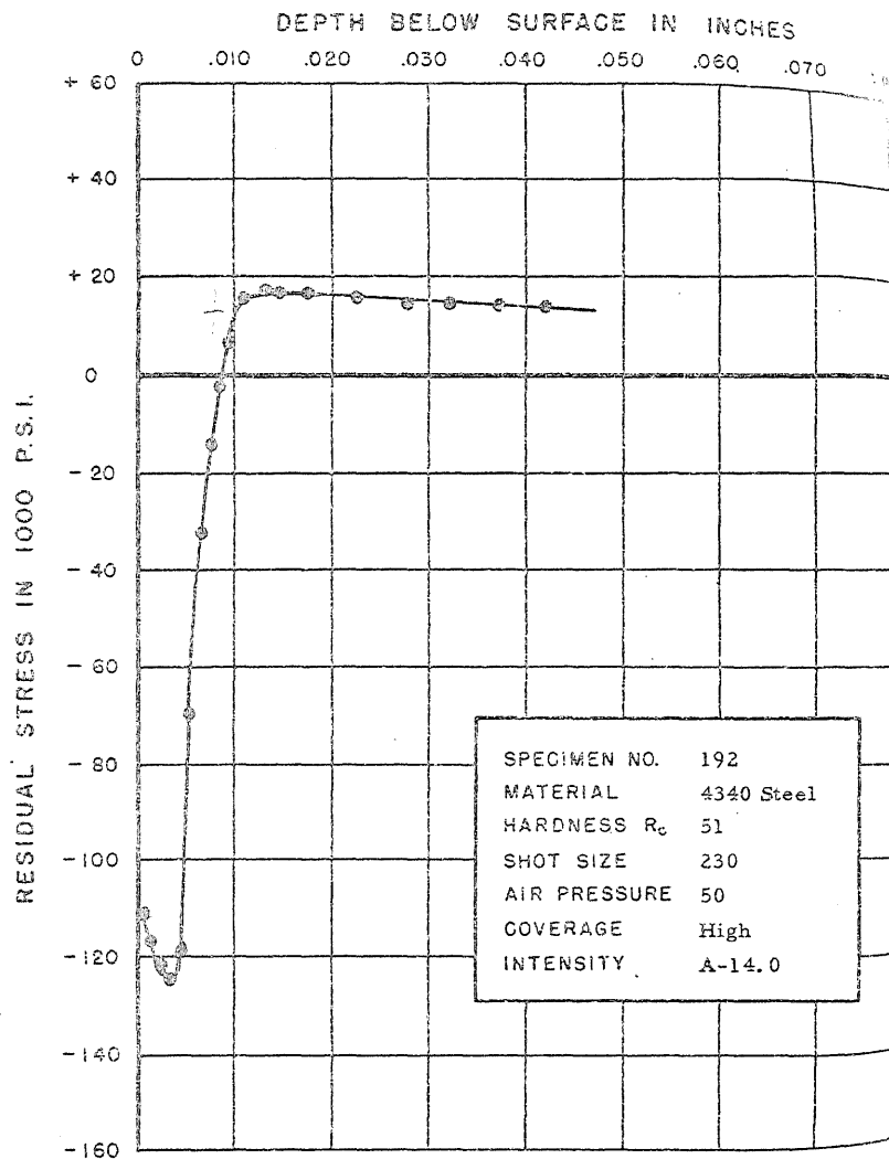
FIGURE 225. RESIDUAL STRESS DISTRIBUTION
