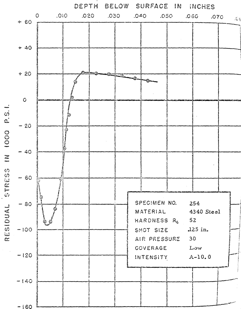
FIGURE 287. RESIDUAL STRESS DISTRIBUTION*
