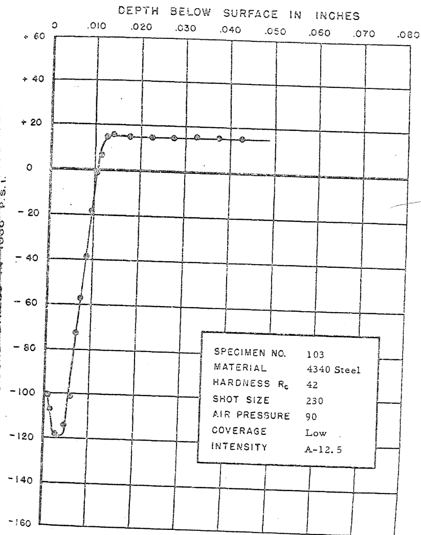
FIGURE 136. RESIDUAL STRESS DISTRIBUTION
