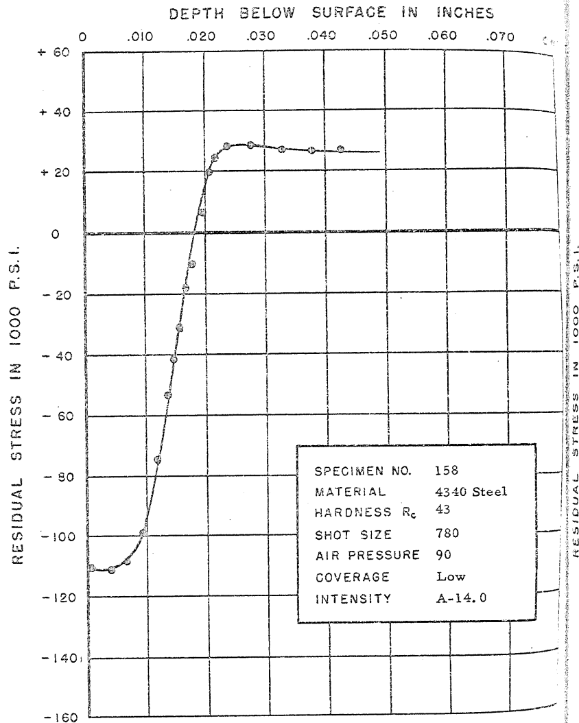
FIGURE 191. RESIDUAL STRESS DISTRIBUTION
