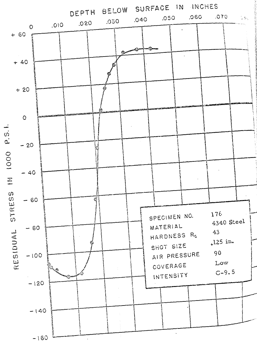
FIGURE 209. RESIDUAL STRESS DISTRIBUTION
