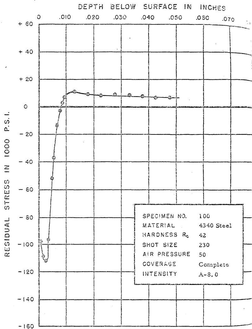
FIGURE 133. RESIDUAL STRESS DISTRIBUTION
