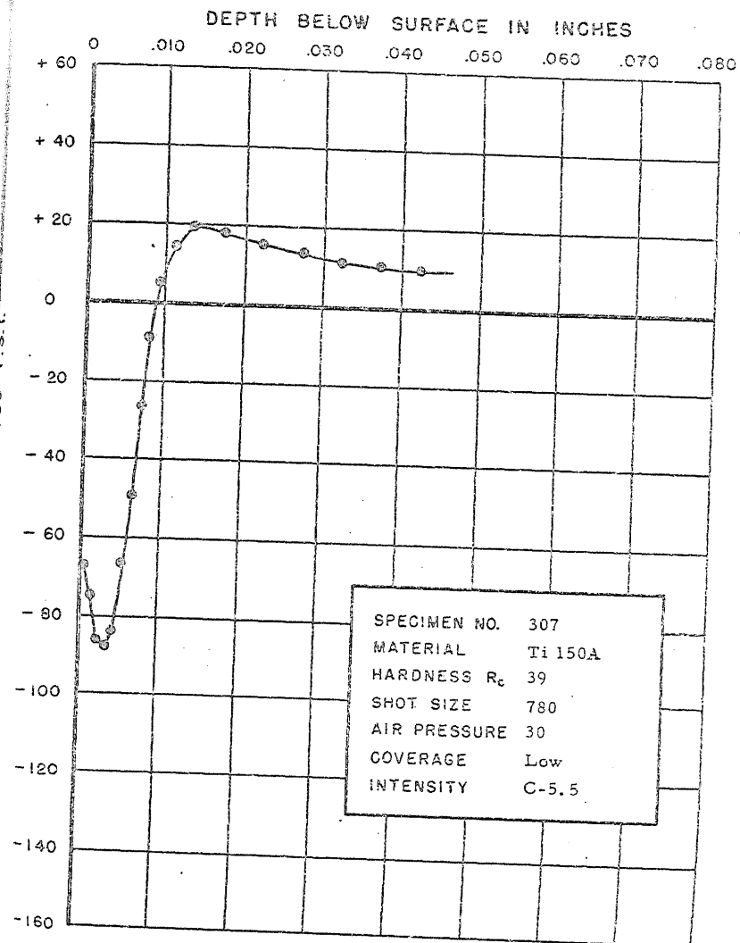
FIGURE 340. RESIDUAL STRESS DISTRIBUTION
