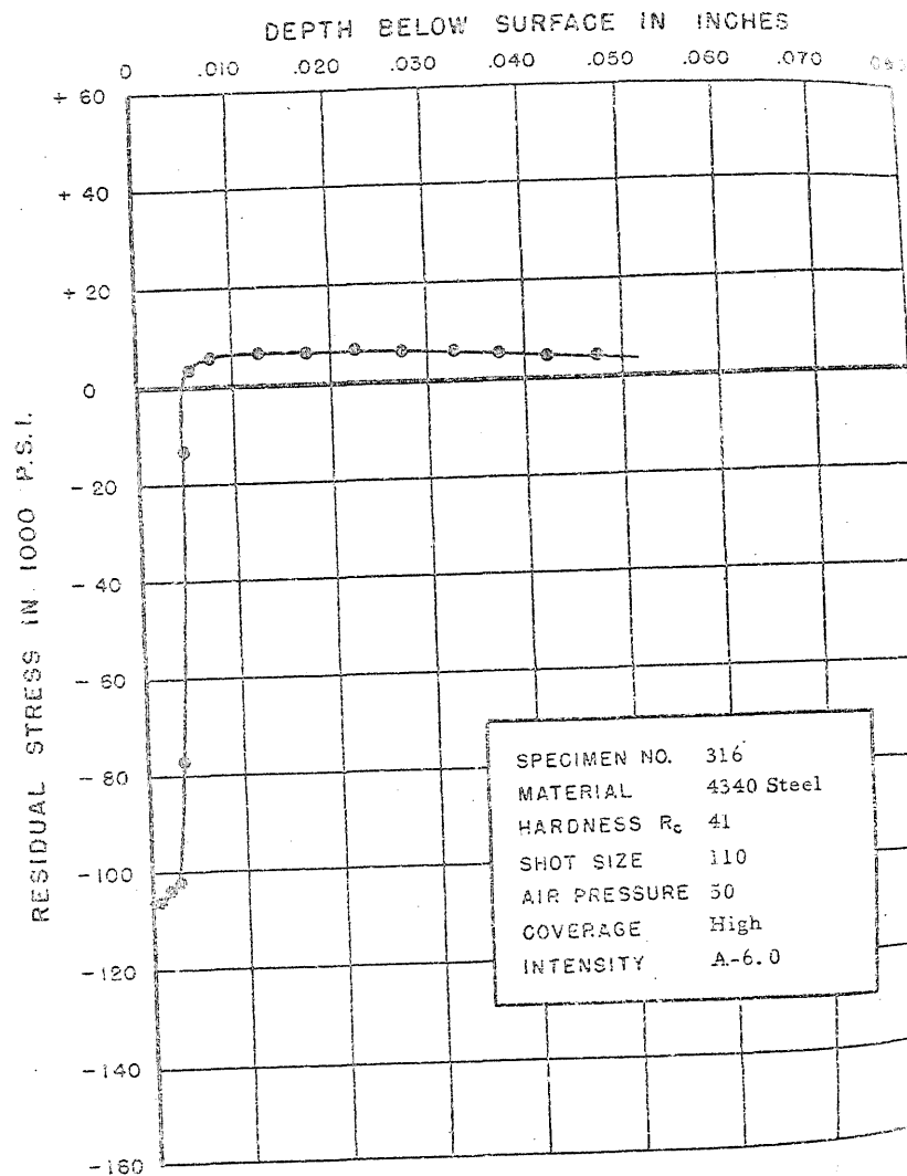
FIGURE 349. RESIDUAL STRESS DISTRIBUTION
