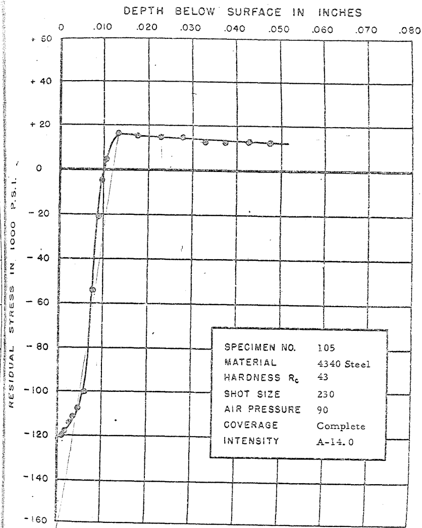
FIGURE 138. RESIDUAL STRESS DISTRIBUTION
