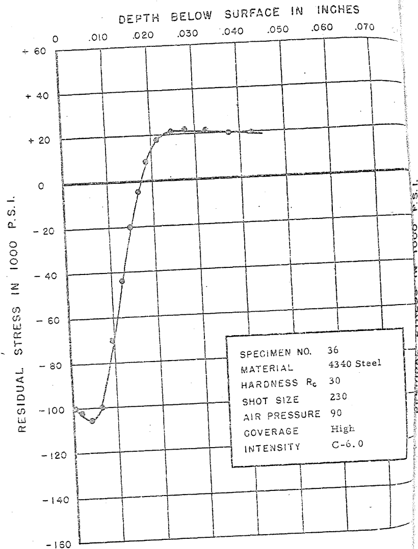
FIGURE 69. RESIDUAL STRESS DISTRIBUTION
