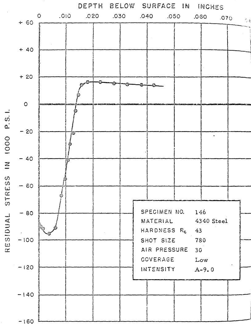
FIGURE 179. RESIDUAL STRESS DISTRIBUTION
