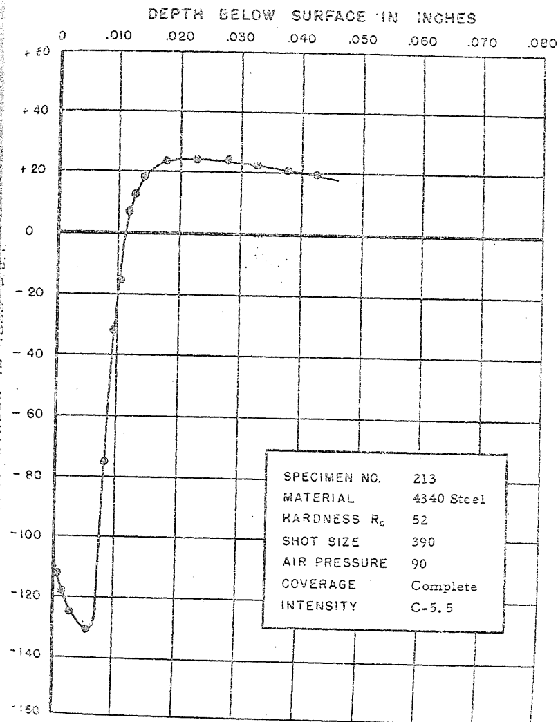
FIGURE 246. RESIDUAL STRESS DISTRIBUTION
