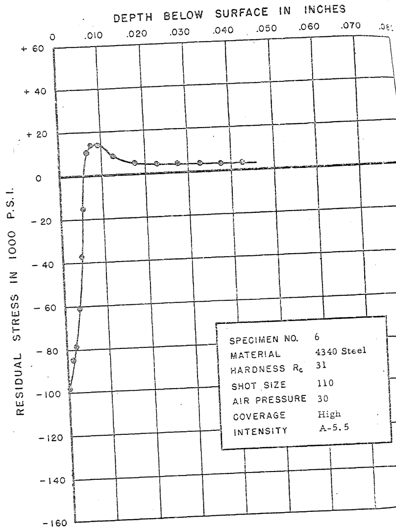
FIGURE 39. RESIDUAL STRESS DISTRIBUTION
