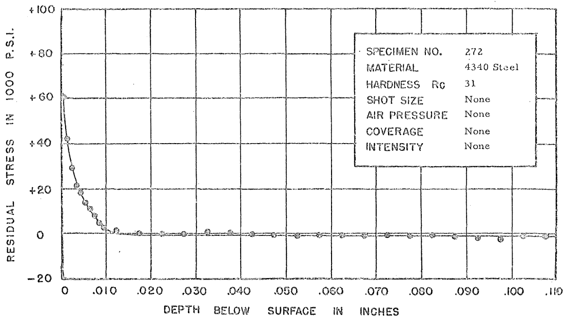
FIGURE 305. RESIDUAL STRESS DISTRIBUTION
