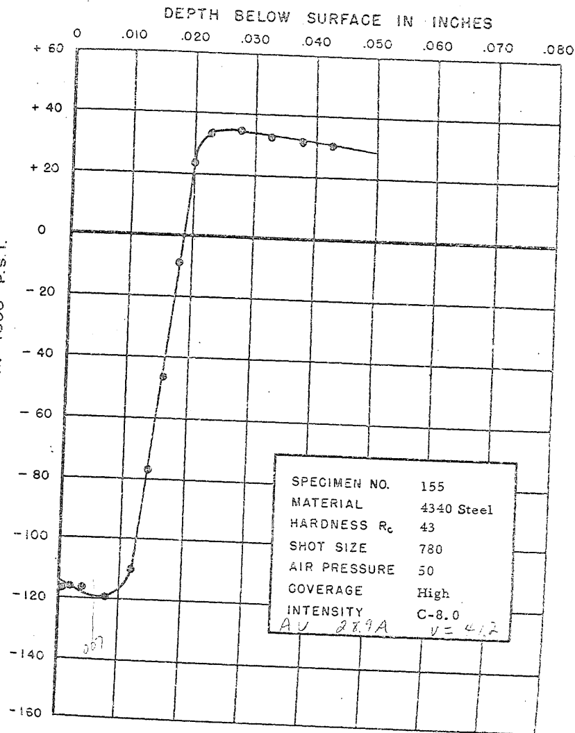
FIGURE 188. RESIDUAL STRESS DISTRIBUTION
