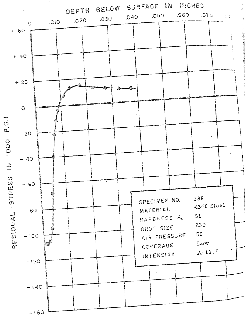
FIGURE 221. RESIDUAL STRESS DISTRIBUTION
