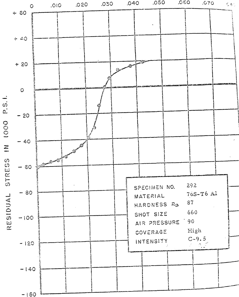
FIGURE 325. RESIDUAL STRESS DISTRIBUTION
