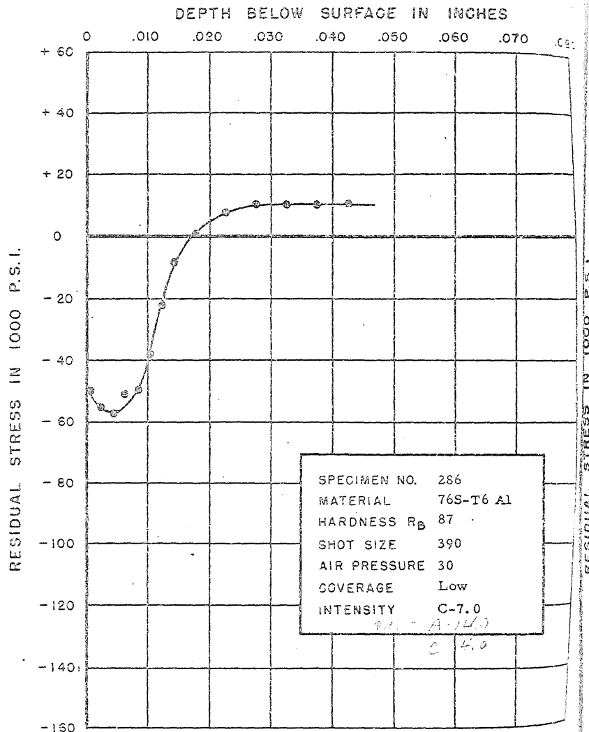
FIGURE 319. RESIDUAL STRESS DISTRIBUTION
