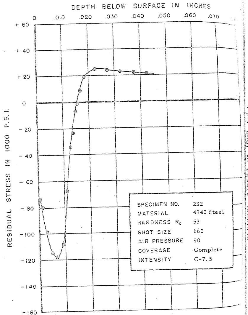
FIGURE 265. RESIDUAL STRESS DISTRIBUTION
