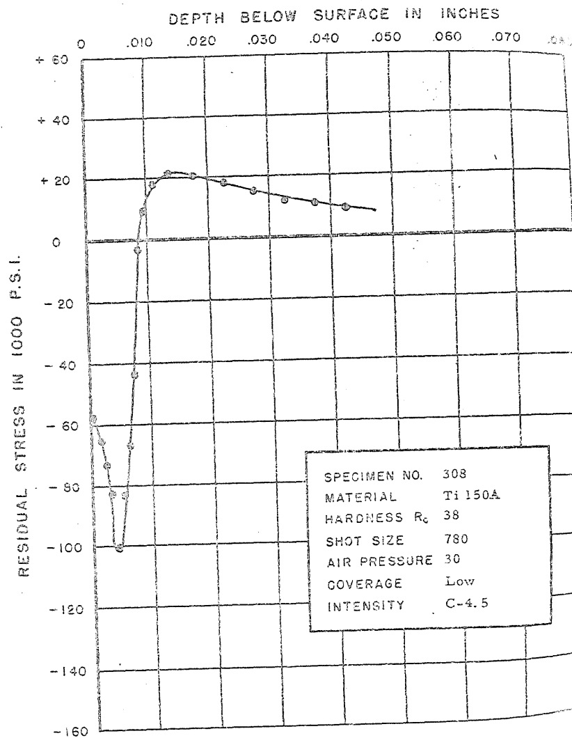
FIGURE 341. RESIDUAL STRESS DISTRIBUTION
