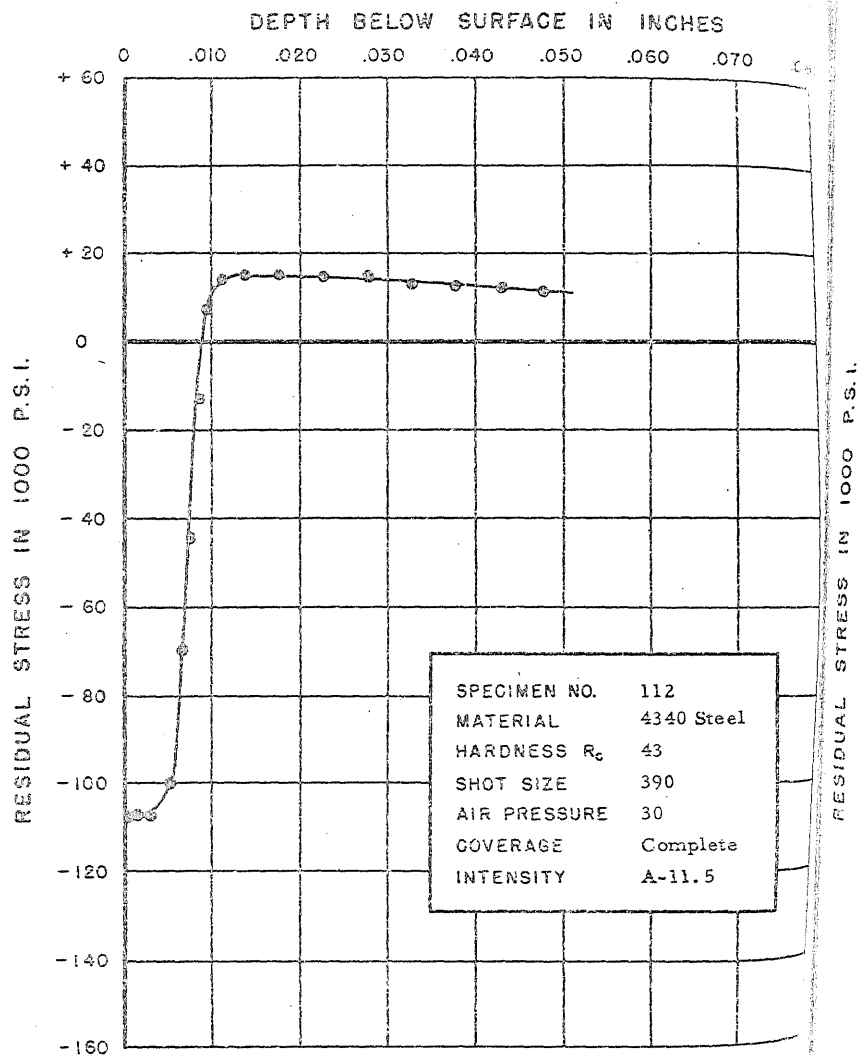
FIGURE 145. RESIDUAL STRESS DISTRIBUTION
