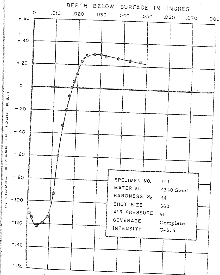
FIGURE 174. RESIDUAL STRESS DISTRIBUTION
