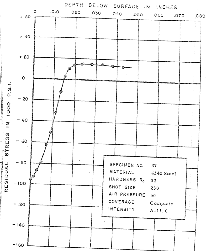
FIGURE 60. RESIDUAL STRESS DISTRIBUTION
