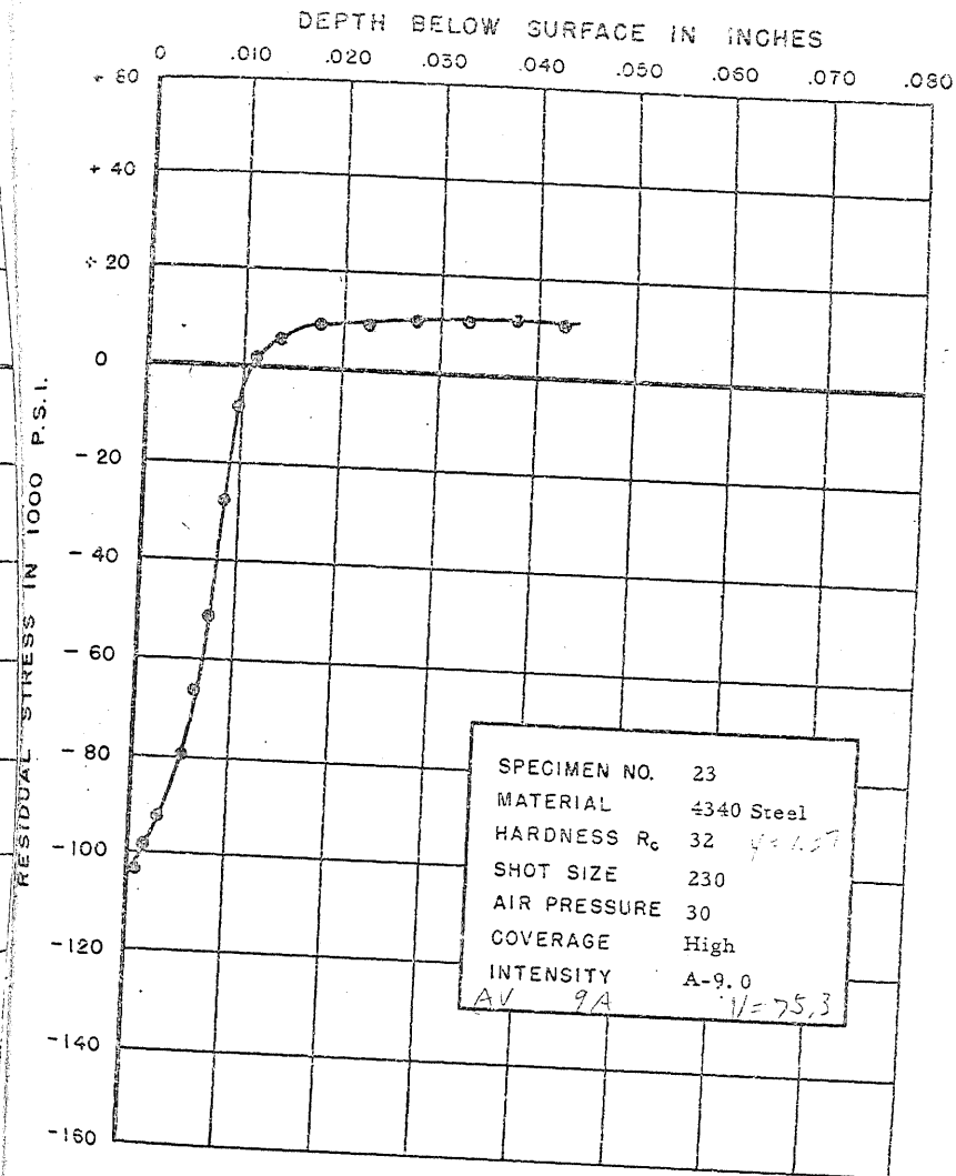
FIGURE 56. RESIDUAL STRESS DISTRIBUTION
