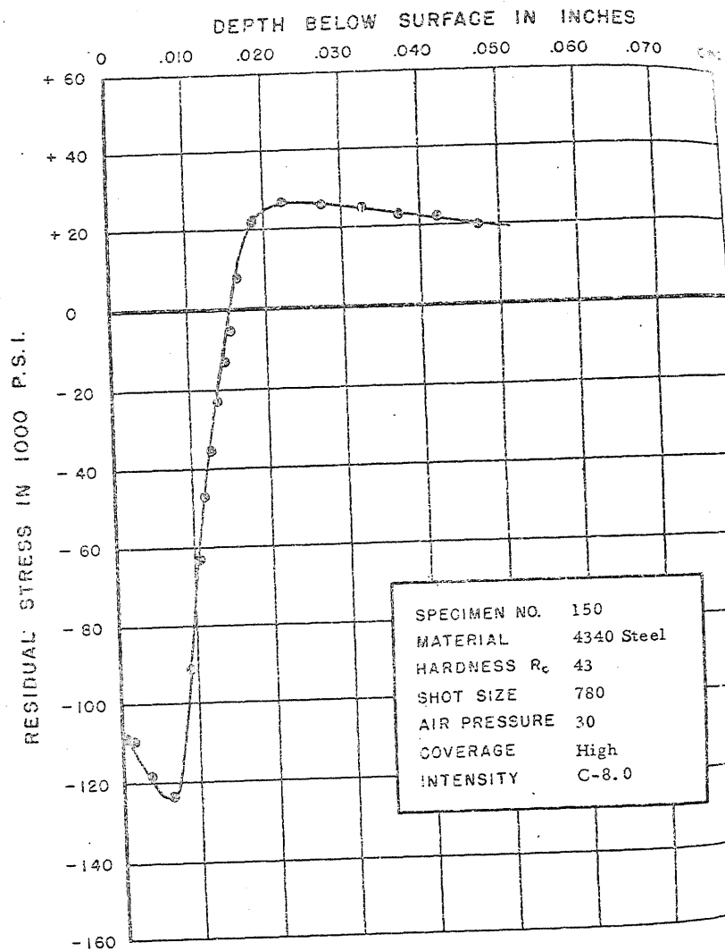
FIGURE 183. RESIDUAL STRESS DISTRIBUTION
