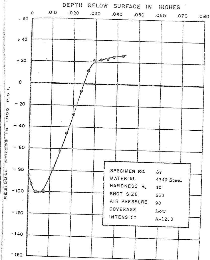
FIGURE 100. RESIDUAL STRESS DISTRIBUTION
