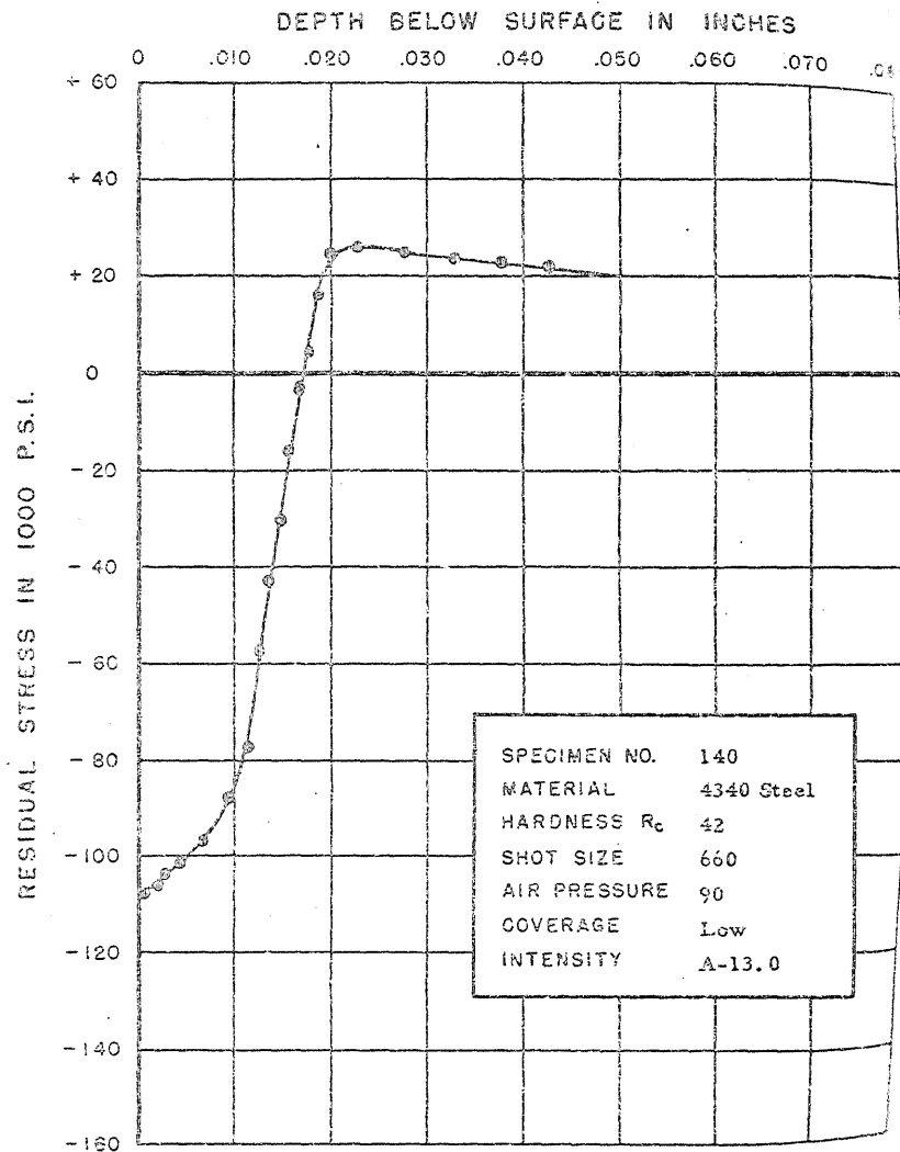
FIGURE 173. RESIDUAL STRESS DISTRIBUTION
