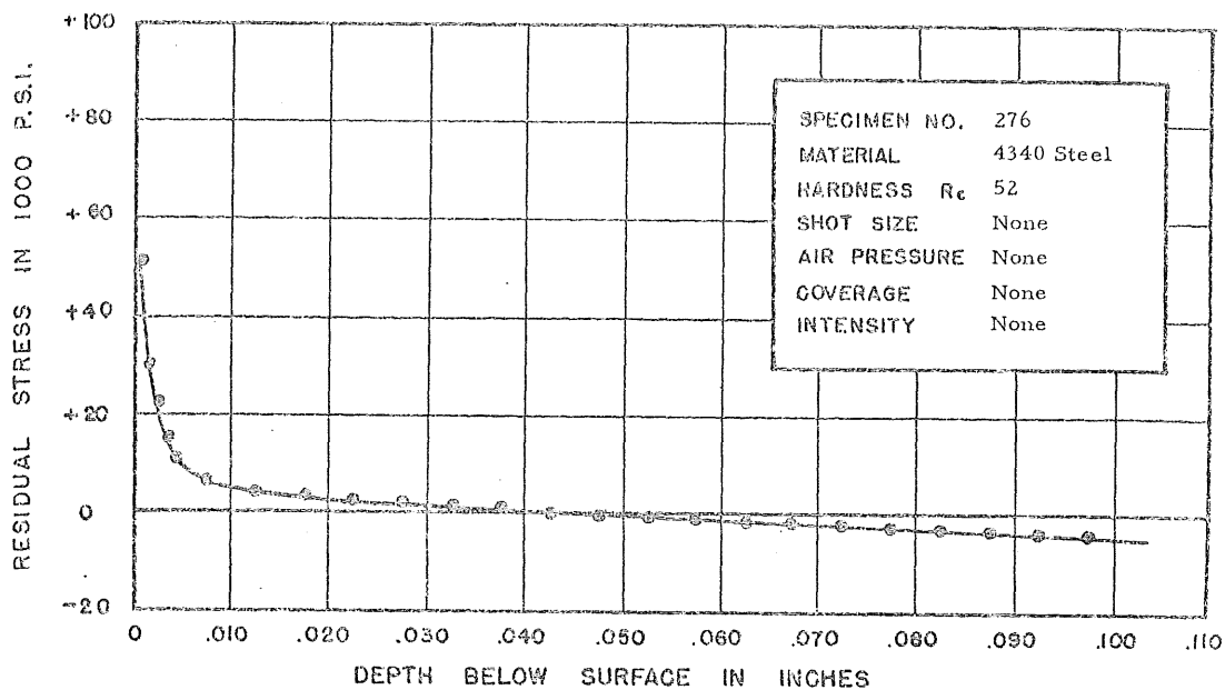
FIGURE 309. RESIDUAL STRESS DISTRIBUTION
