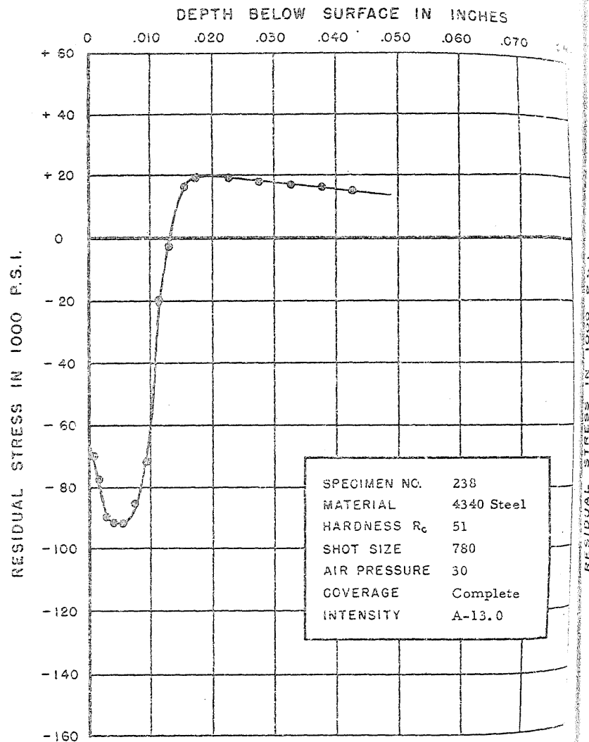
FIGURE 271. RESIDUAL STRESS DISTRIBUTION
