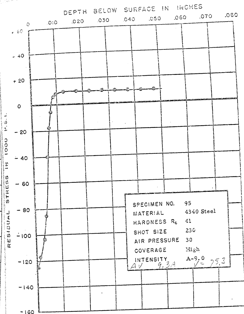
FIGURE 128. RESIDUAL STRESS DISTRIBUTION
