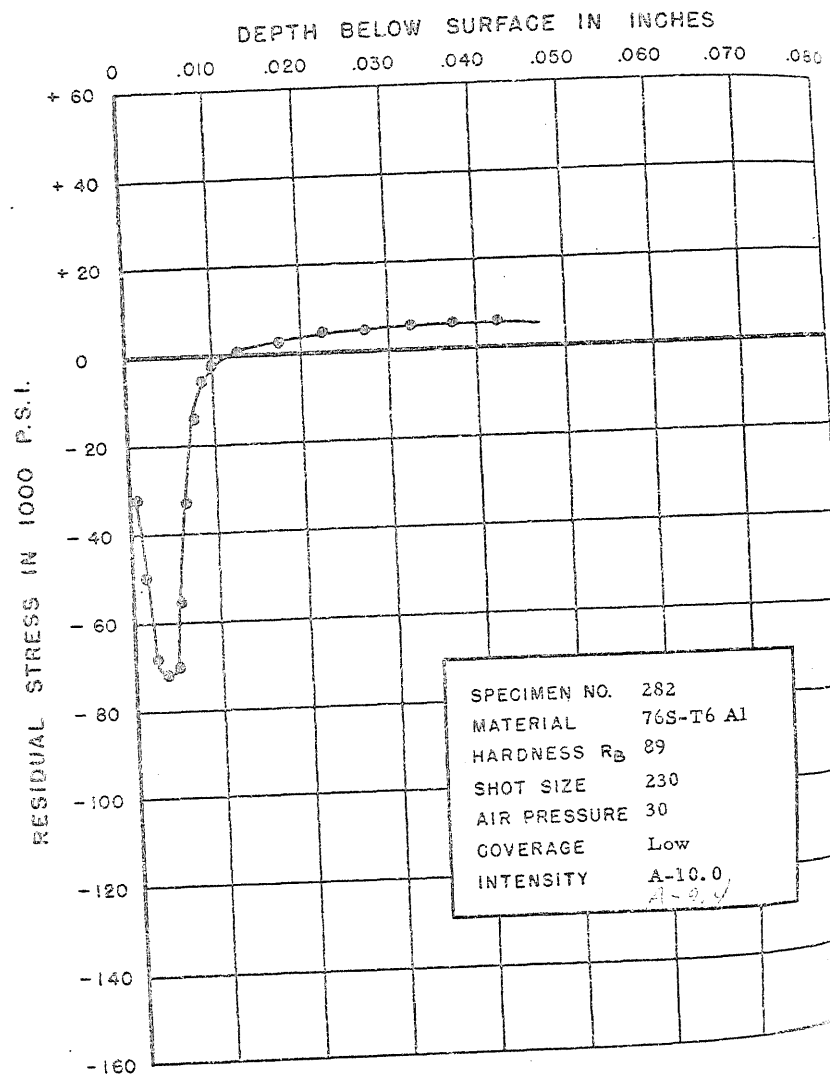
FIGURE 315. RESIDUAL STRESS DISTRIBUTION
