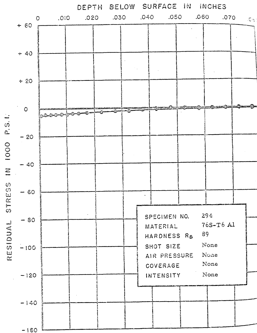
FIGURE 327. RESIDUAL STRESS DISTRIBUTION
