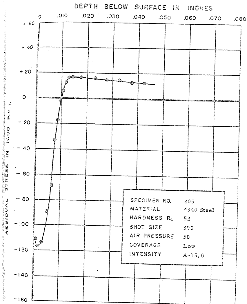
FIGURE 238. RESIDUAL STRESS DISTRIBUTION
