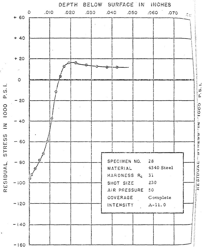
FIGURE 61. RESIDUAL STRESS DISTRIBUTION
