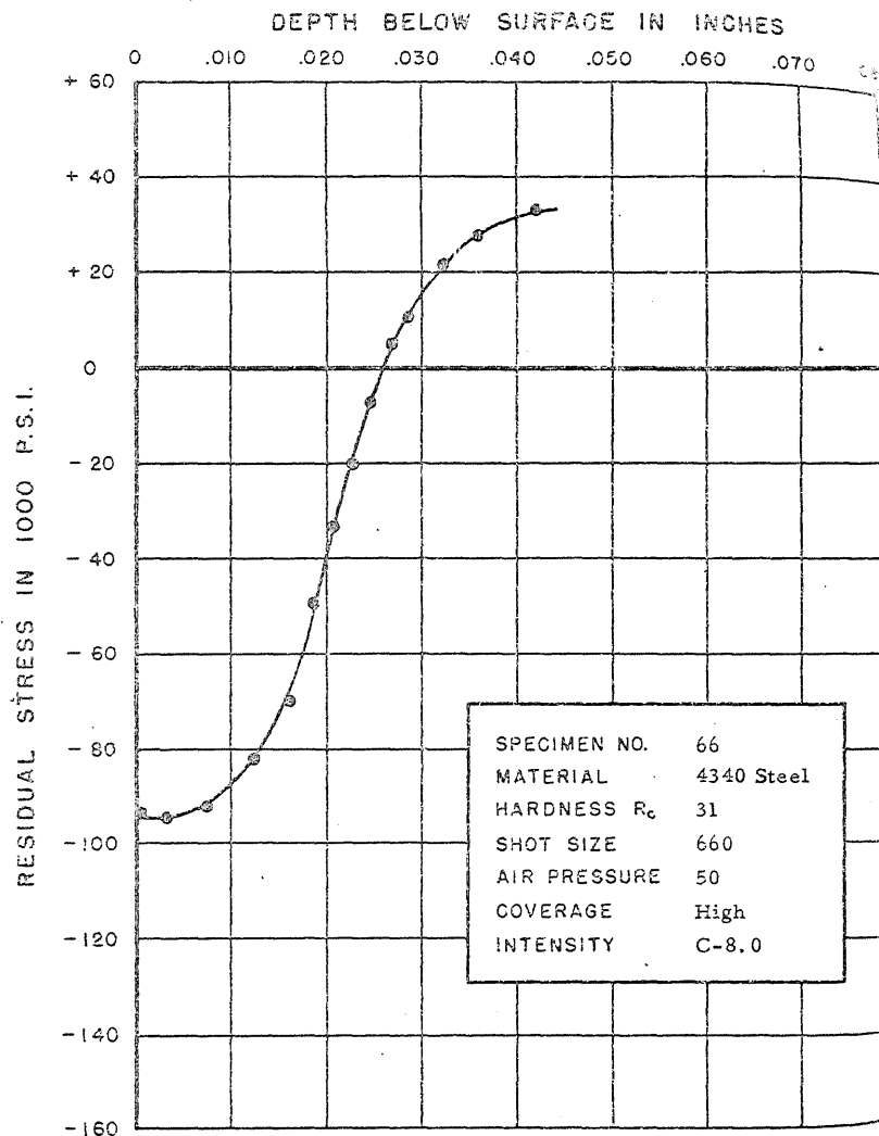
FIGURE 99. RESIDUAL STRESS DISTRIBUTION
