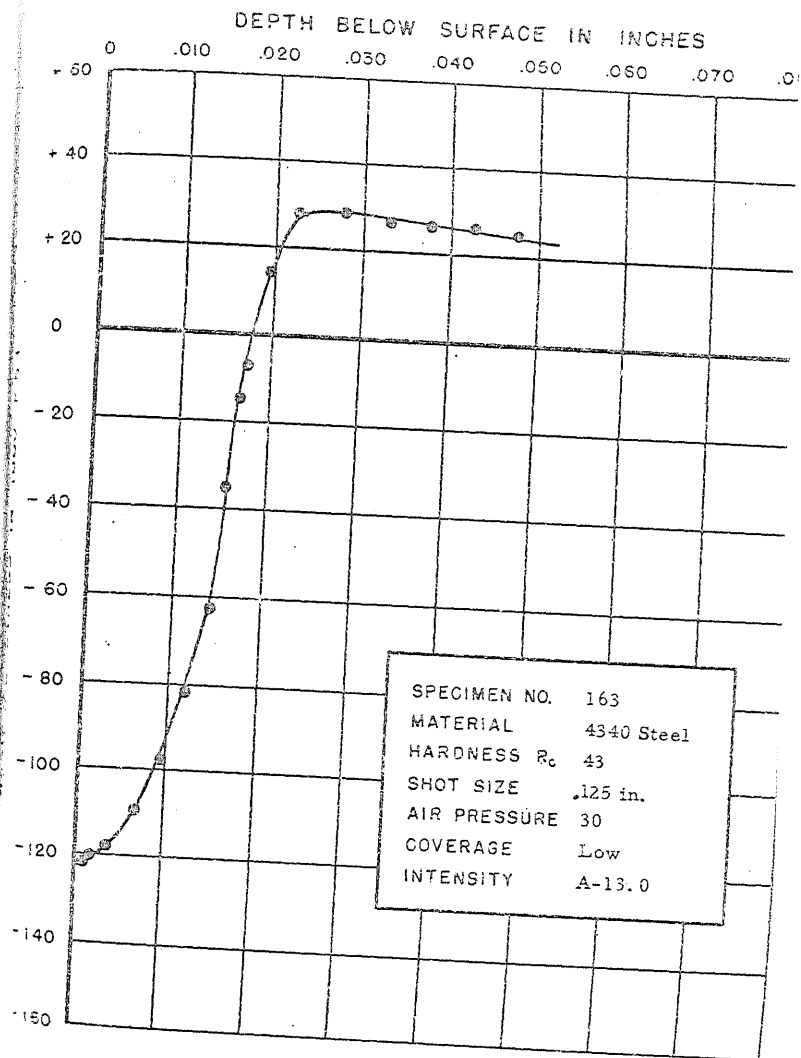
FIGURE 196. RESIDUAL STRESS DISTRIBUTION
