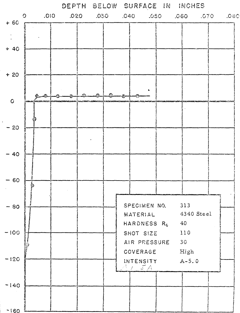
FIGURE 345. RESIDUAL STRESS DISTRIBUTION
