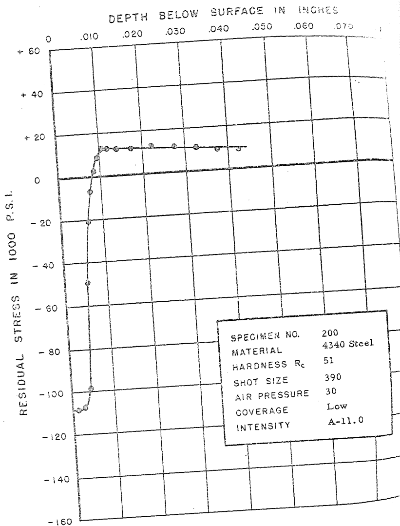
FIGURE 233. RESIDUAL STRESS DISTRIBUTION
