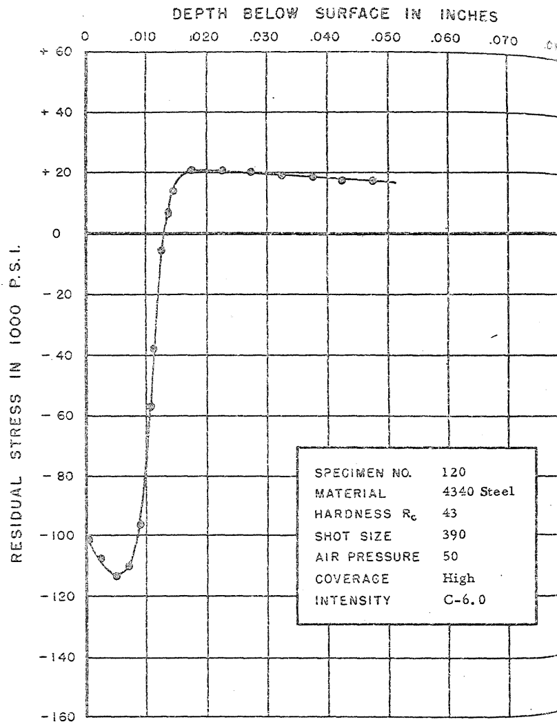
FIGURE 153. RESIDUAL STRESS DISTRIBUTION
