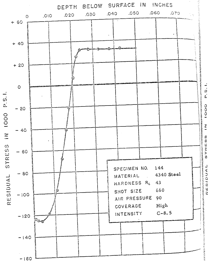
FIGURE 177. RESIDUAL STRESS DISTRIBUTION
