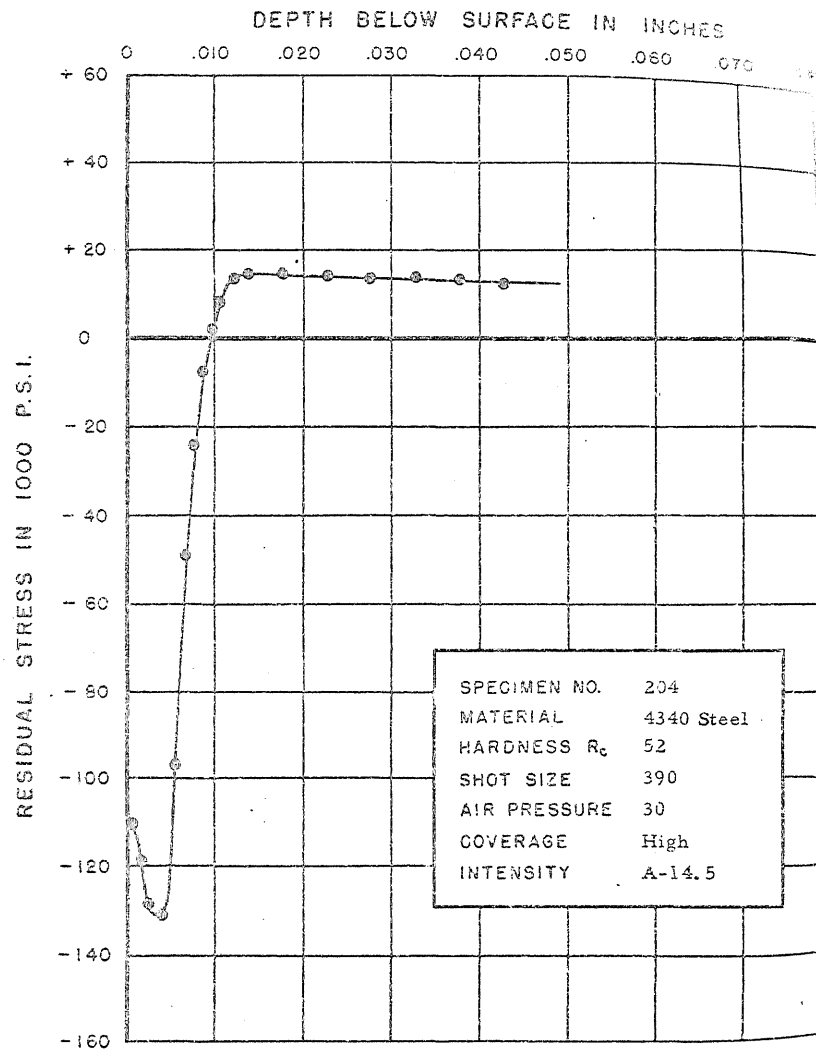
FIGURE 237. RESIDUAL STRESS DISTRIBUTION
