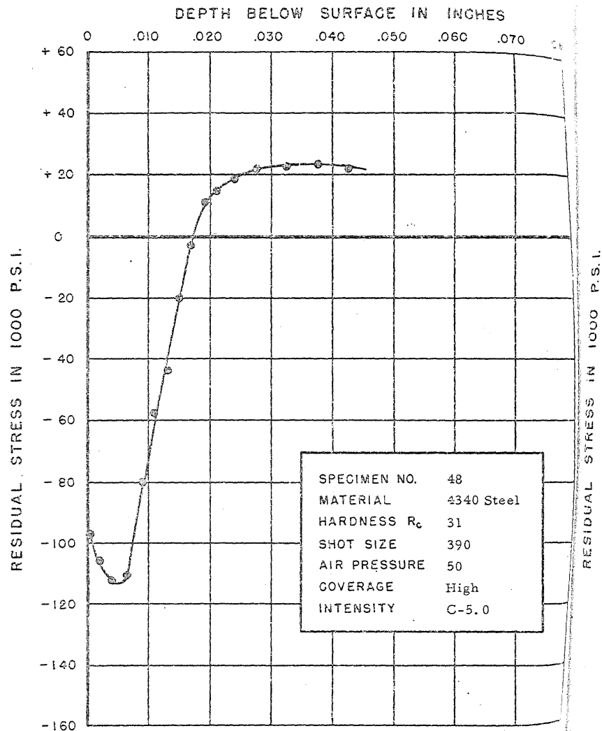
FIGURE 81. RESIDUAL STRESS DISTRIBUTION
