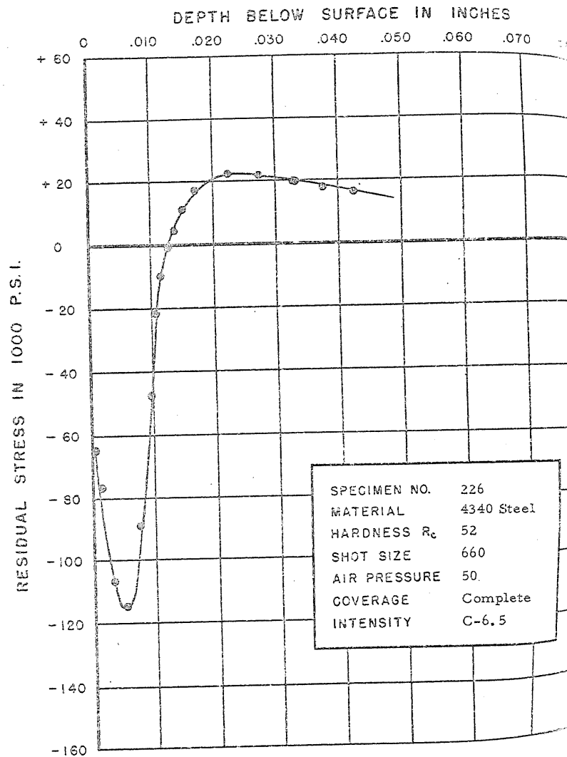
FIGURE 259. RESIDUAL STRESS DISTRIBUTION
