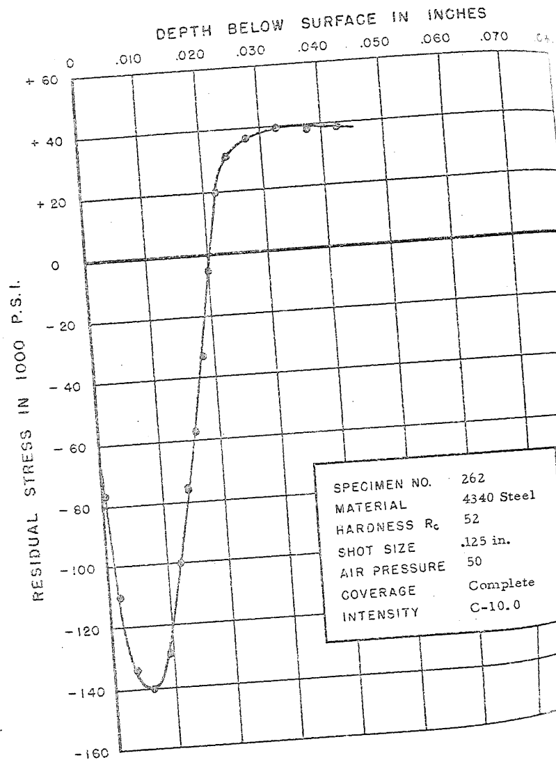
FIGURE 295. RESIDUAL STRESS DISTRIBUTION
