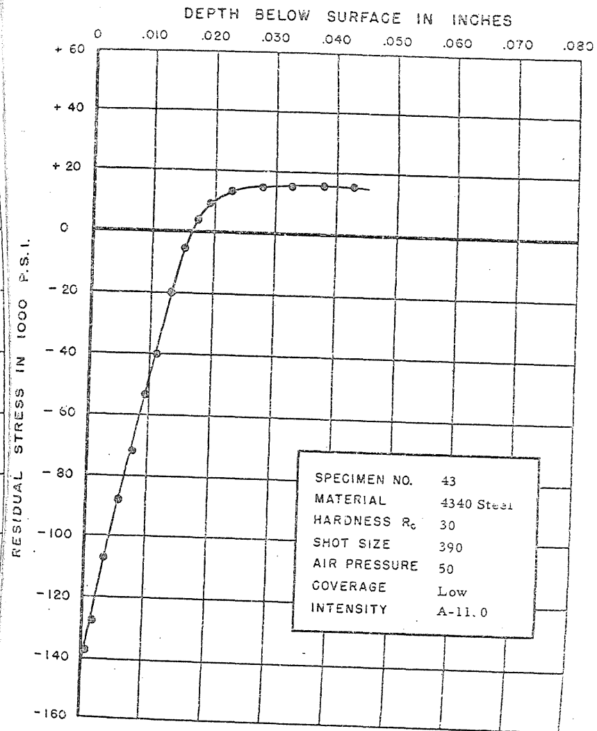
FIGURE 76. RESIDUAL STRESS DISTRIBUTION
