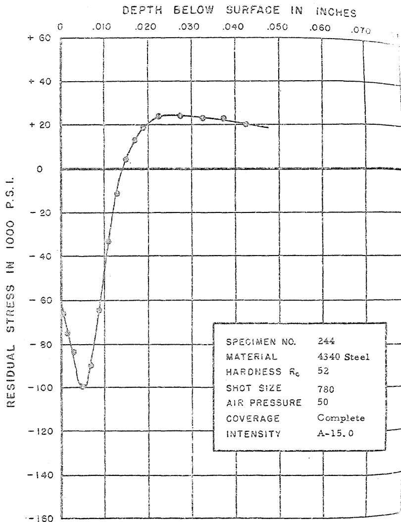
FIGURE 277. RESIDUAL STRESS DISTRIBUTION
