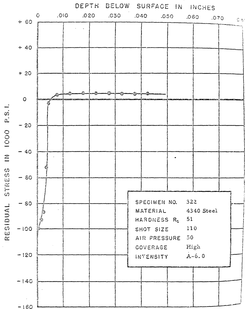
FIGURE 355. RESIDUAL STRESS DISTRIBUTION
