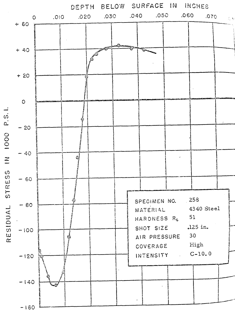
FIGURE 291. RESIDUAL STRESS DISTRIBUTION
