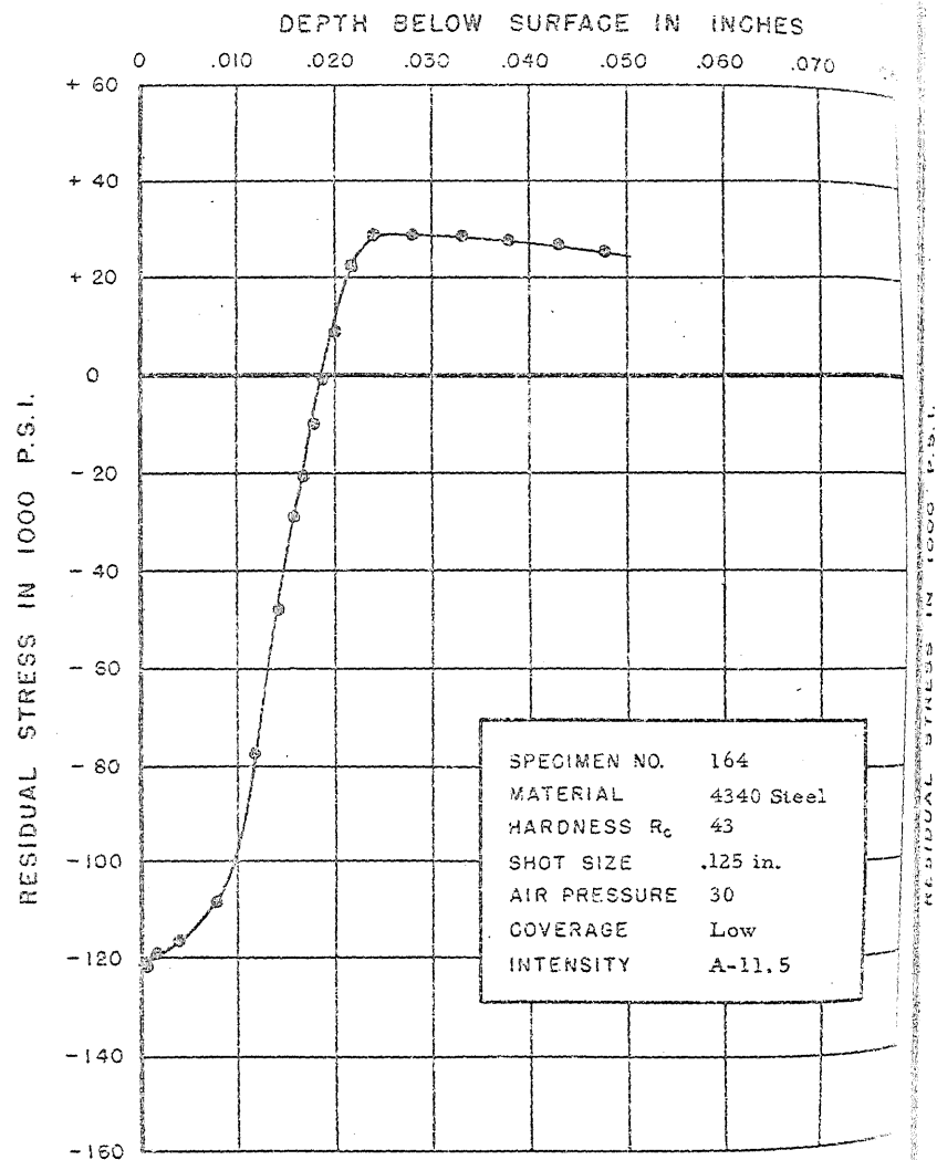
FIGURE 197. RESIDUAL STRESS DISTRIBUTION
