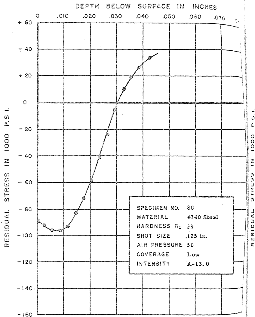
FIGURE 113. RESIDUAL STRESS DISTRIBUTION
