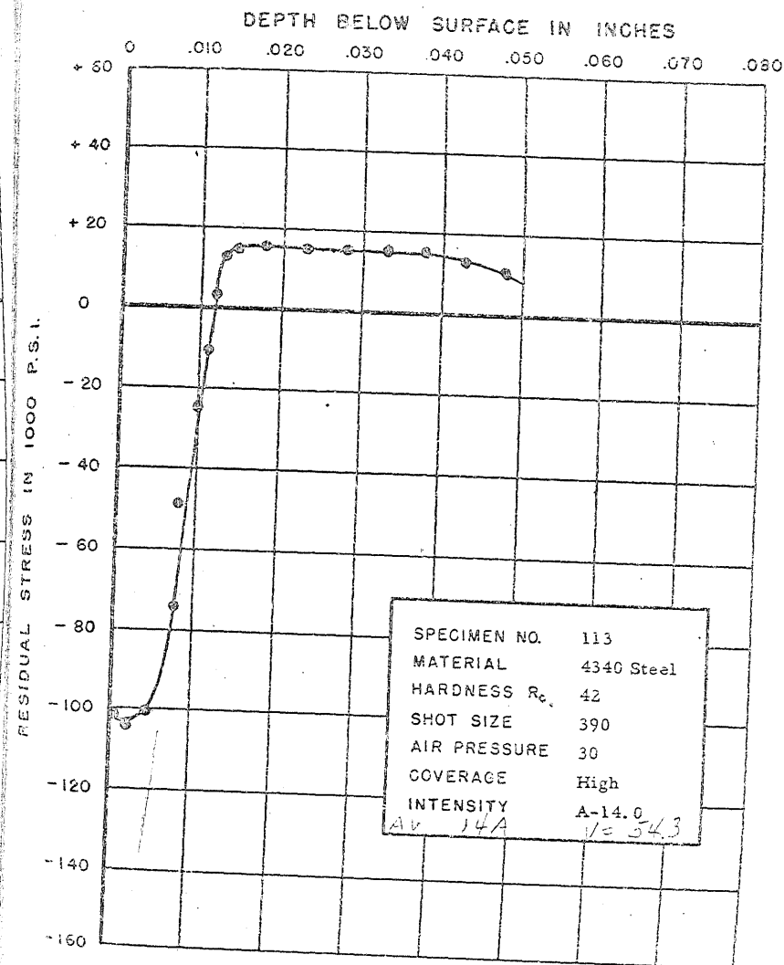
FIGURE 146. RESIDUAL STRESS DISTRIBUTION
