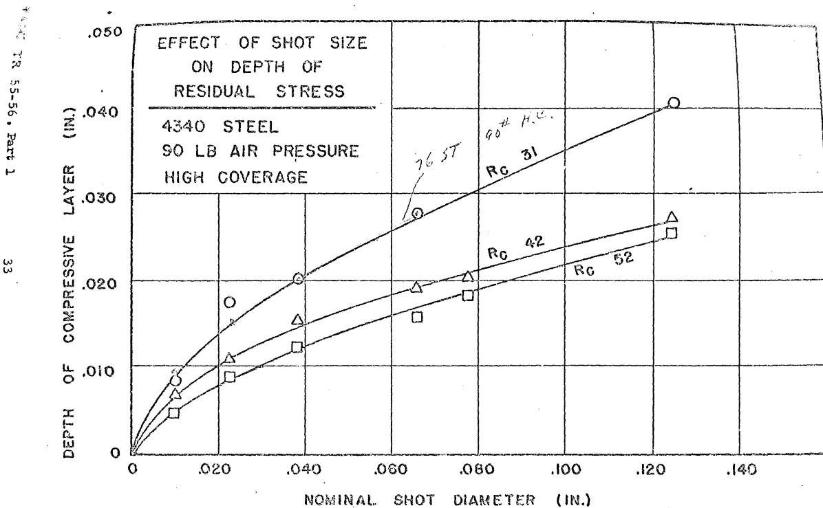
FIGURE 22. EFFECTIVE DEPTH OF PEENING
