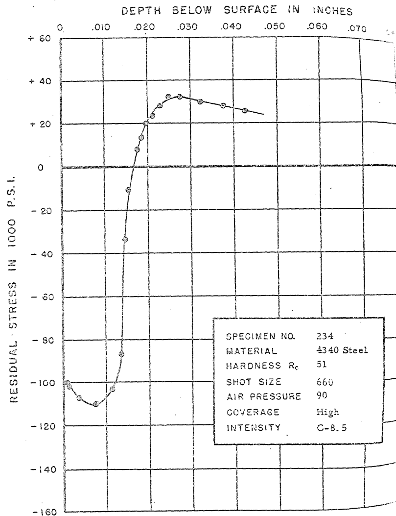
FIGURE 267. RESIDUAL STRESS DISTRIBUTION
