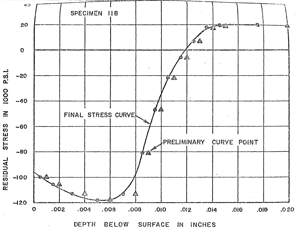
FIGURE 33. SAMPLE RESIDUAL STRESS DISTRIBUTION
