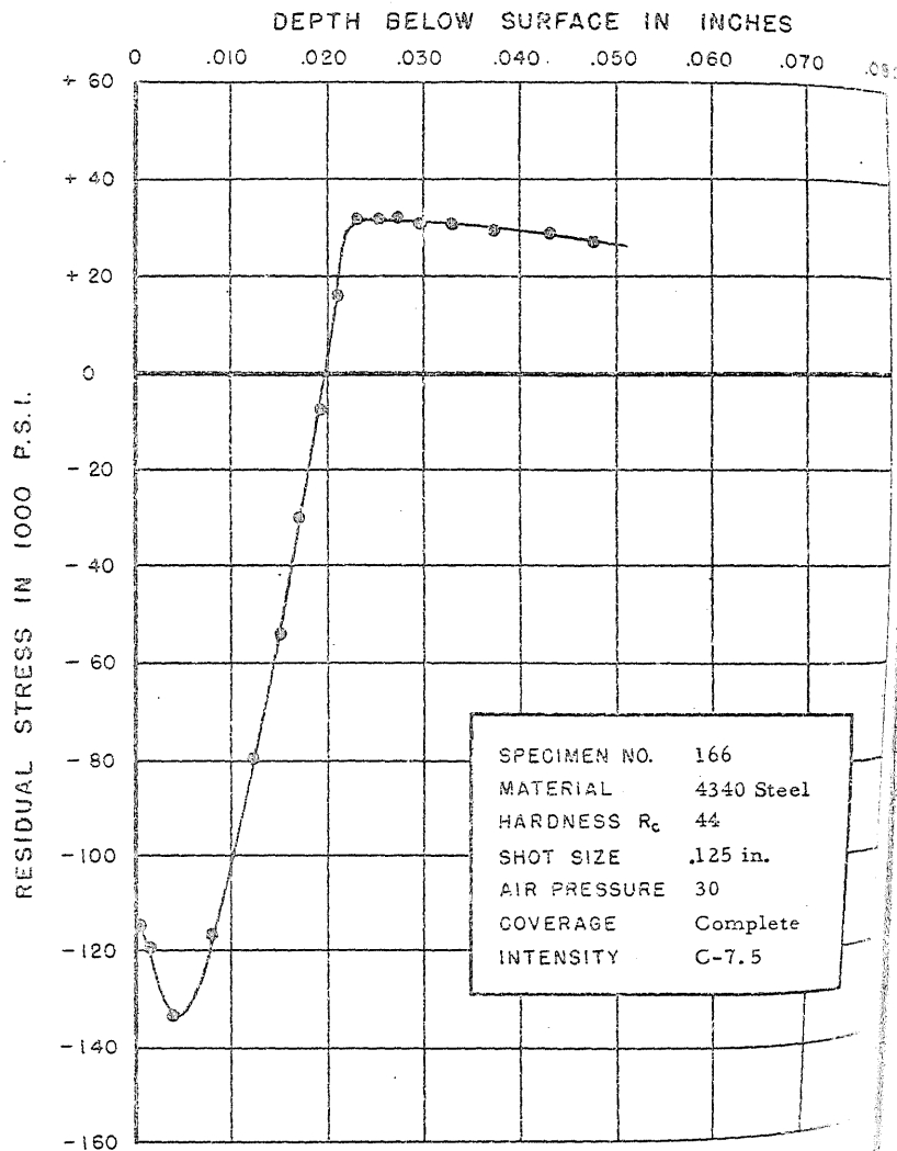
FIGURE 199. RESIDUAL STRESS DISTRIBUTION
