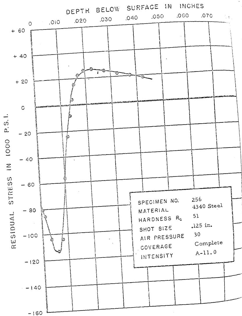
FIGURE 289. RESIDUAL STRESS DISTRIBUTION
