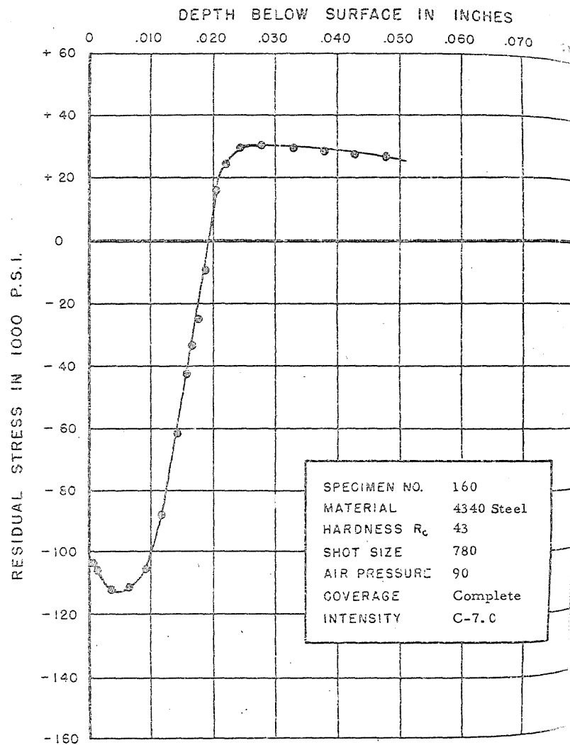
FIGURE 193. RESIDUAL STRESS DISTRIBUTION
