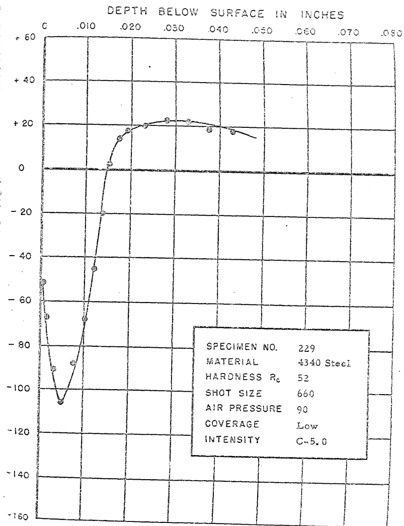
FIGURE 262. RESIDUAL STRESS DISTRIBUTION
