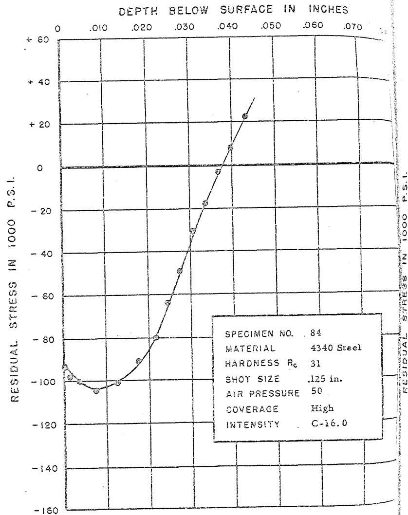
FIGURE 117. RESIDUAL STRESS DISTRIBUTION
