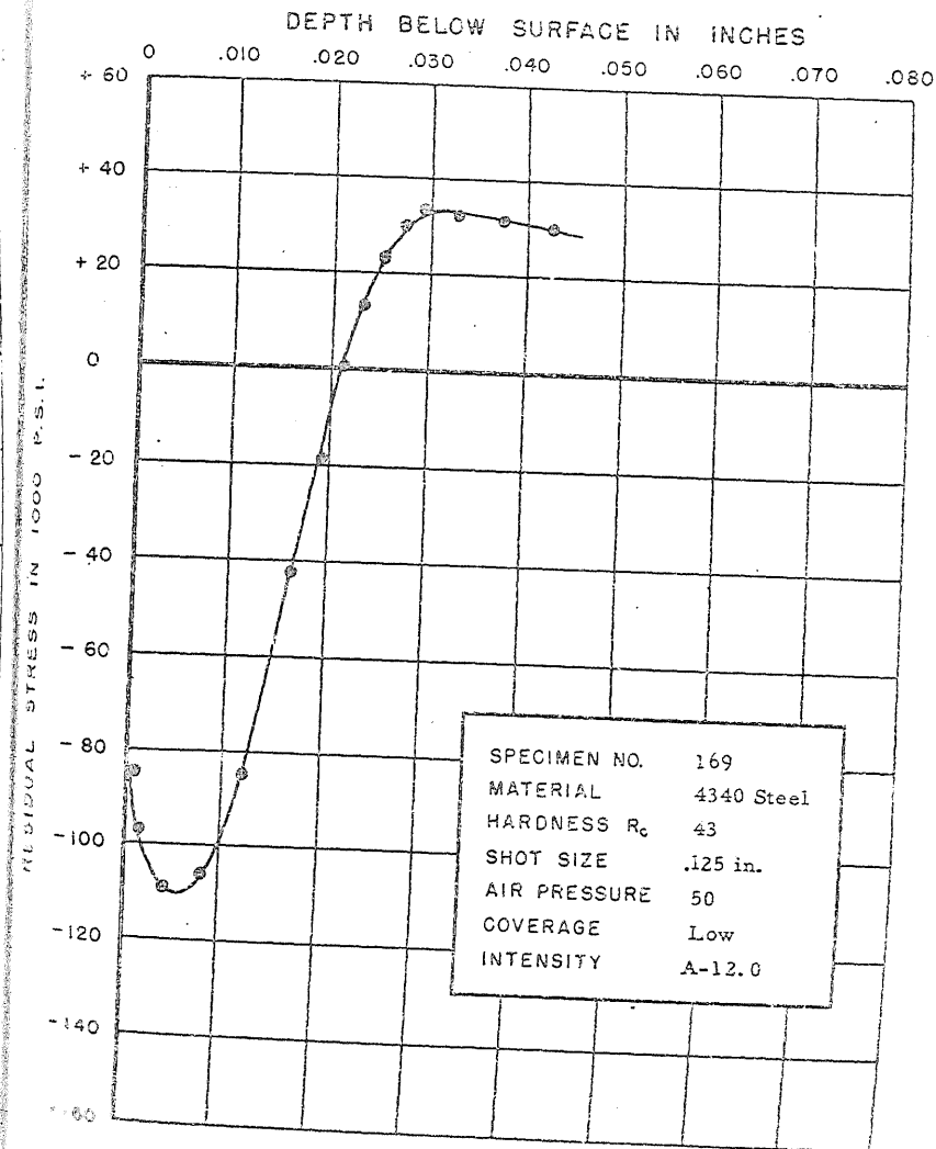
FIGURE 202. RESIDUAL STRESS DISTRIBUTION
