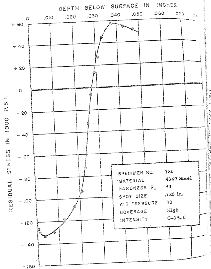
FIGURE 213. RESIDUAL STRESS DISTRIBUTION
