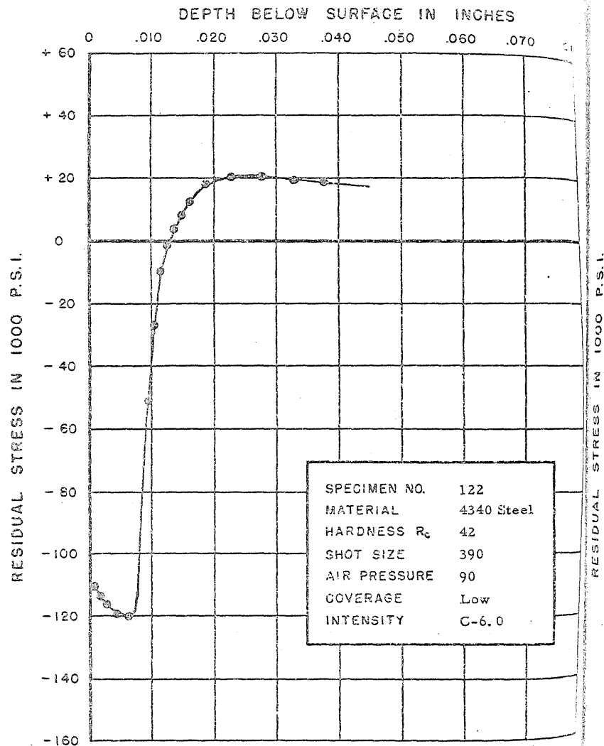
FIGURE 155. RESIDUAL STRESS DISTRIBUTION
