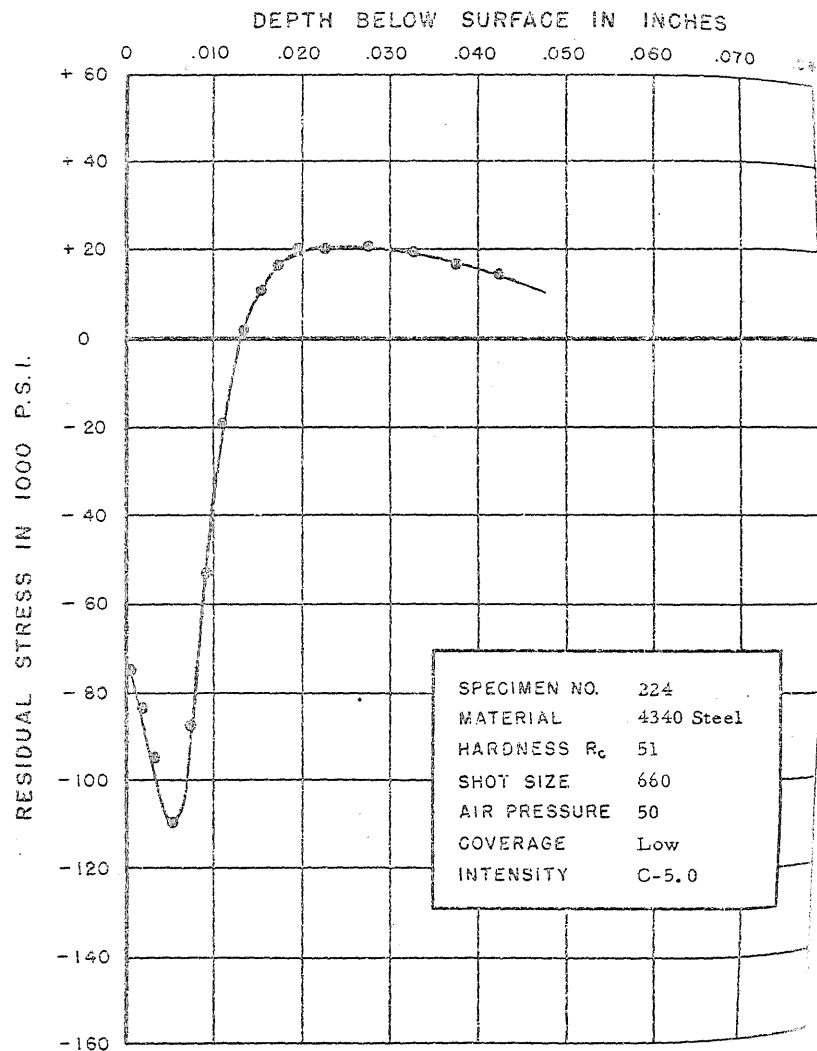
FIGURE 257. RESIDUAL STRESS DISTRIBUTION
