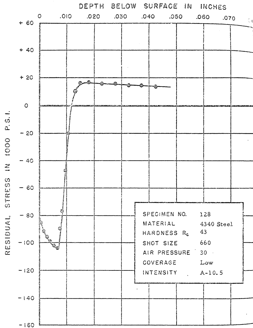
FIGURE 161. RESIDUAL STRESS DISTRIBUTION
