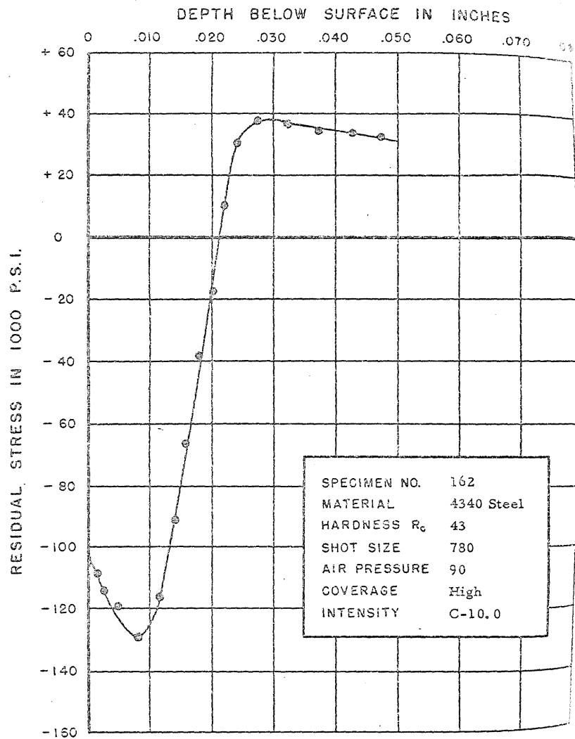
FIGURE 195. RESIDUAL STRESS DISTRIBUTION
