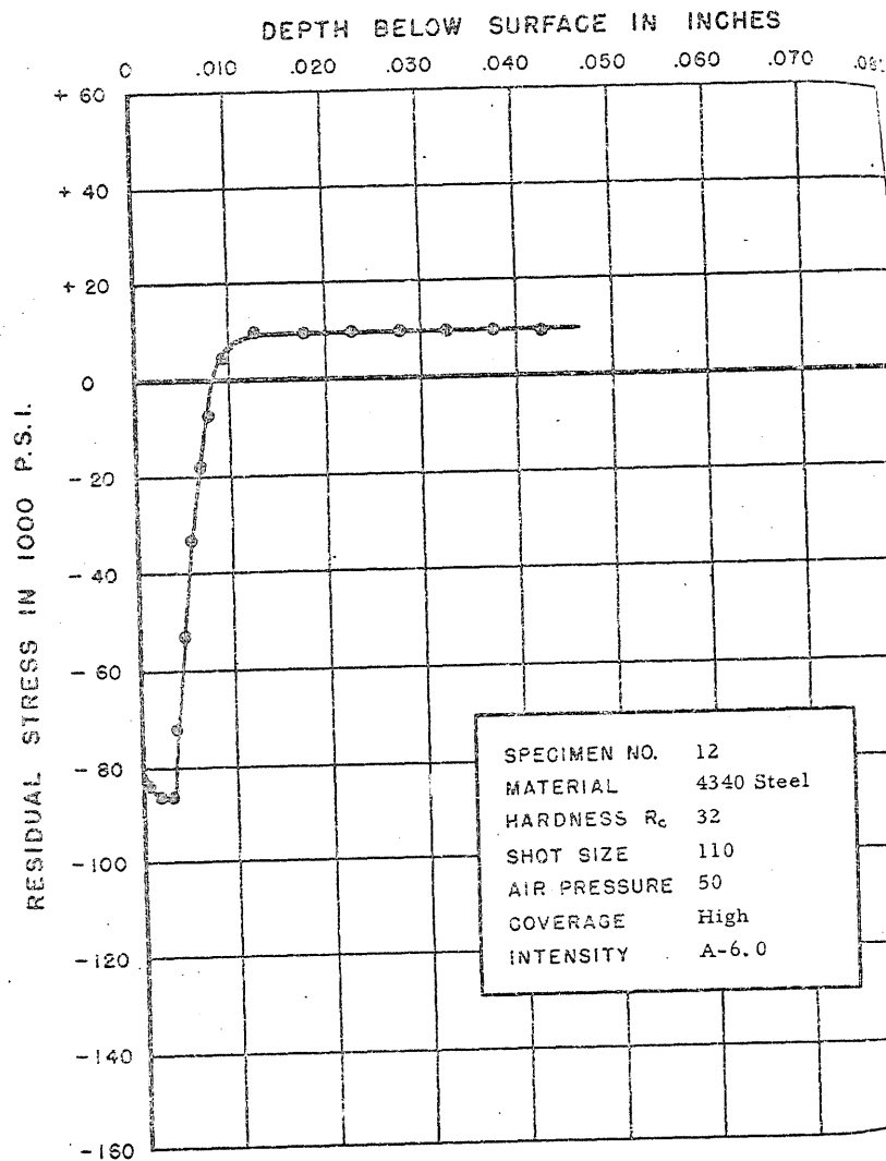
FIGURE 45. RESIDUAL STRESS DISTRIBUTION
