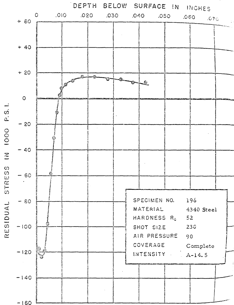
FIGURE 229. RESIDUAL STRESS DISTRIBUTION
