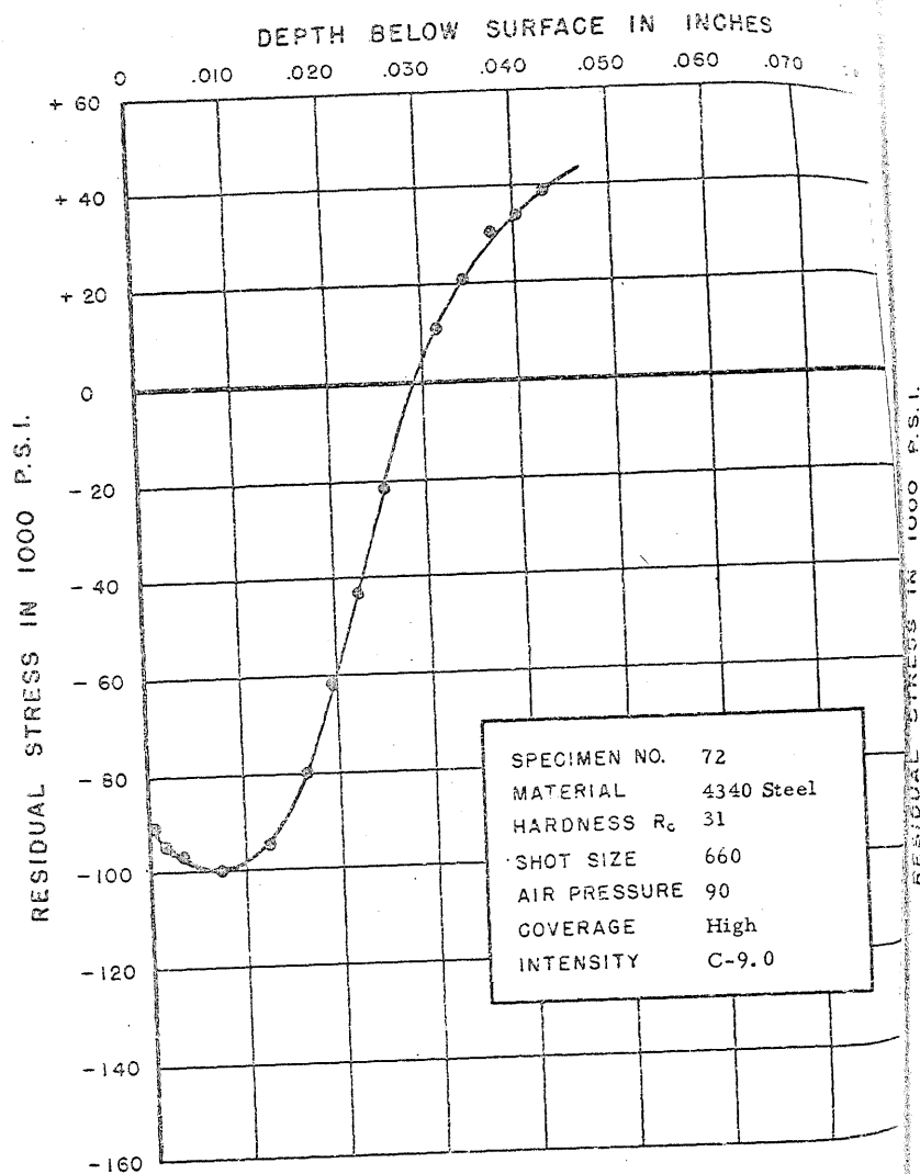
FIGURE 105. RESIDUAL STRESS DISTRIBUTION
