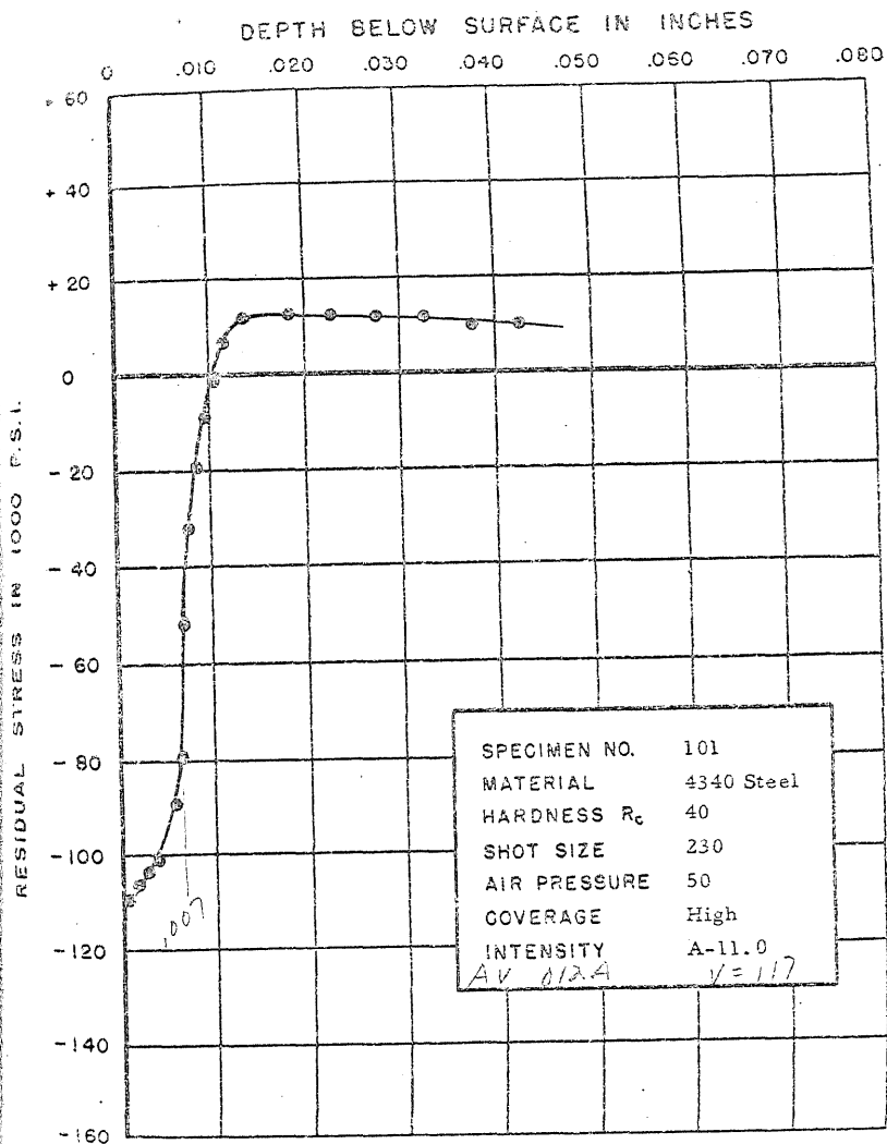
FIGURE 134. RESIDUAL STRESS DISTRIBUTION
