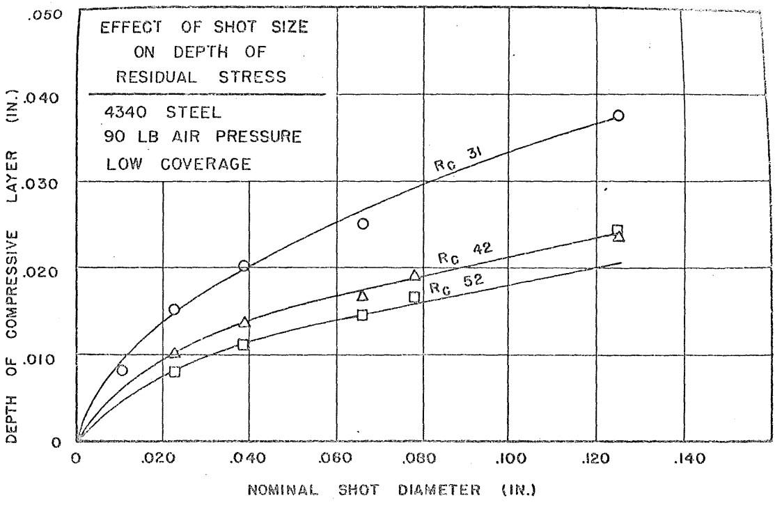
FIGURE 20. EFFECTIVE DEPTH OF PEENING
