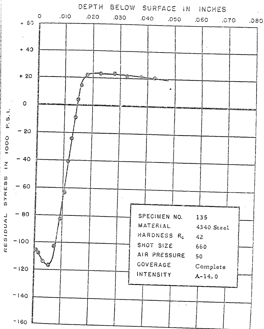
FIGURE 168. RESIDUAL STRESS DISTRIBUTION
