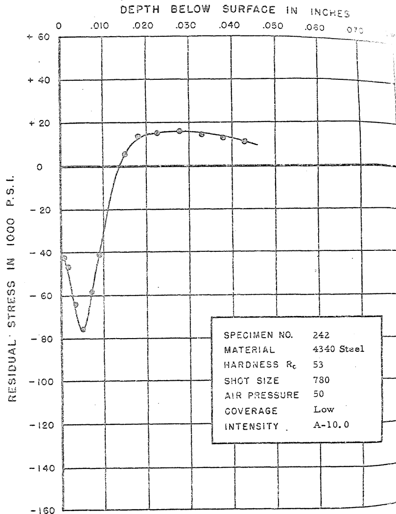
FIGURE 275. RESIDUAL STRESS DISTRIBUTION
