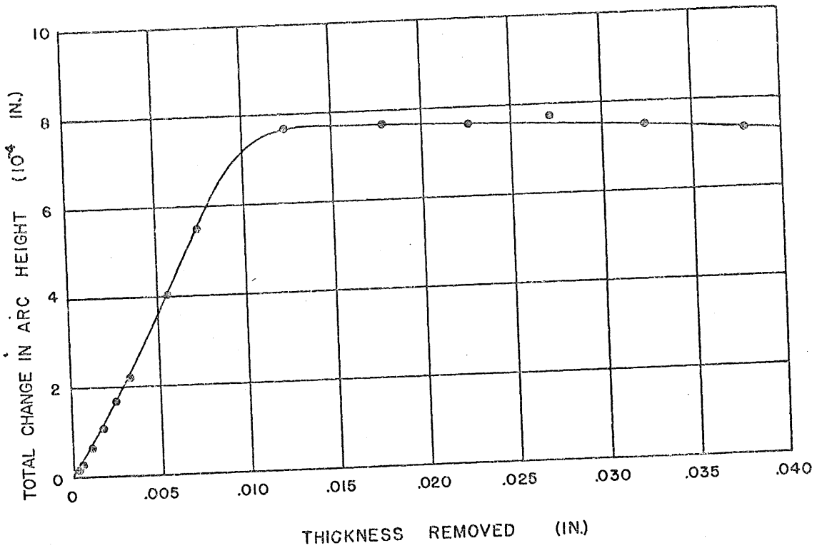
FIGURE 32. CHANGE IN ARC HEIGHT VERSUS THICKNESS REMOVED FOR SPECIMEN NO. 118
