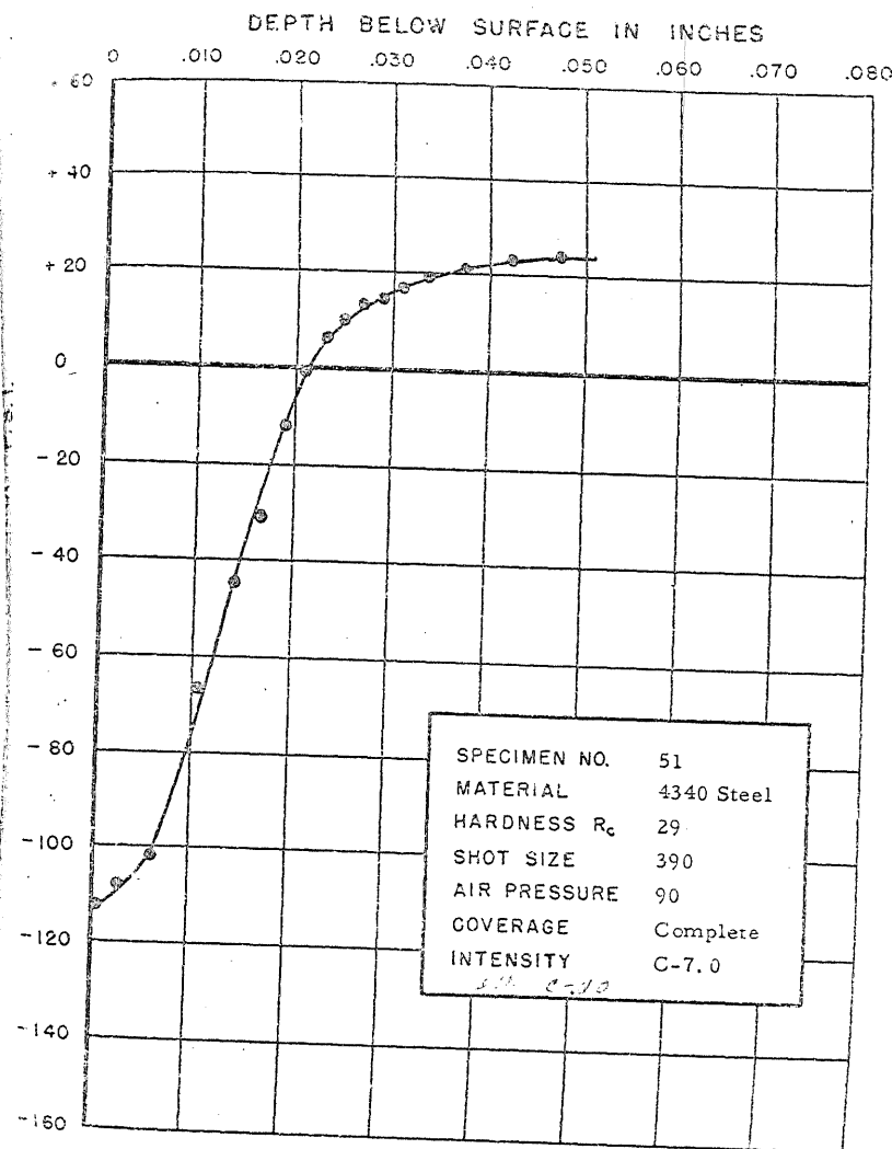
FIGURE 84. RESIDUAL STRESS DISTRIBUTION
