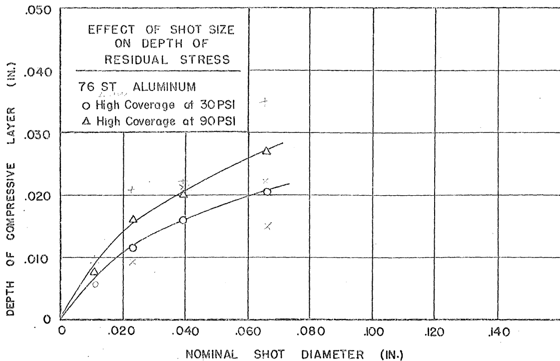
FIGURE 23. EFFECTIVE DEPTH OF PEENING
