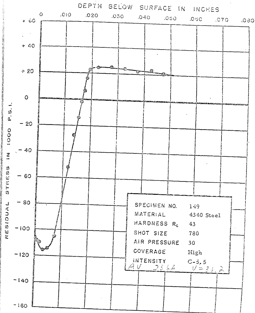
FIGURE 182. RESIDUAL STRESS DISTRIBUTION
