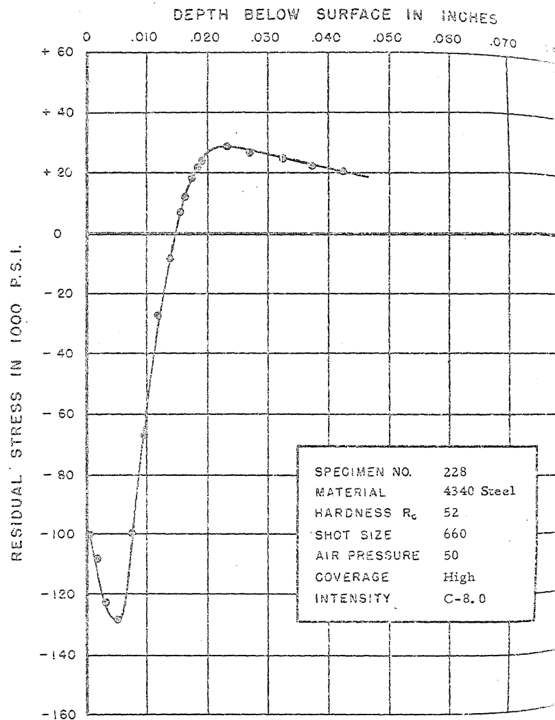
FIGURE 261. RESIDUAL STRESS DISTRIBUTION
