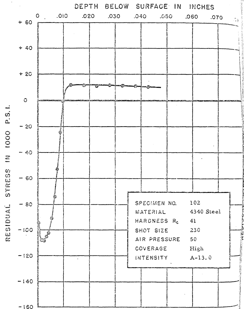
FIGURE 135 RESIDUAL STRESS DISTRIBUTION
