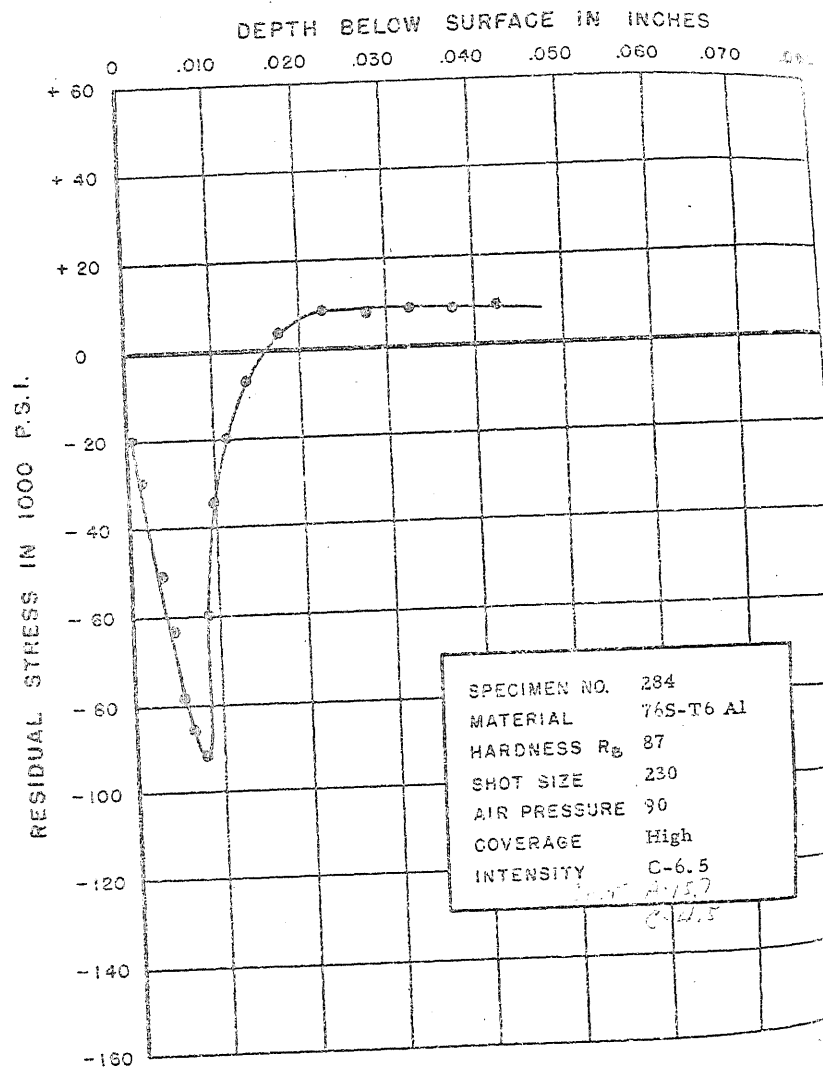
FIGURE 317. RESIDUAL STRESS DISTRIBUTION
