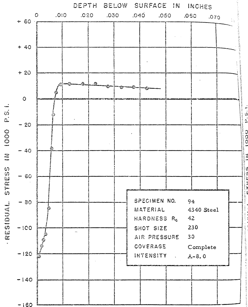
FIGURE 127. RESIDUAL STRESS DISTRIBUTION
