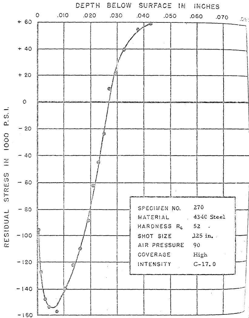
FIGURE 303. RESIDUAL STRESS DISTRIBUTION
