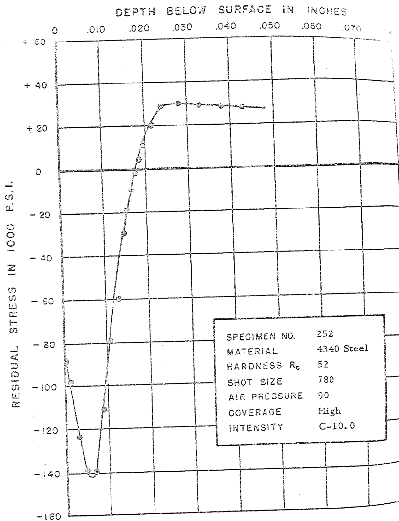
FIGURE 285. RESIDUAL STRESS DISTRIBUTION
