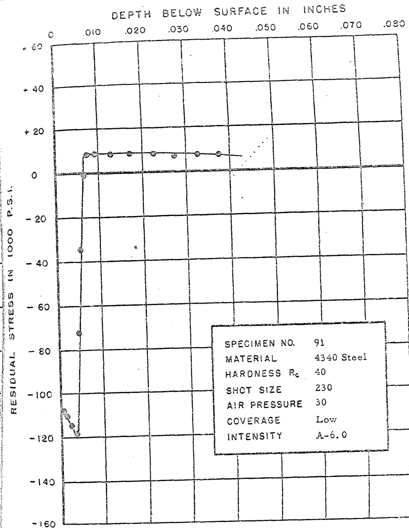
FIGURE 124. RESIDUAL STRESS DISTRIBUTION
