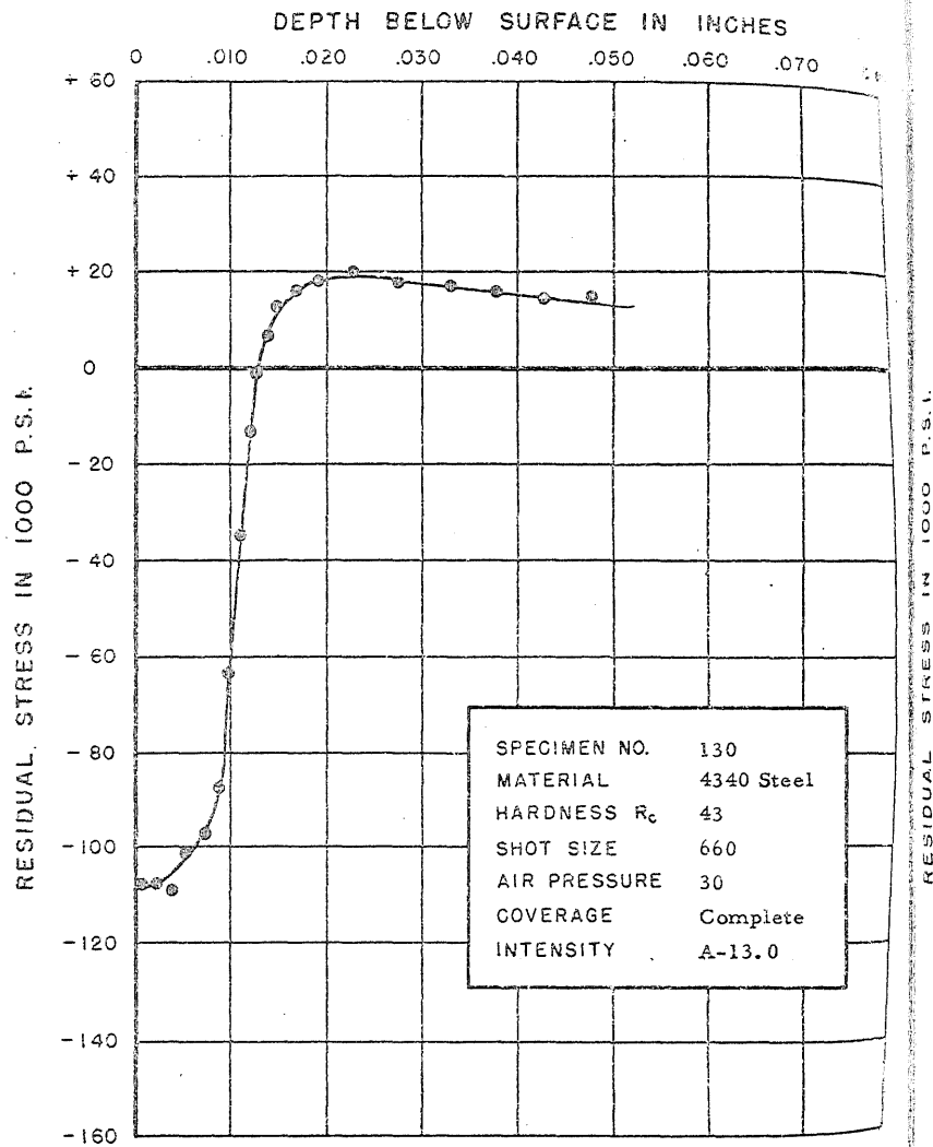
FIGURE 163. RESIDUAL STRESS DISTRIBUTION
