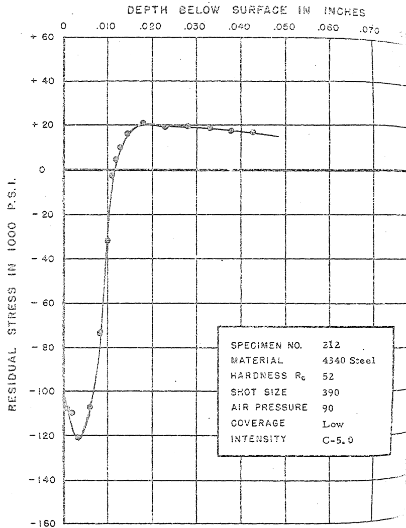
FIGURE 245. RESIDUAL STRESS DISTRIBUTION
