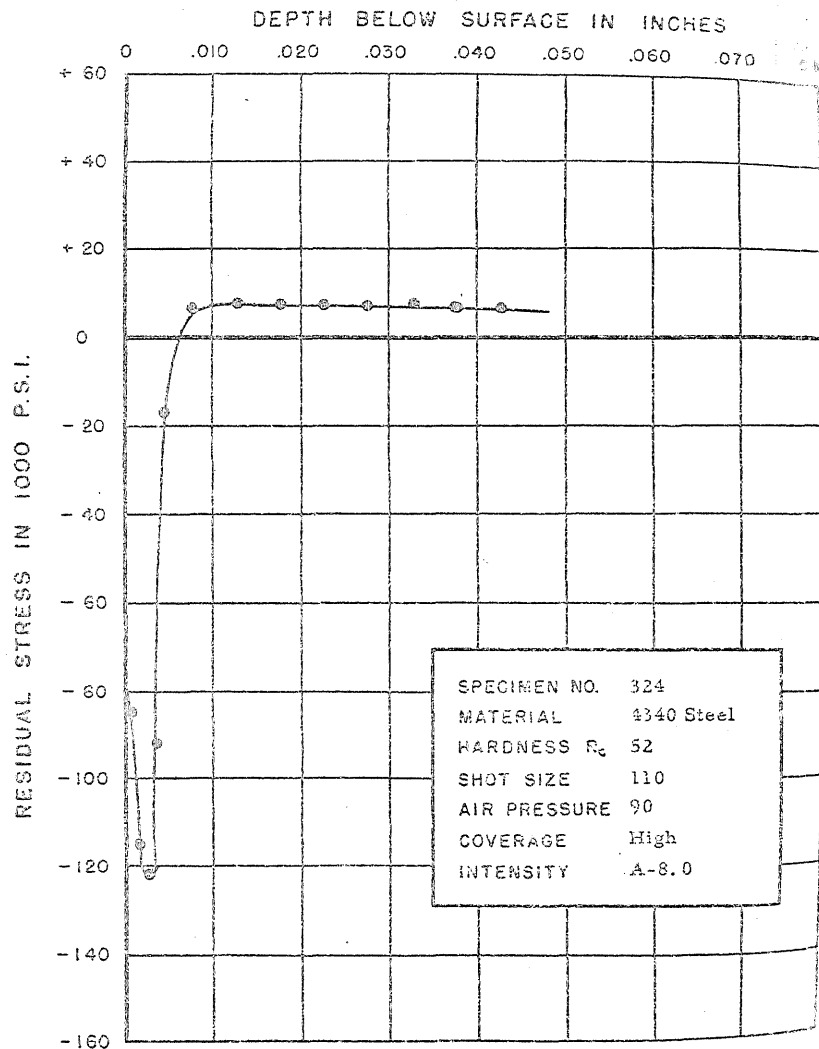
FIGURE 357. RESIDUAL STRESS DISTRIBUTION
