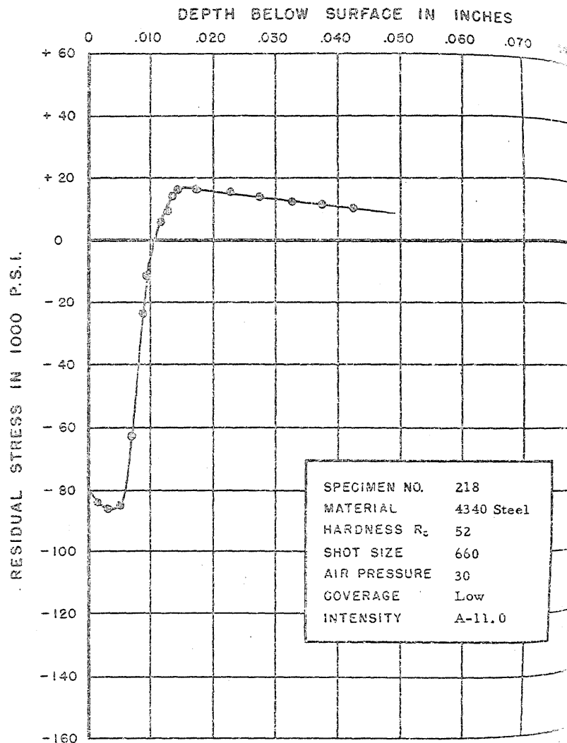
FIGURE 251. RESIDUAL STRESS DISTRIBUTION
