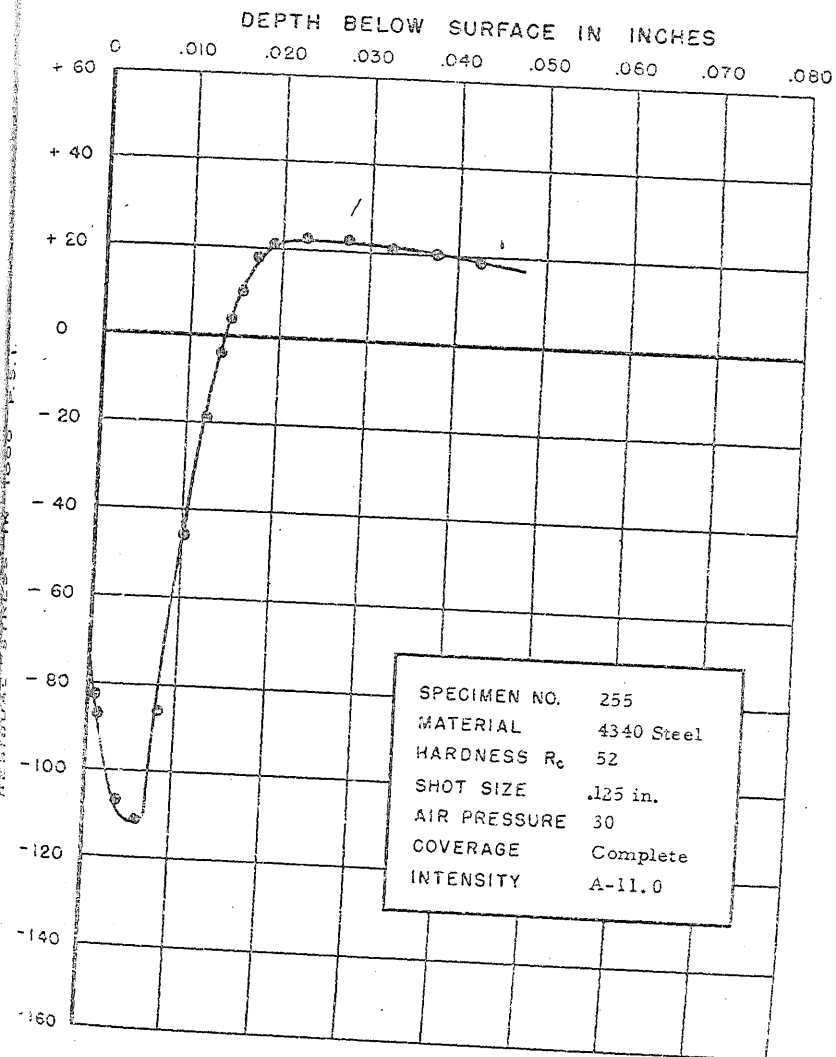
FIGURE 288. RESIDUAL STRESS DISTRIBUTION
