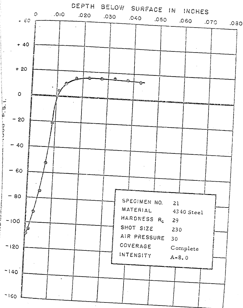
FIGURE 54. RESIDUAL STRESS DISTRIBUTION
