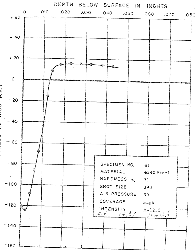
FIGURE 74. RESIDUAL STRESS DISTRIBUTION
