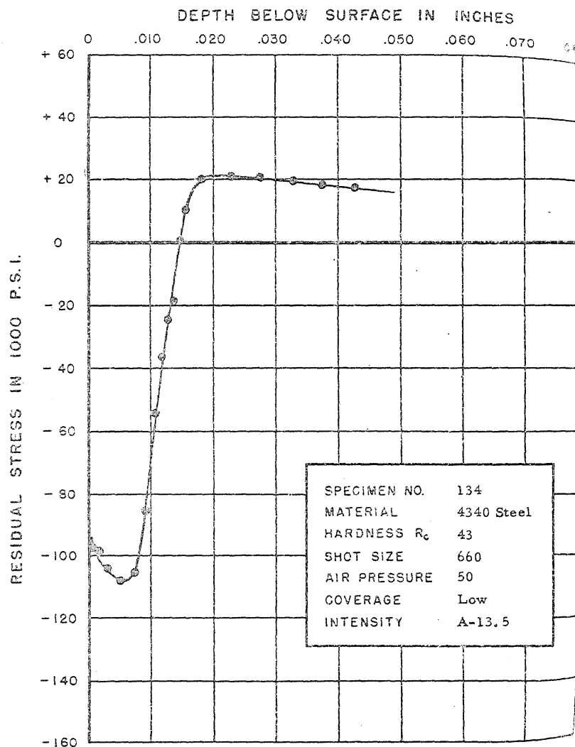
FIGURE 167. RESIDUAL STRESS DISTRIBUTION
