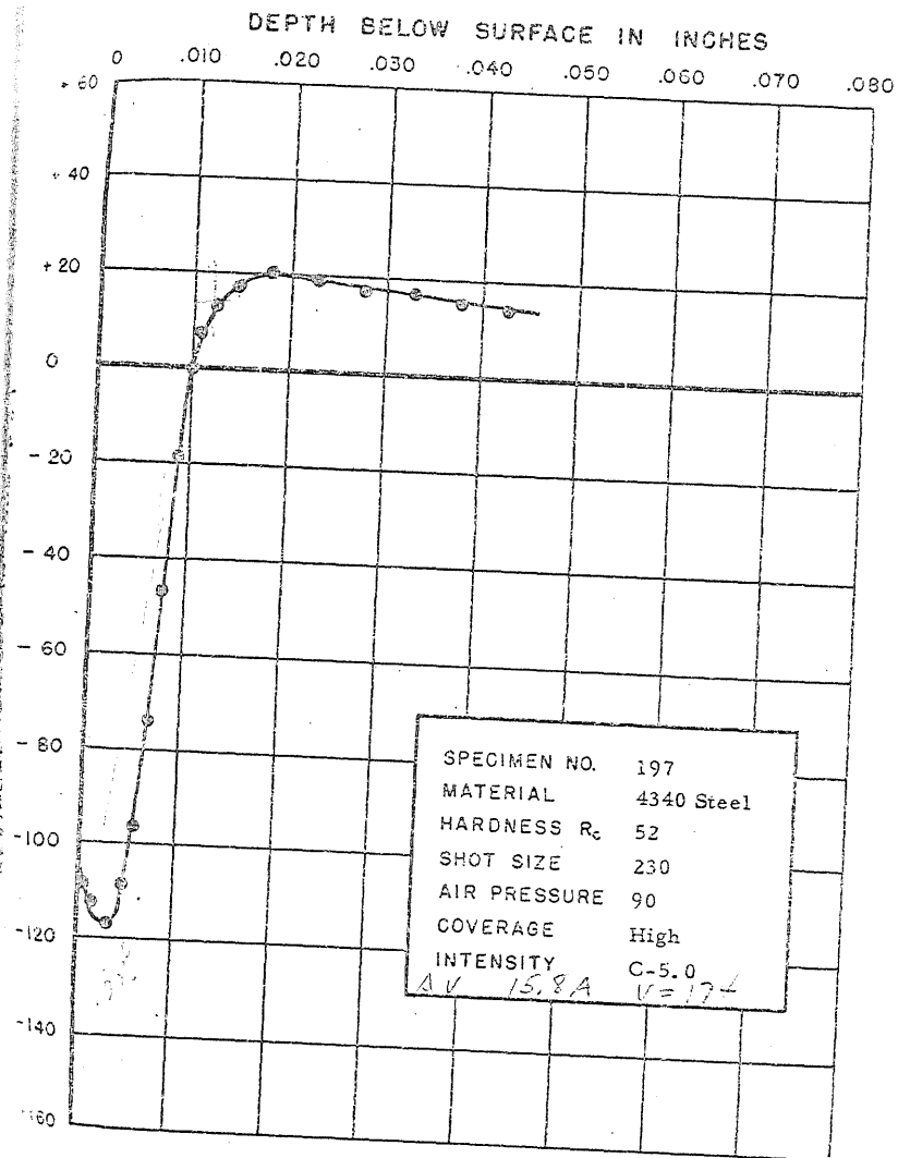
FIGURE 230. RESIDUAL STRESS DISTRIBUTION
