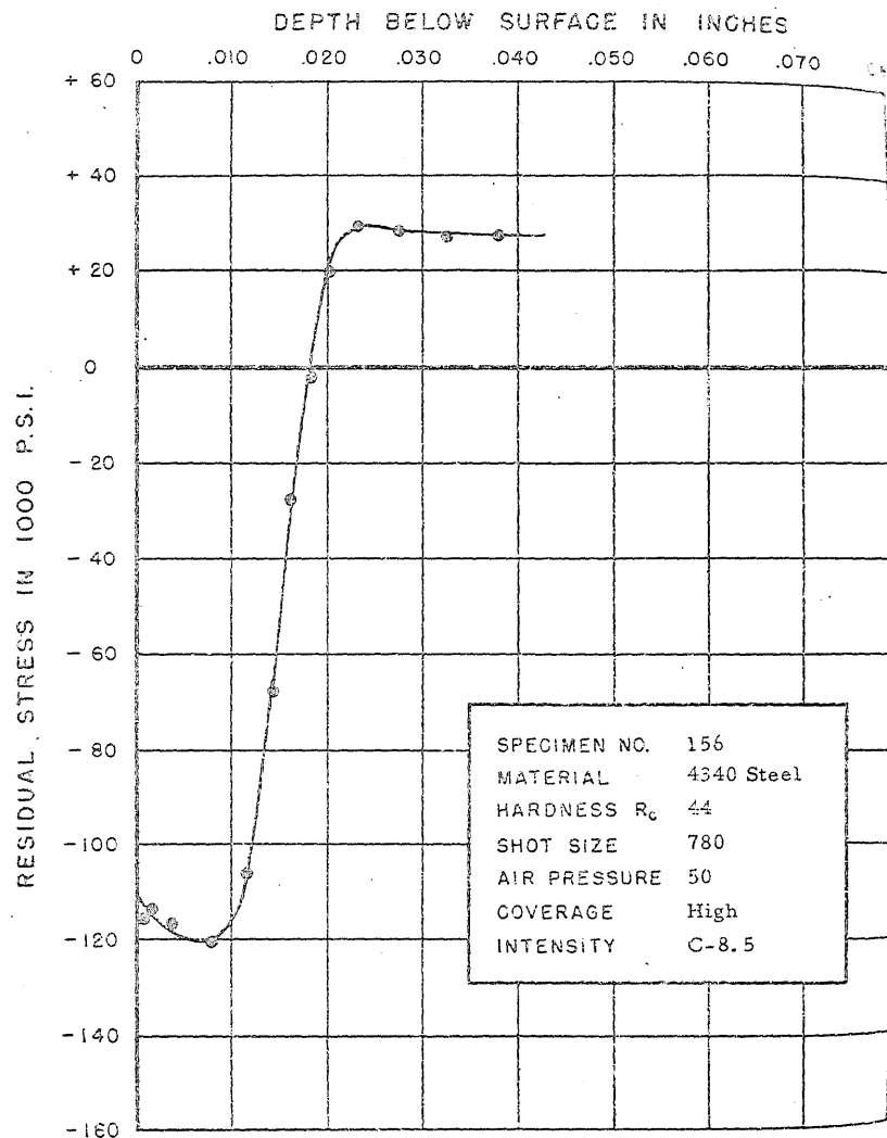
FIGURE 189. RESIDUAL STRESS DISTRIBUTION
