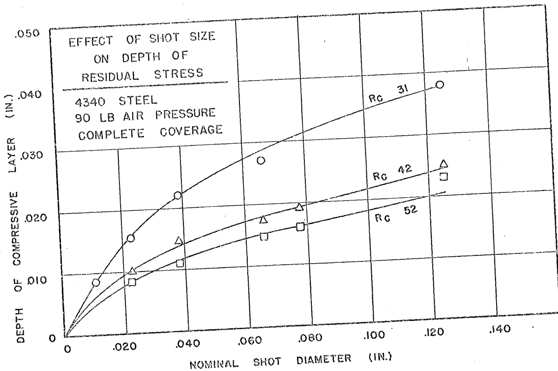
FIGURE 21. EFFECTIVE DEPTH OF PEENING
