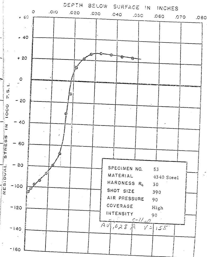
FIGURE 86. RESIDUAL STRESS DISTRIBUTION
