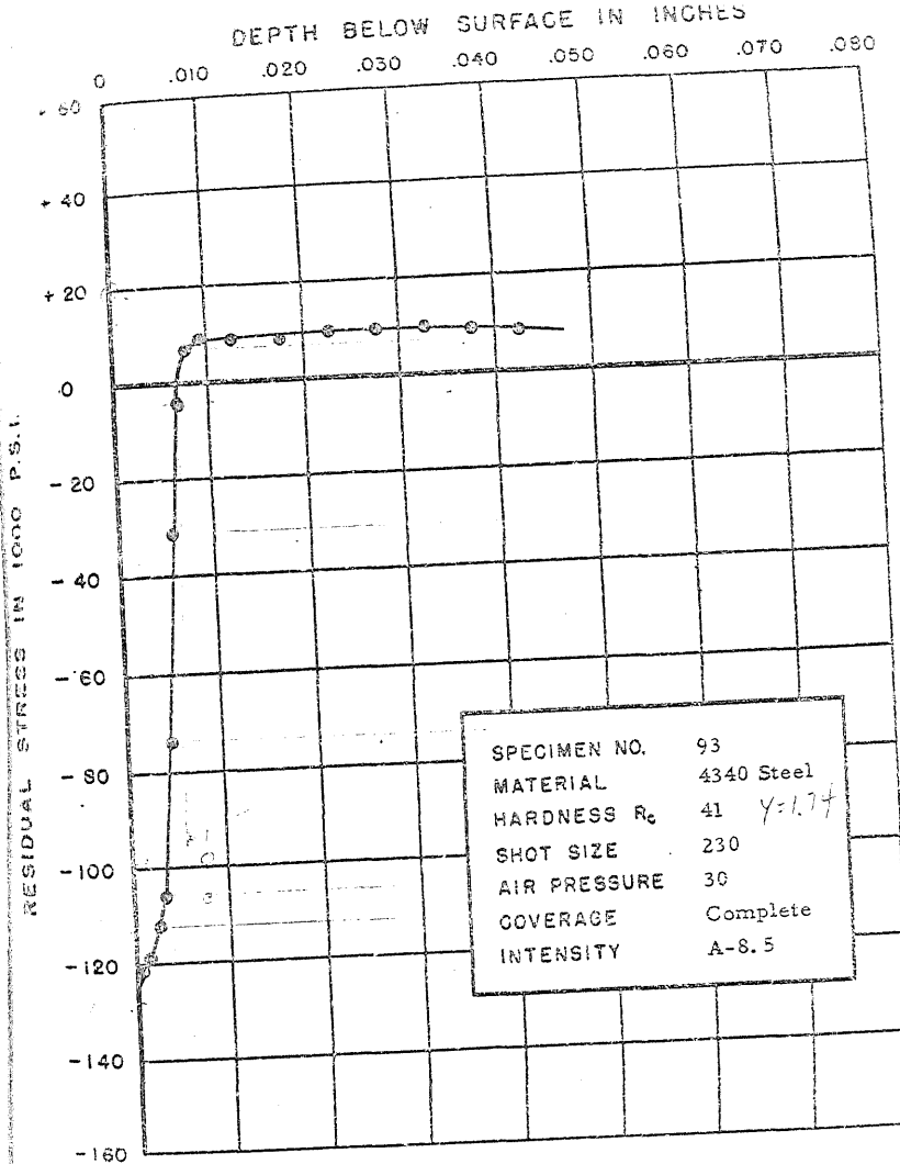
FIGURE 126. RESIDUAL STRESS DISTRIBUTION
