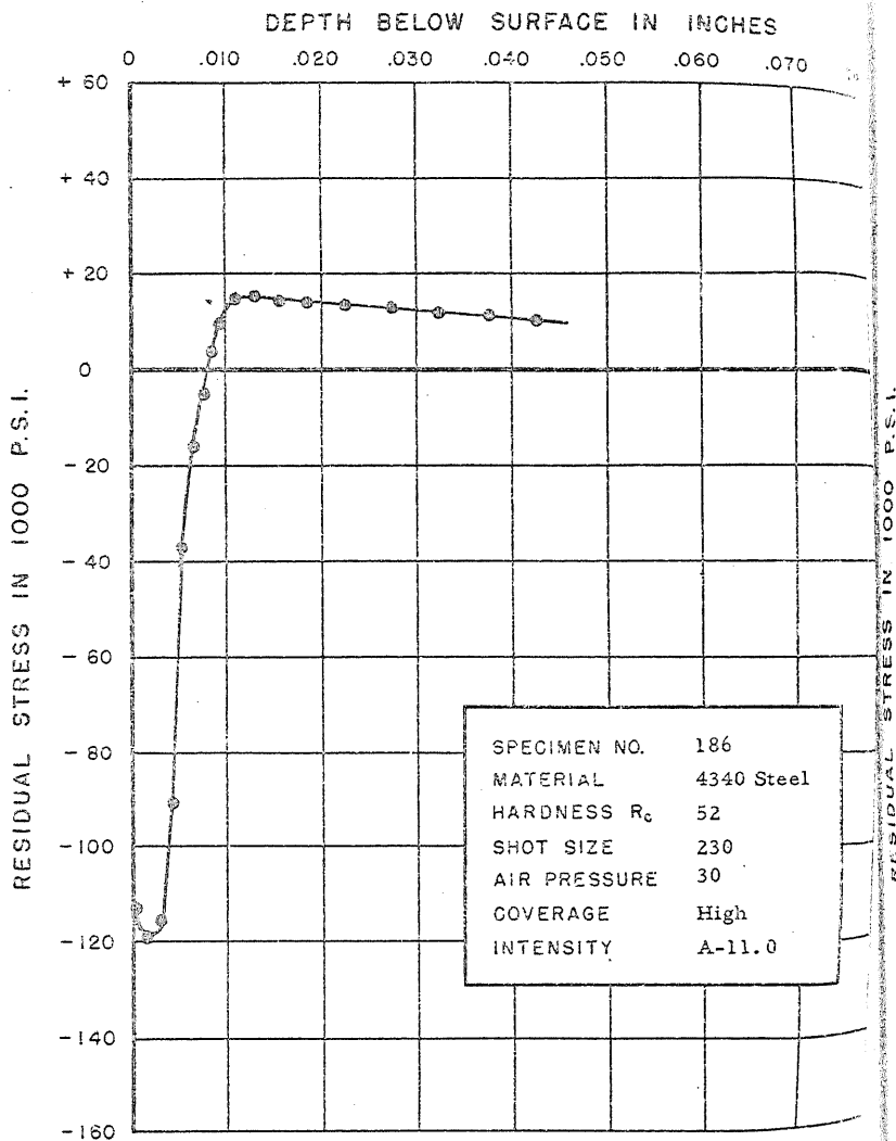
FIGURE 219. RESIDUAL STRESS DISTRIBUTION
