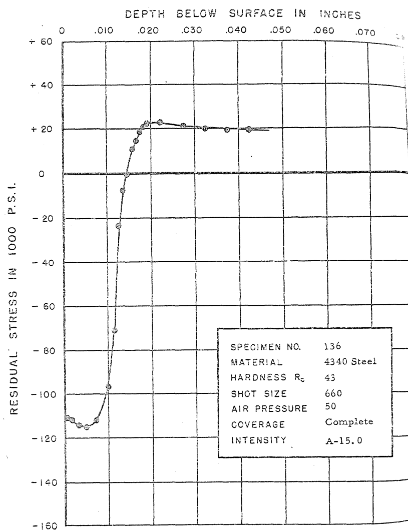
FIGURE 169. RESIDUAL STRESS DISTRIBUTION
