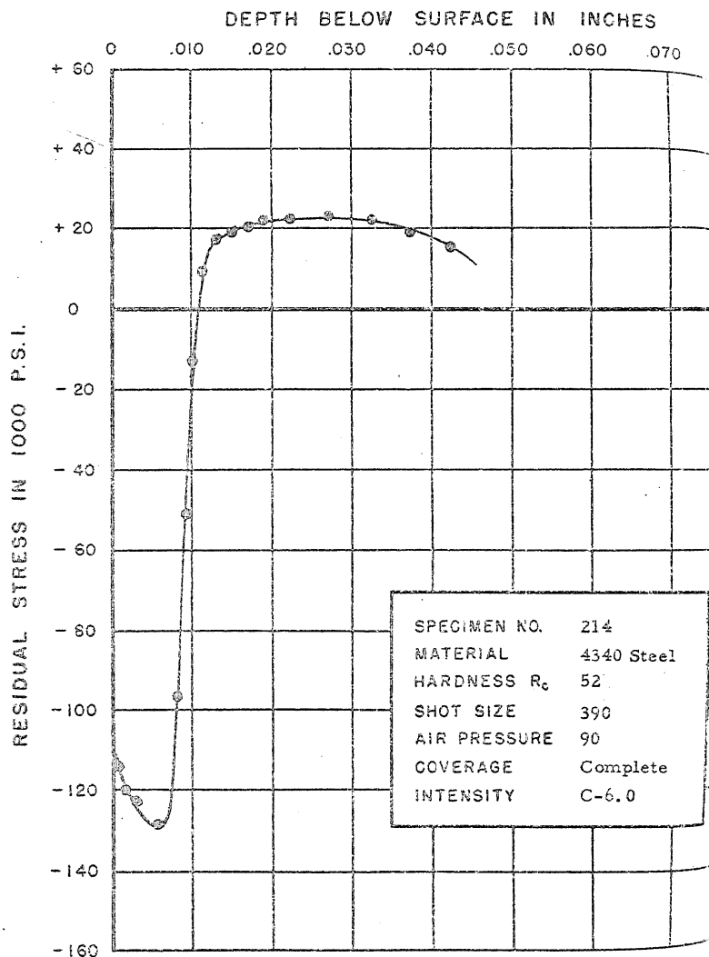
FIGURE 247. RESIDUAL STRESS DISTRIBUTION
