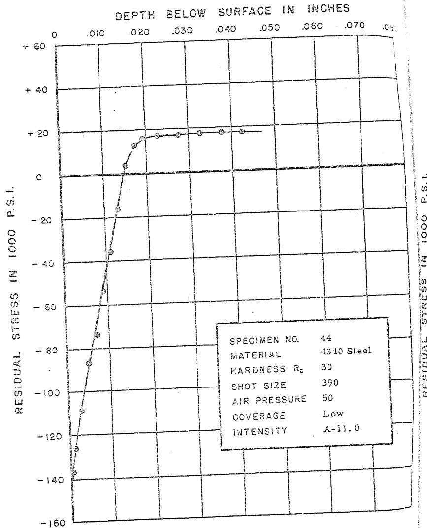
FIGURE 77. RESIDUAL STRESS DISTRIBUTION
