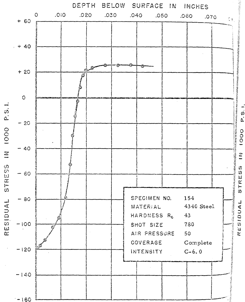
FIGURE 187. RESIDUAL STRESS DISTRIBUTION*
