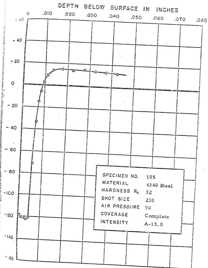
FIGURE 228. RESIDUAL STRESS DISTRIBUTION
