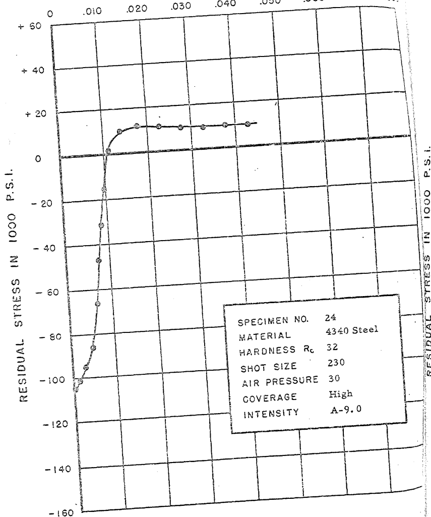
FIGURE 57. RESIDUAL STRESS DISTRIBUTION
