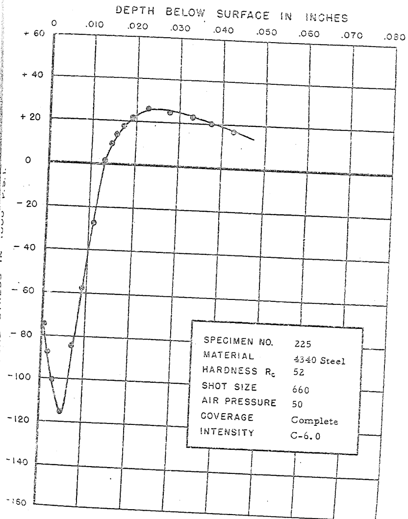
FIGURE 258. RESIDUAL STRESS DISTRIBUTION
