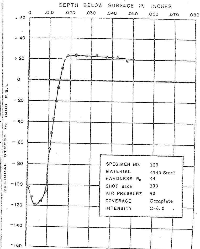
FIGURE 156. RESIDUAL STRESS DISTRIBUTION
