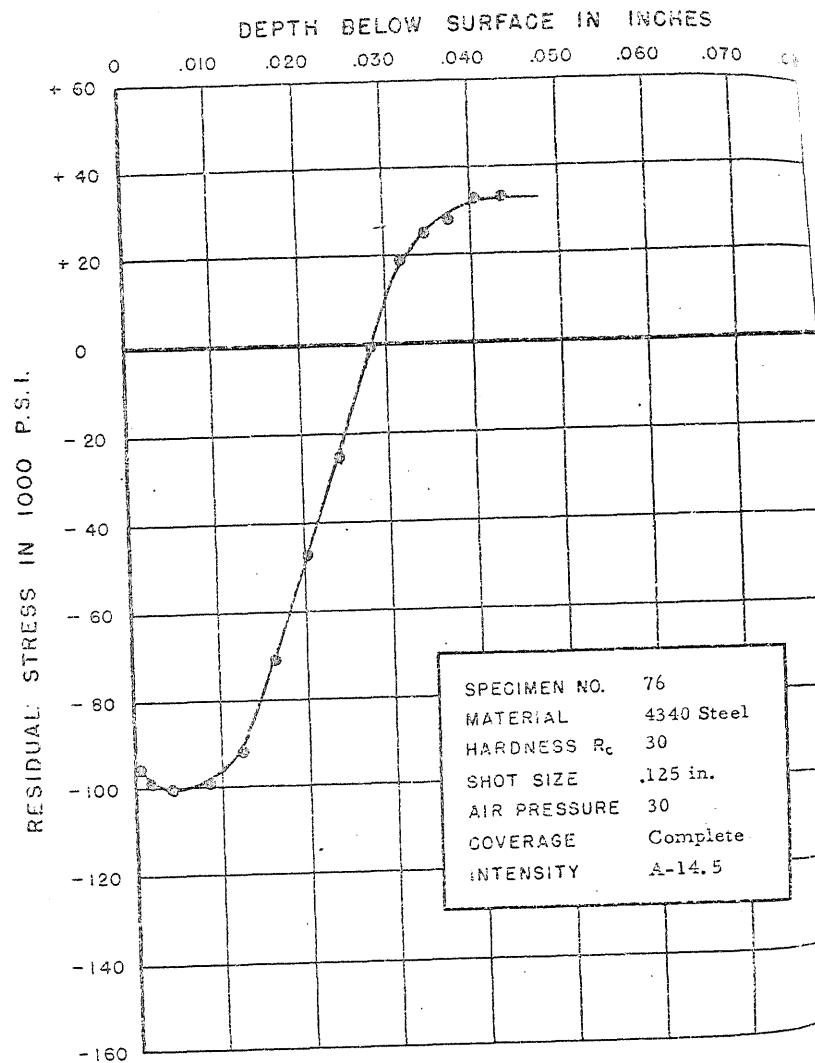
FIGURE 109. RESIDUAL STRESS DISTRIBUTION
