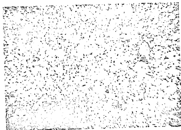
Figure 3. Microstructure of AISI 4340 ( R_c 42) - 1475° F O. Q. 900° F Draw Nital Etch (250X)
