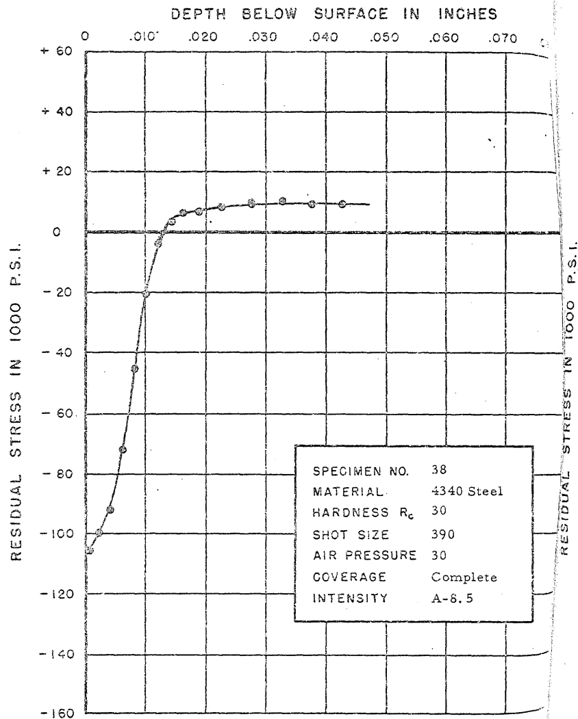
FIGURE 71. RESIDUAL STRESS DISTRIBUTION
