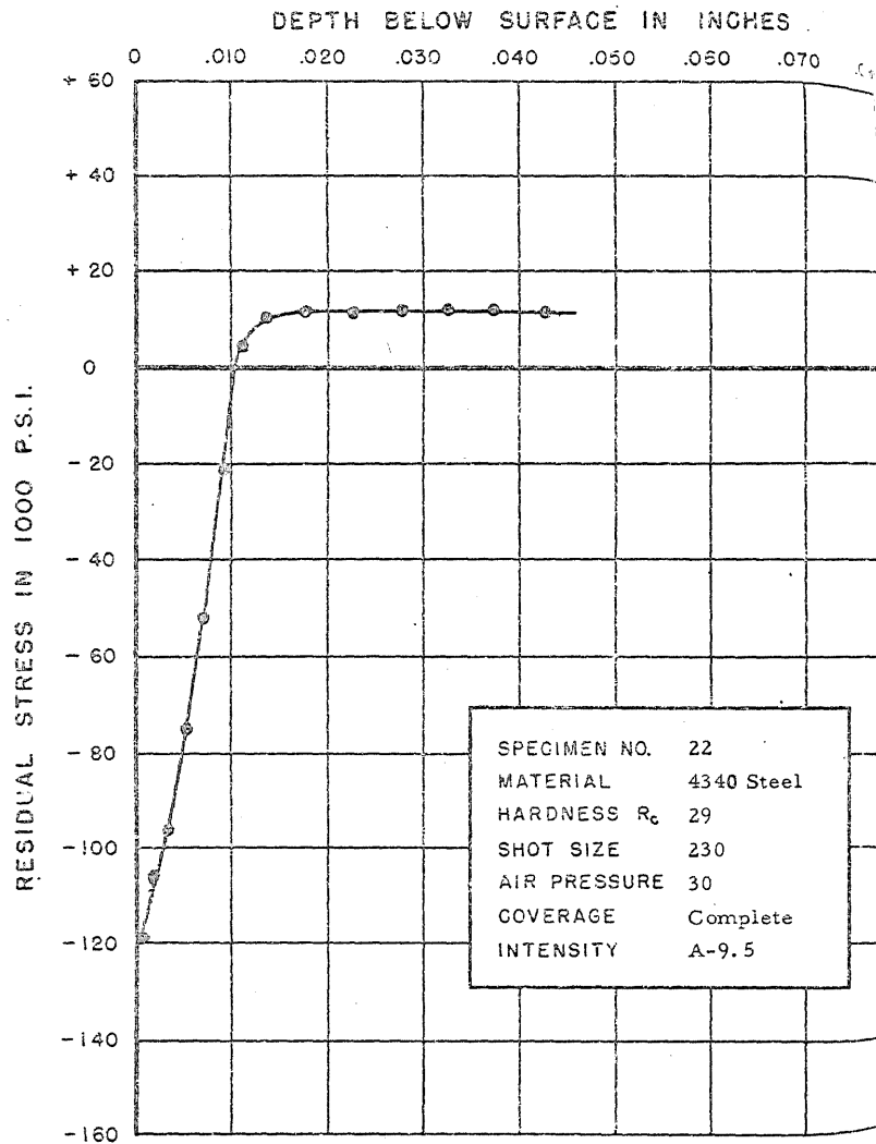
FIGURE 55. RESIDUAL STRESS DISTRIBUTION
