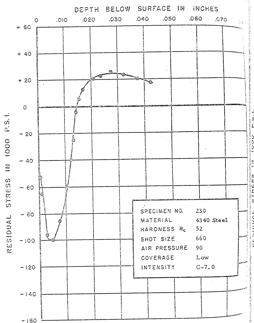
FIGURE 263. RESIDUAL STRESS DISTRIBUTION
