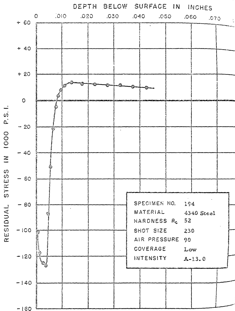
FIGURE 227. RESIDUAL STRESS DISTRIBUTION
