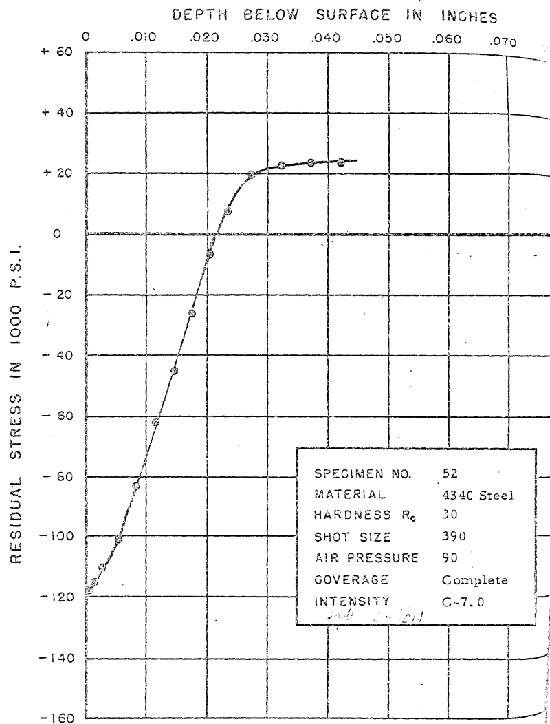
FIGURE 85. RESIDUAL STRESS DISTRIBUTION
