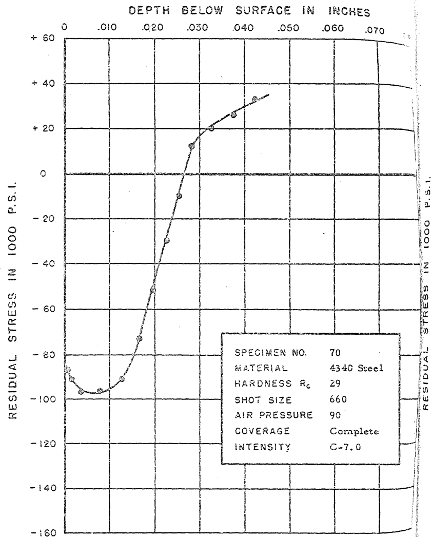
FIGURE 103. RESIDUAL STRESS DISTRIBUTION
