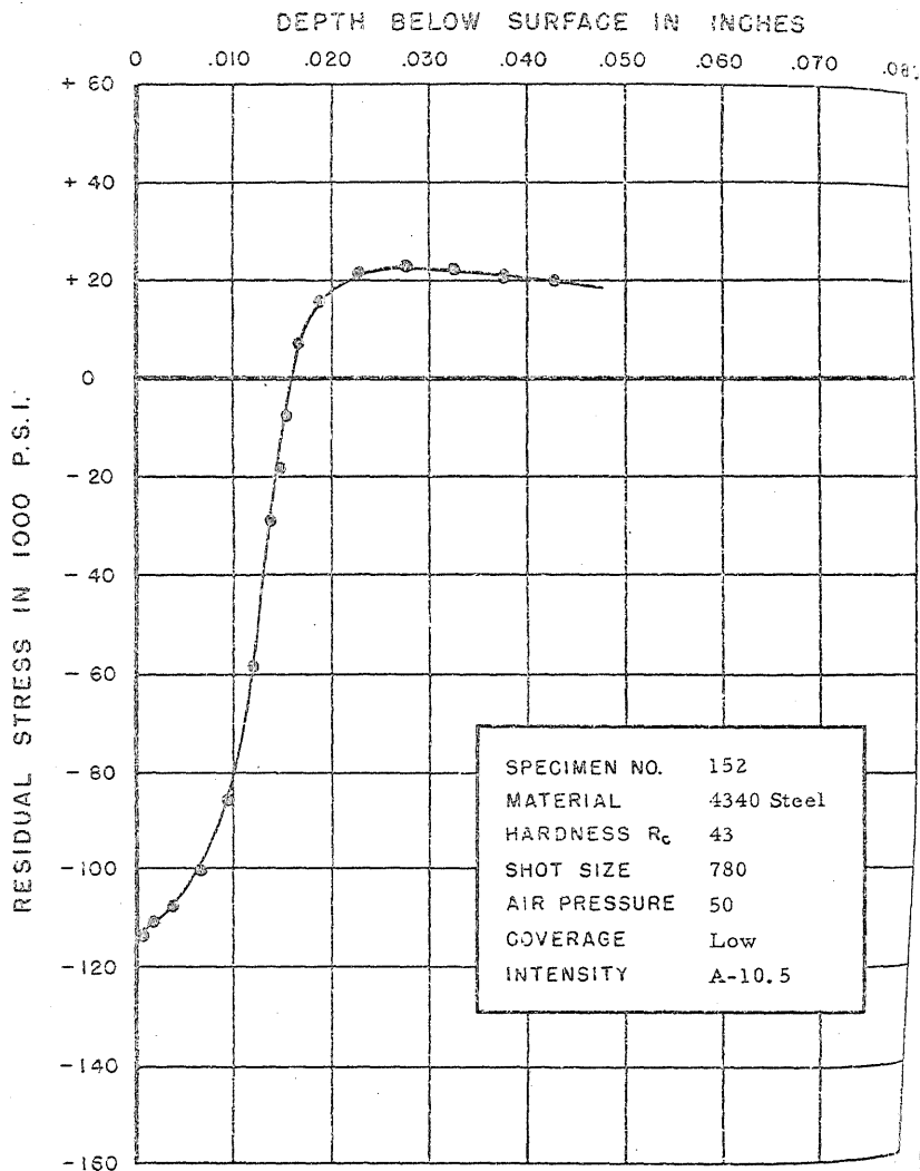
FIGURE 185. RESIDUAL STRESS DISTRIBUTION
