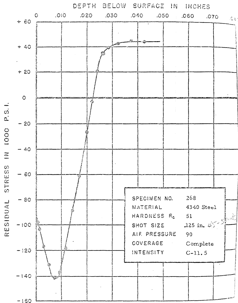
FIGURE 301. RESIDUAL STRESS DISTRIBUTION
