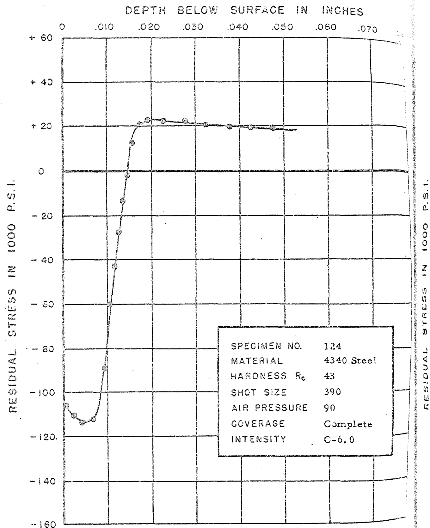
FIGURE 157. RESIDUAL STRESS DISTRIBUTION
