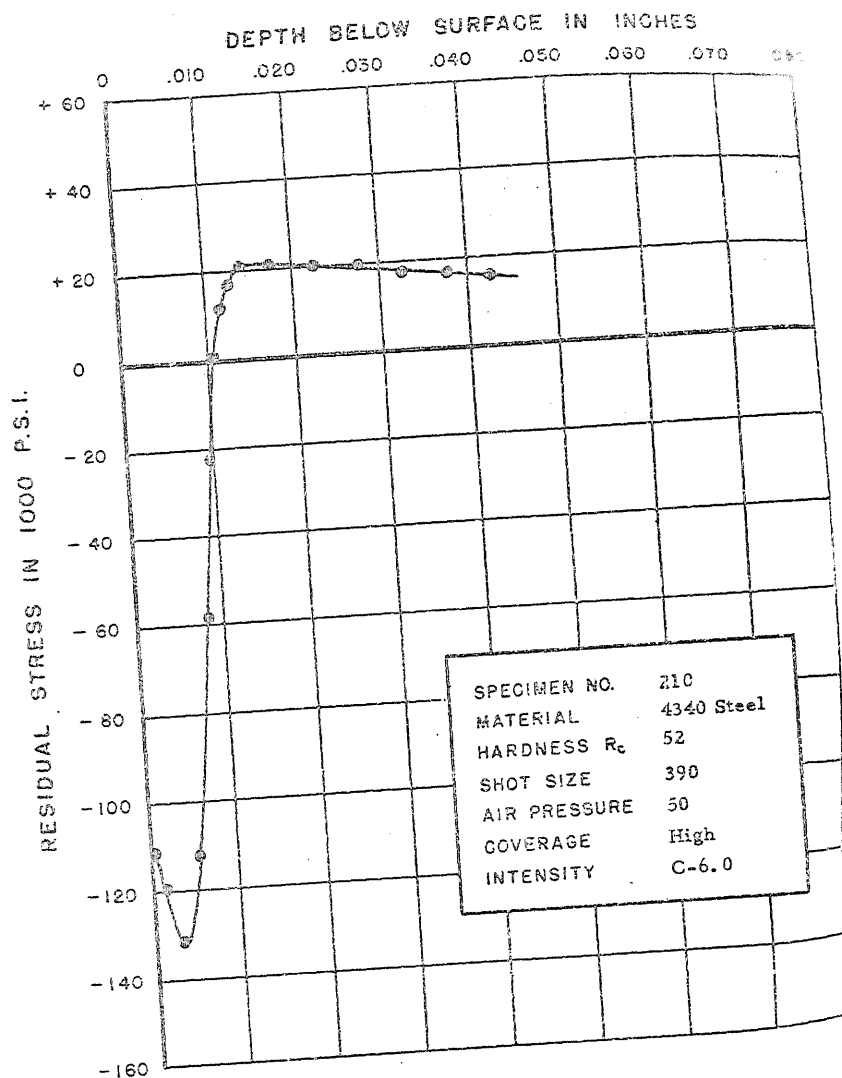
FIGURE 243. RESIDUAL STRESS DISTRIBUTION
