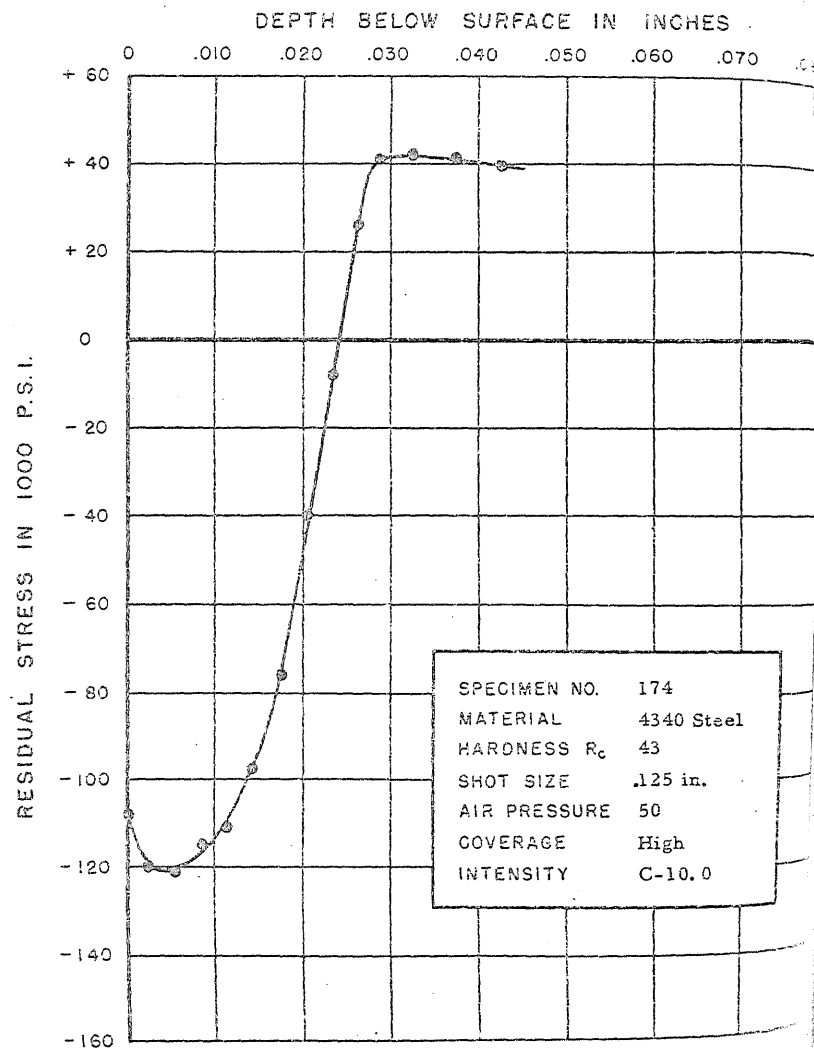
FIGURE 207. RESIDUAL STRESS DISTRIBUTION
