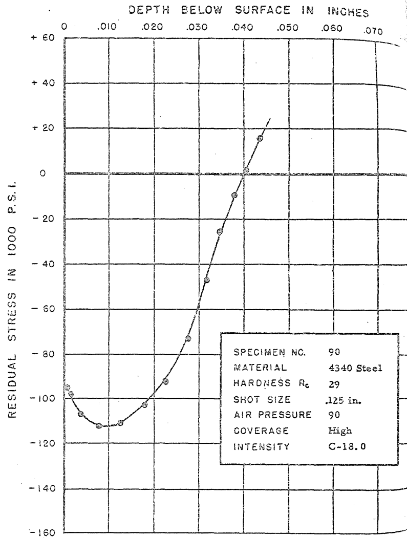
FIGURE 123. RESIDUAL STRESS DISTRIBUTION
