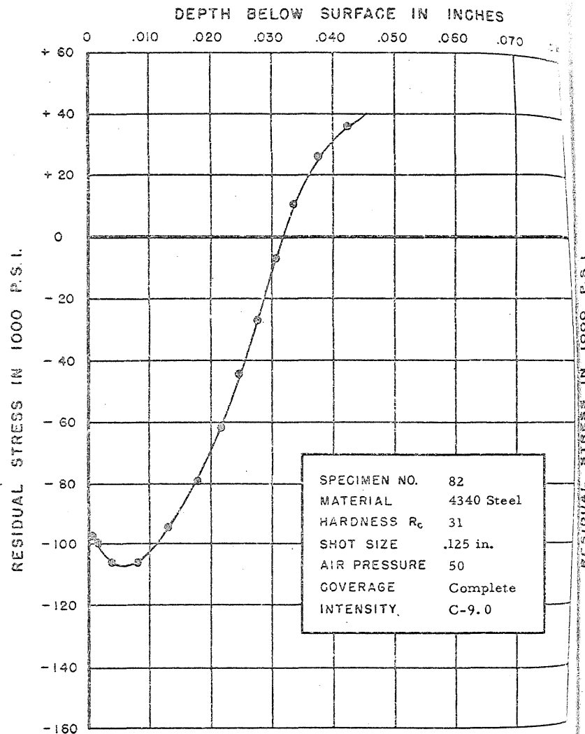
FIGURE 115. RESIDUAL STRESS DISTRIBUTION
