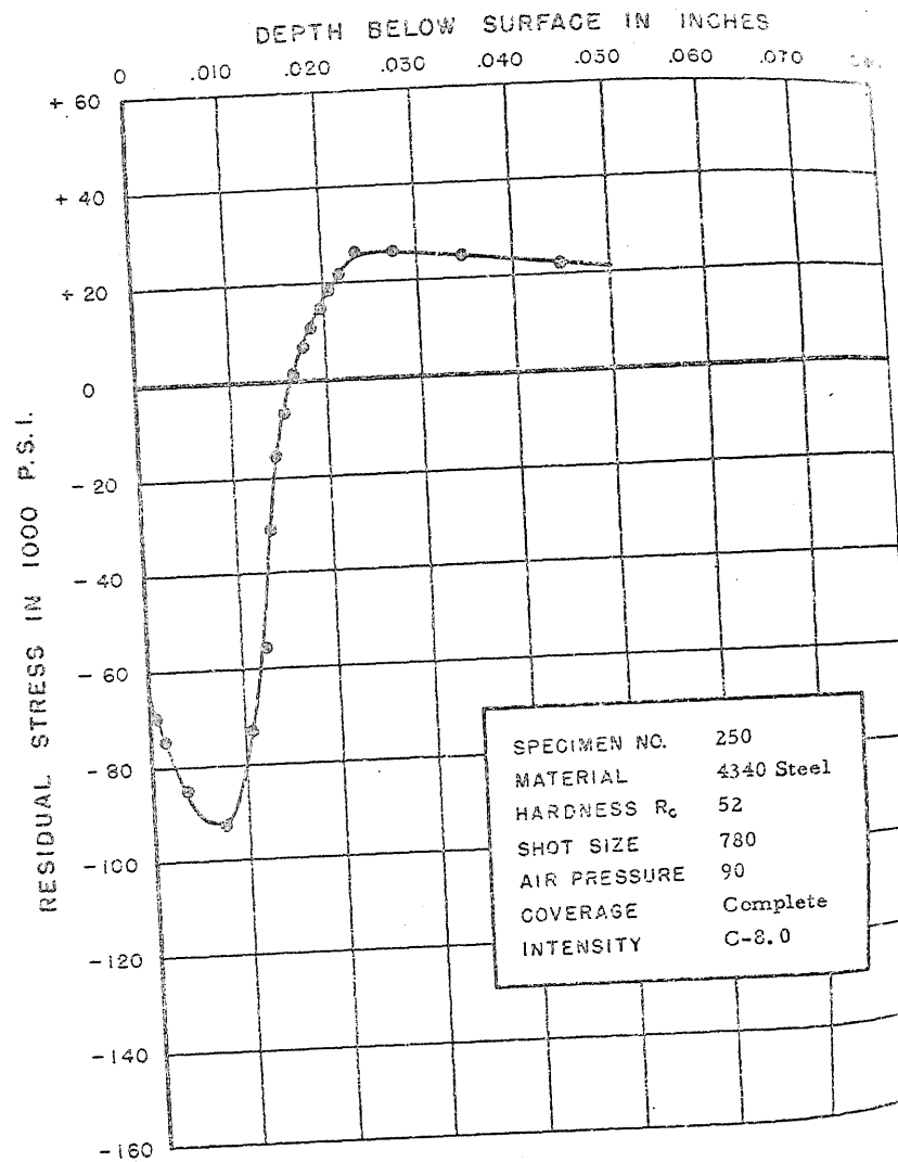
FIGURE 283. RESIDUAL STRESS DISTRIBUTION
