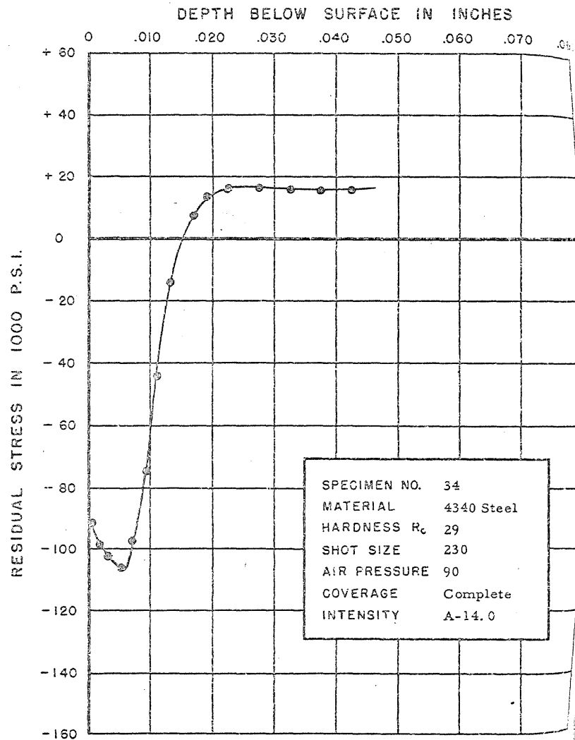
FIGURE 67. RESIDUAL STRESS DISTRIBUTION
