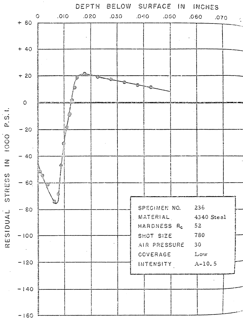
FIGURE 269. RESIDUAL STRESS DISTRIBUTION
