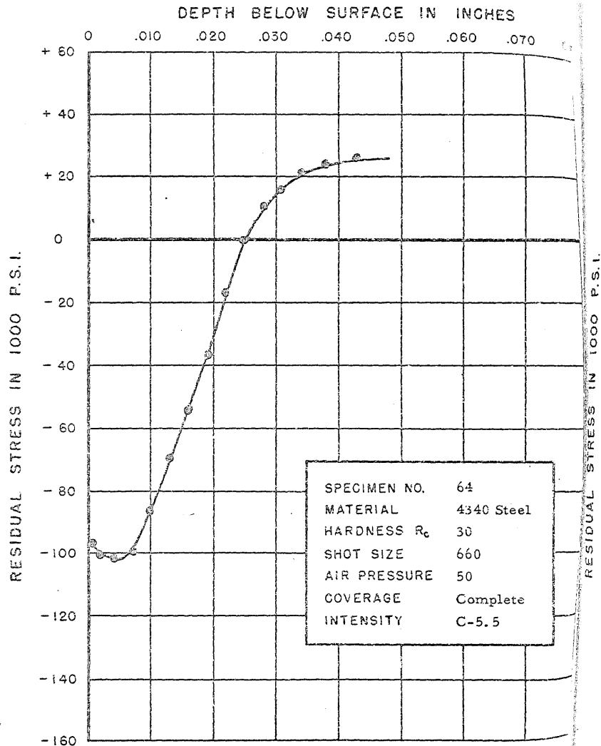
FIGURE 97. RESIDUAL STRESS DISTRIBUTION
