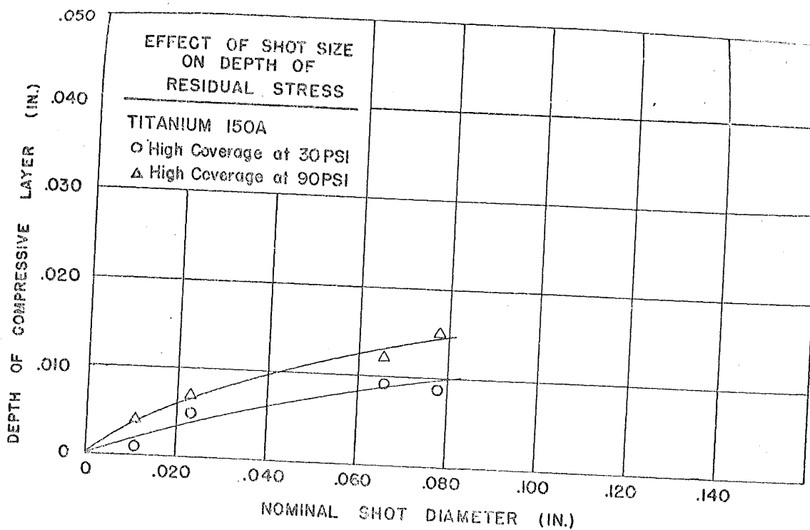
FIGURE 24. EFFECTIVE DEPTH OF PEENING
