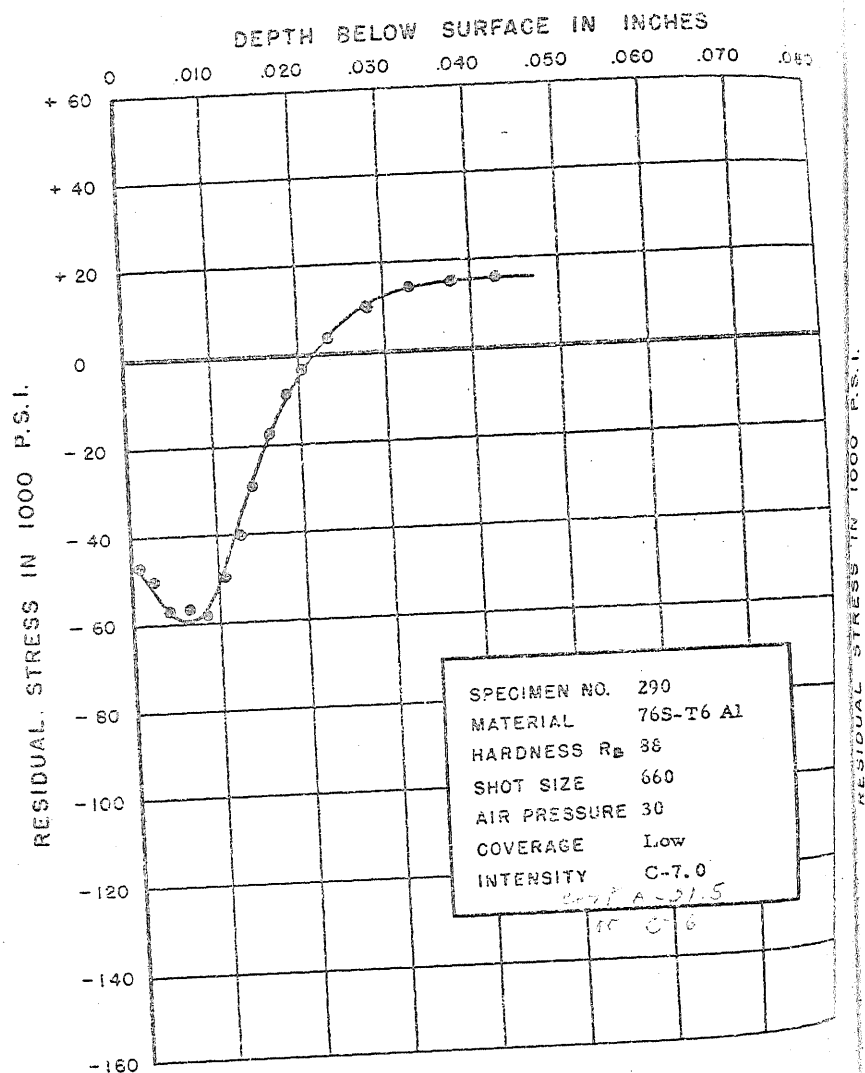
FIGURE 323. RESIDUAL STRESS DISTRIBUTION
