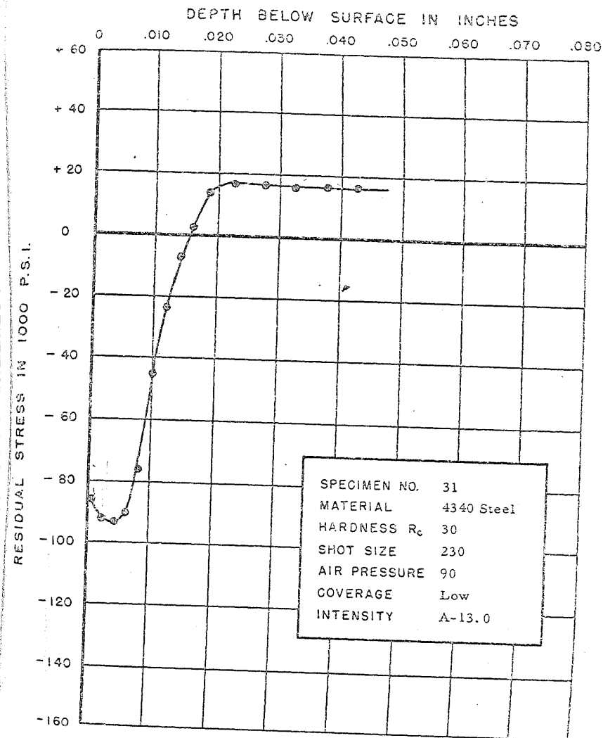
FIGURE 64. RESIDUAL STRESS DISTRIBUTION
