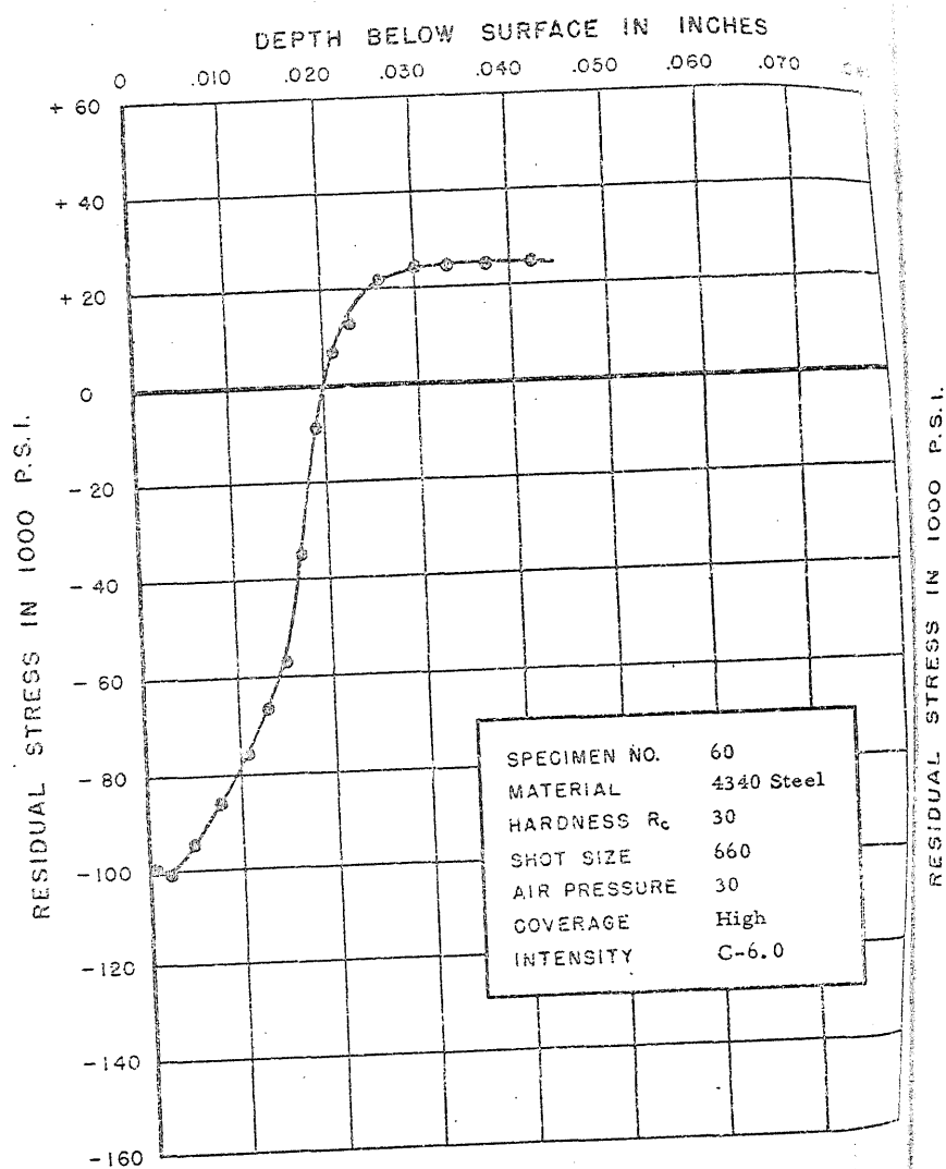
FIGURE 93. RESIDUAL STRESS DISTRIBUTION
