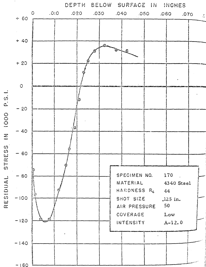
FIGURE 203. RESIDUAL STRESS DISTRIBUTION
