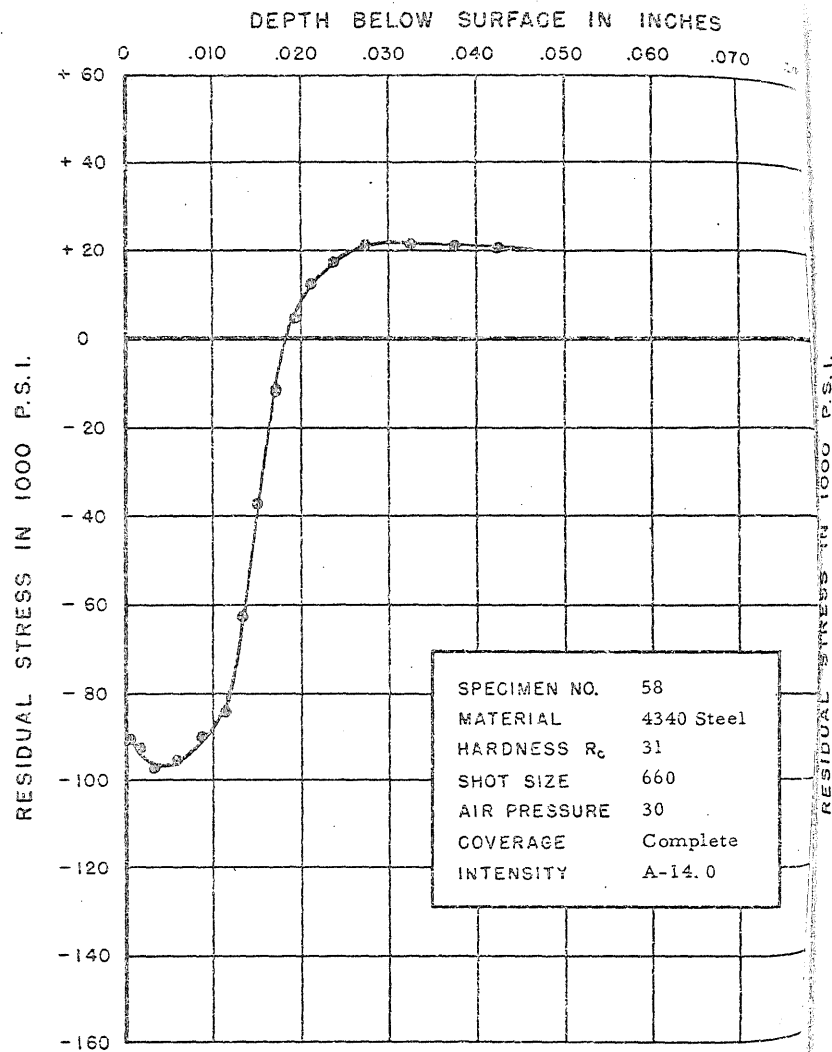
FIGURE 91. RESIDUAL STRESS DISTRIBUTION
