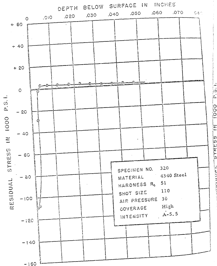
FIGURE 353. RESIDUAL STRESS DISTRIBUTION
