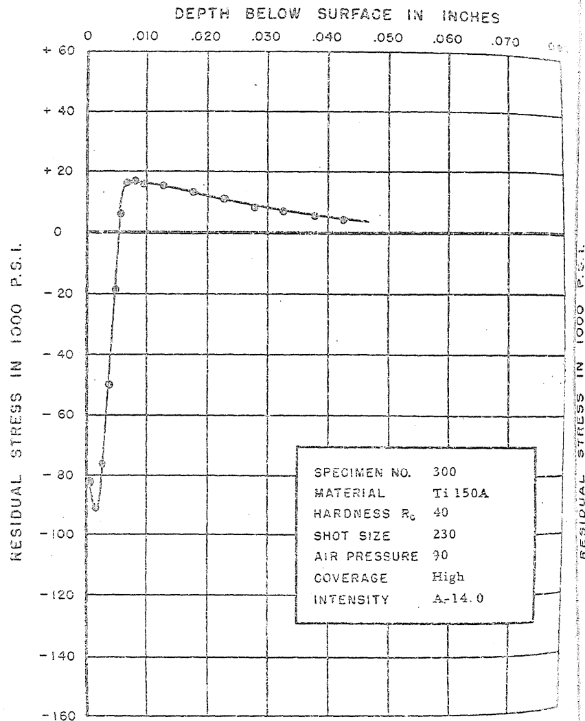
FIGURE 333. RESIDUAL STRESS DISTRIBUTION
