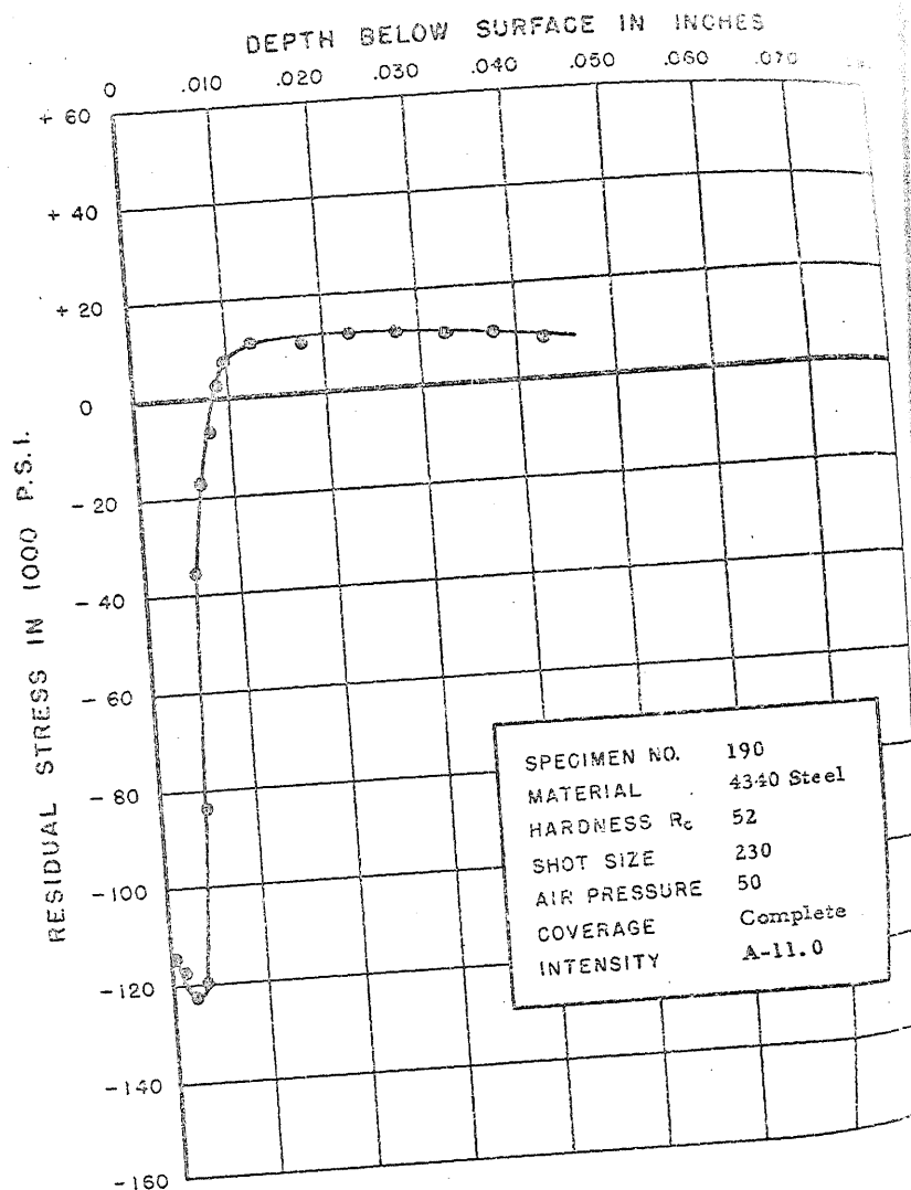
FIGURE 223. RESIDUAL STRESS DISTRIBUTION
