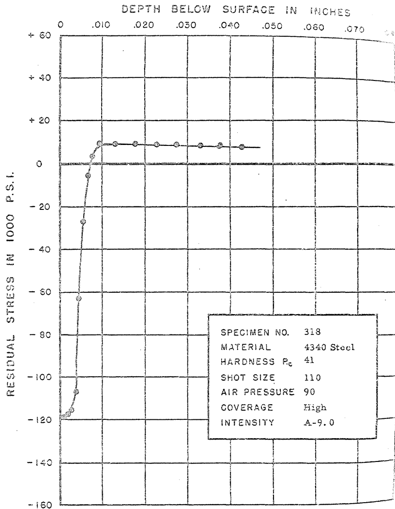
FIGURE 351. RESIDUAL STRESS DISTRIBUTION
