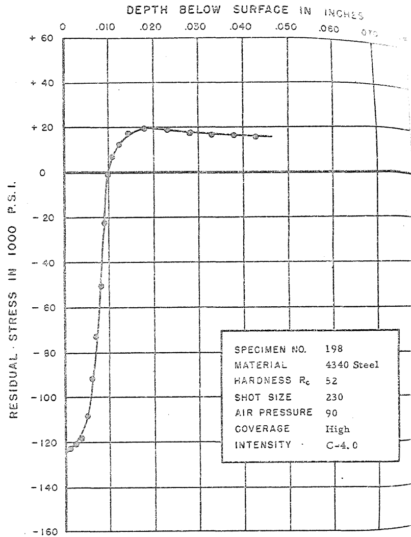
FIGURE 231. RESIDUAL STRESS DISTRIBUTION
