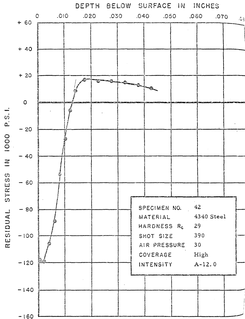
FIGURE 75. RESIDUAL STRESS DISTRIBUTION
