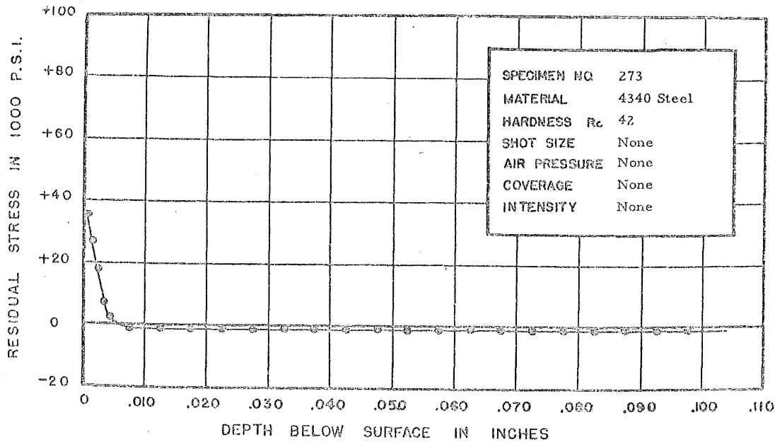
FIGURE 306. RESIDUAL STRESS DISTRIBUTION
