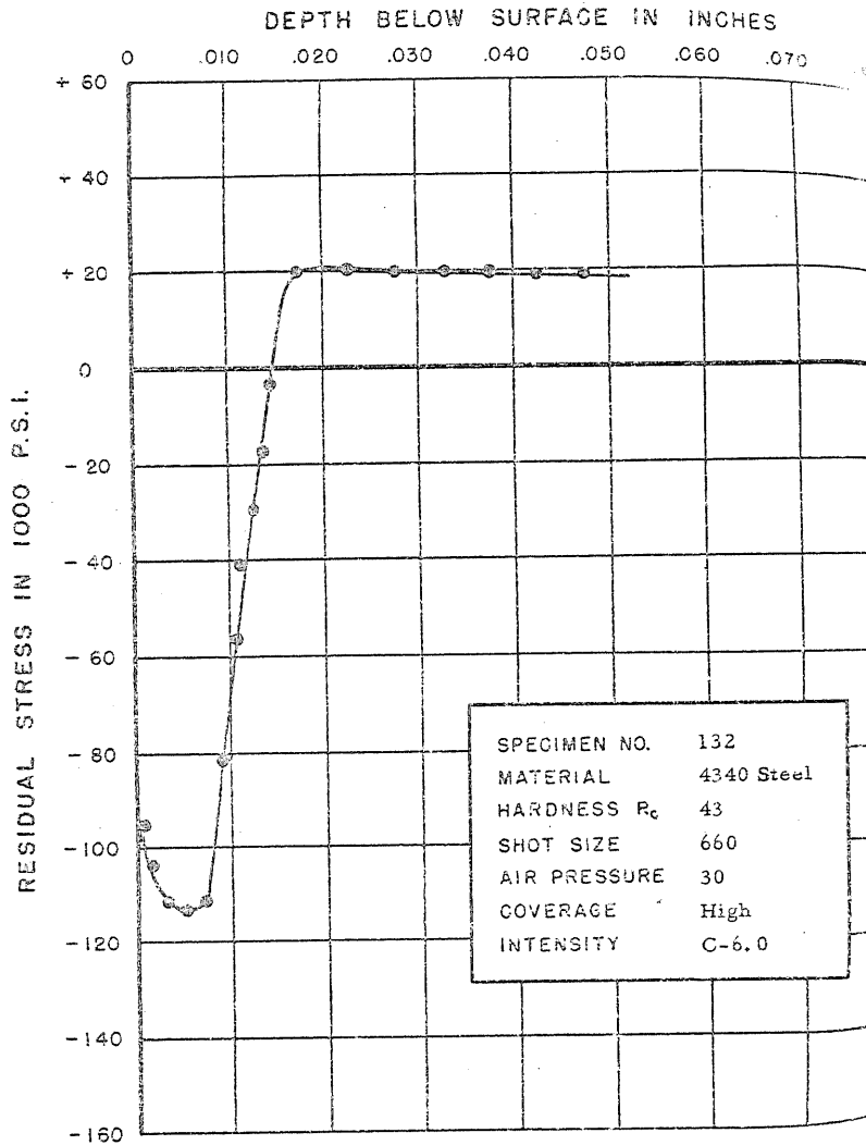
FIGURE 165. RESIDUAL STRESS DISTRIBUTION
