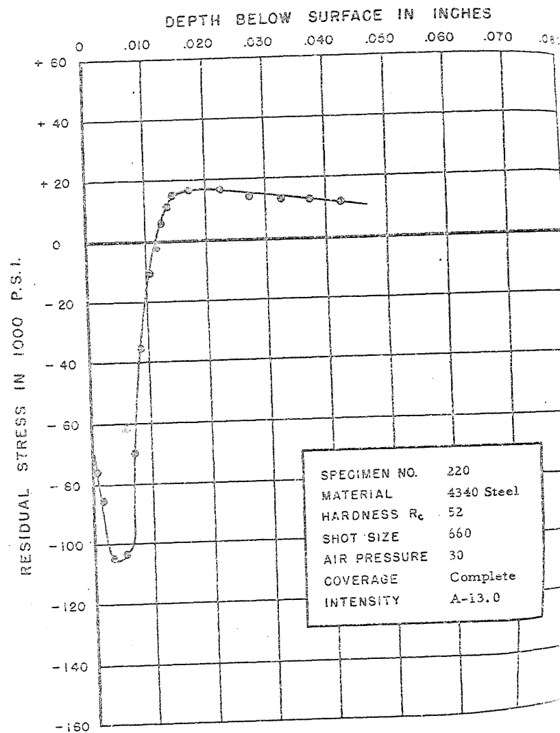
FIGURE 253. RESIDUAL STRESS DISTRIBUTION
