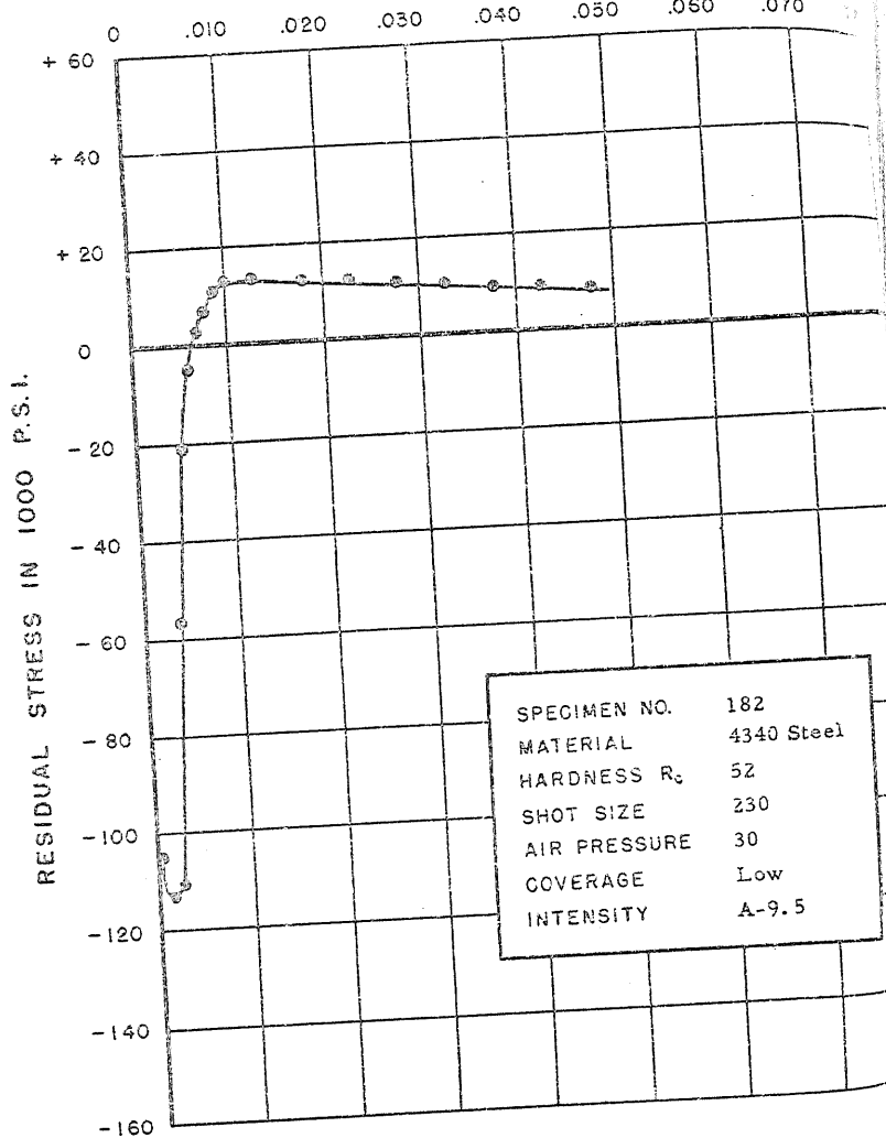
FIGURE 215. RESIDUAL STRESS DISTRIBUTION
