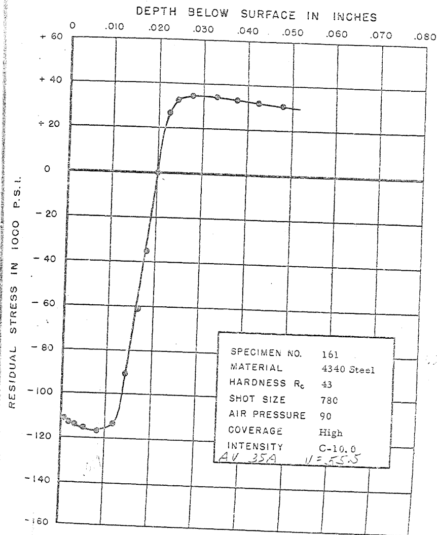
FIGURE 194. RESIDUAL STRESS DISTRIBUTION
