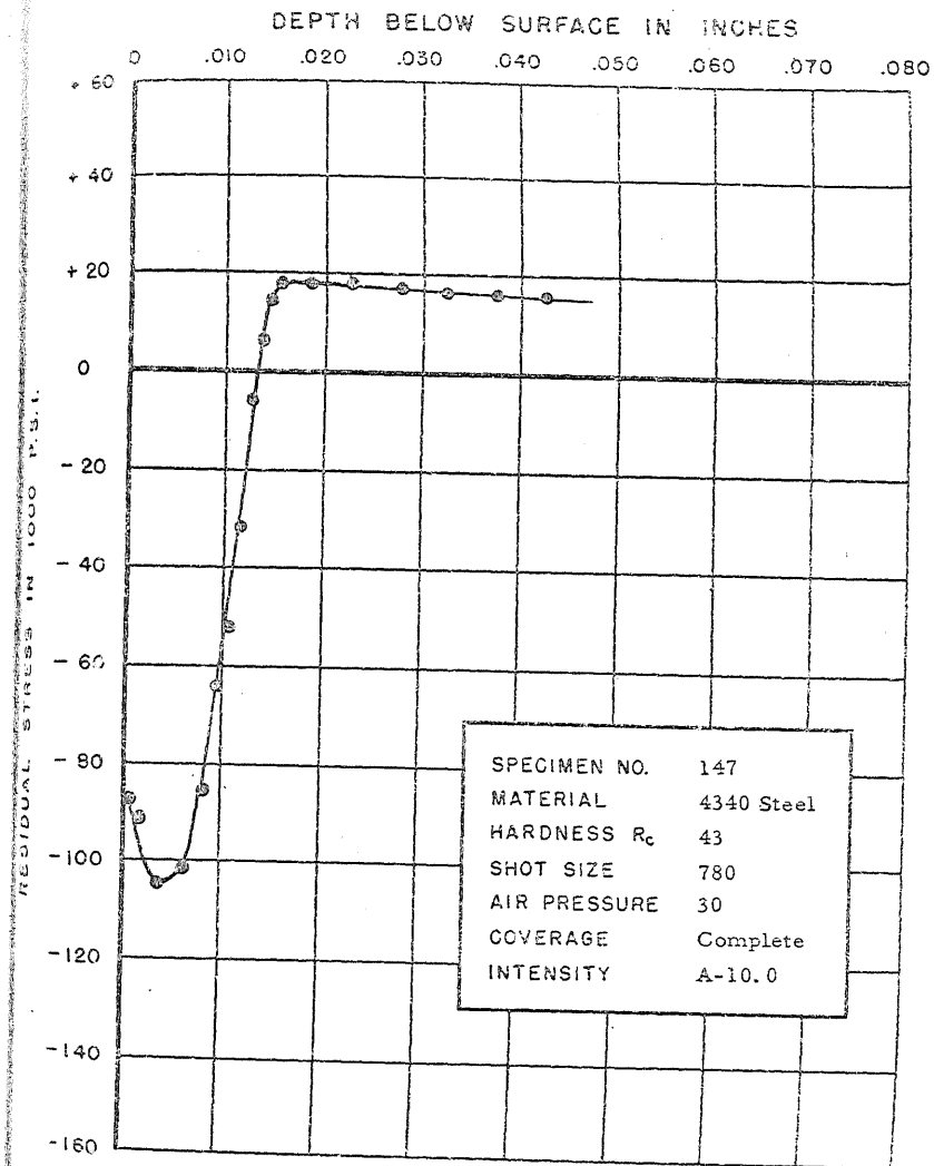
FIGURE 180. RESIDUAL STRESS DISTRIBUTION
