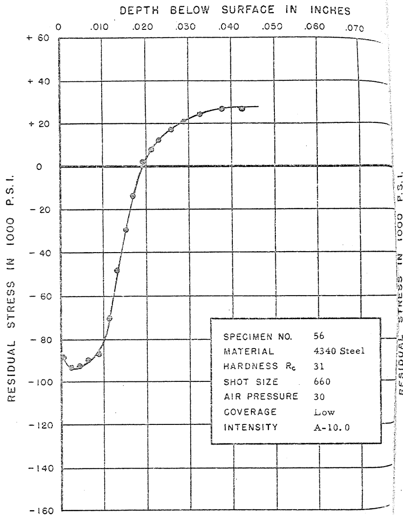
FIGURE 89. RESIDUAL STRESS DISTRIBUTION
