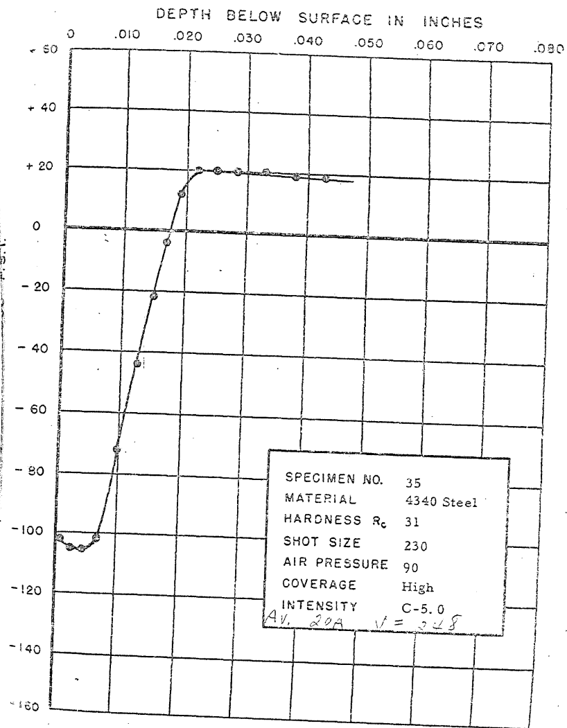
FIGURE 68. RESIDUAL STRESS DISTRIBUTION
