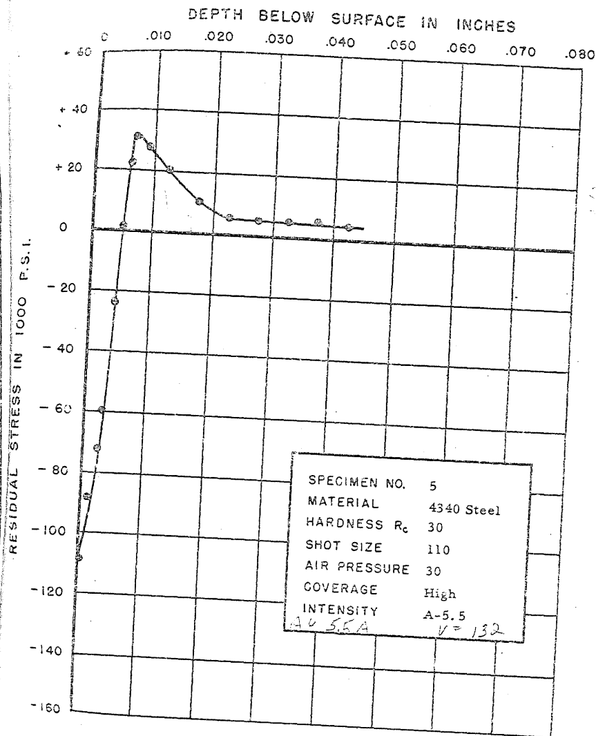
FIGURE 38. RESIDUAL STRESS DISTRIBUTION
