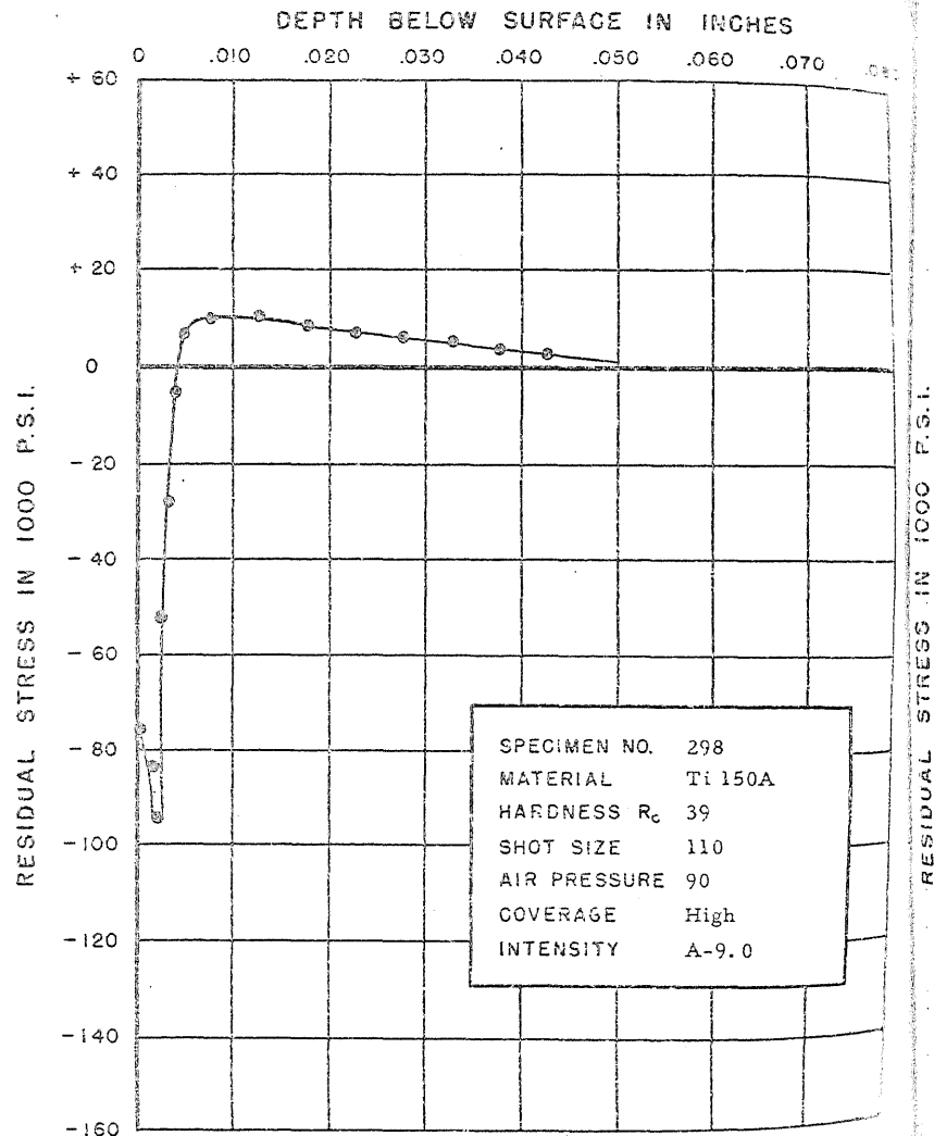
FIGURE 331. RESIDUAL STRESS DISTRIBUTION
