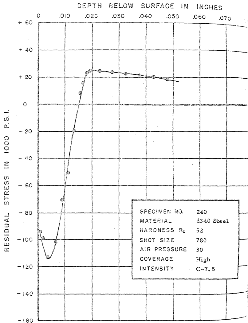
FIGURE 273. RESIDUAL STRESS DISTRIBUTION
