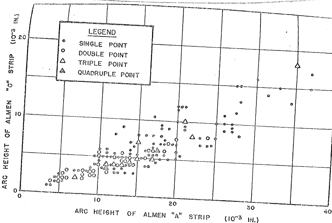
FIGURE 27. ARC HEIGHT DISTRIBUTION OF ALMEN "A" & "C" STRIPS
