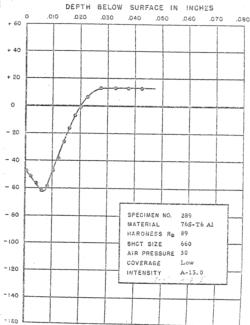
FIGURE 322. RESIDUAL STRESS DISTRIBUTION
