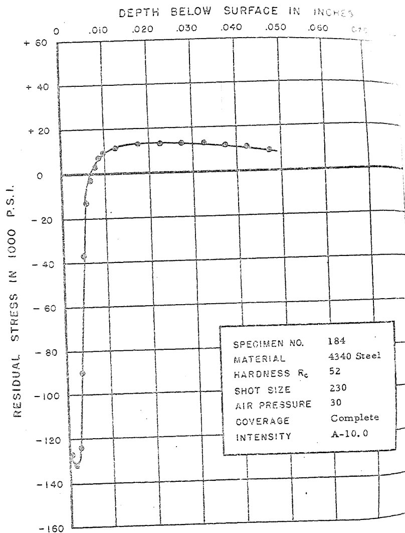
FIGURE 217. RESIDUAL STRESS DISTRIBUTION
