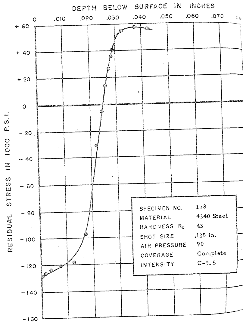
FIGURE 211. RESIDUAL STRESS DISTRIBUTION
