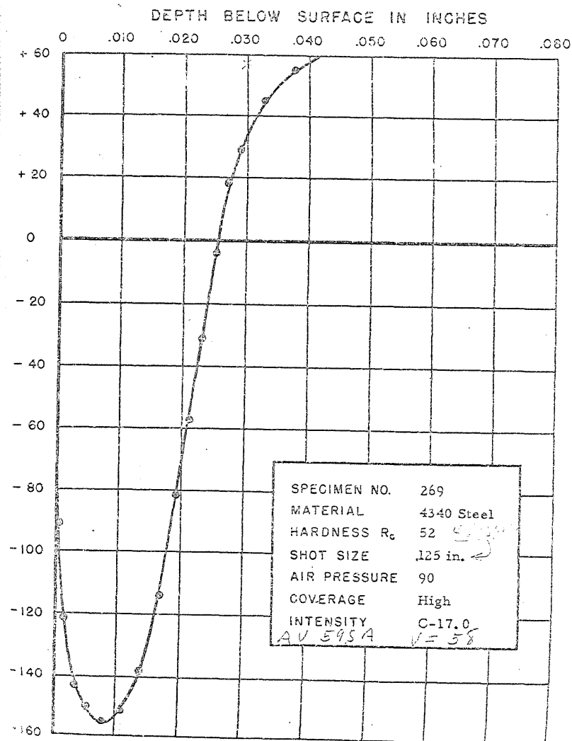
FIGURE 302. RESIDUAL STRESS DISTRIBUTION
