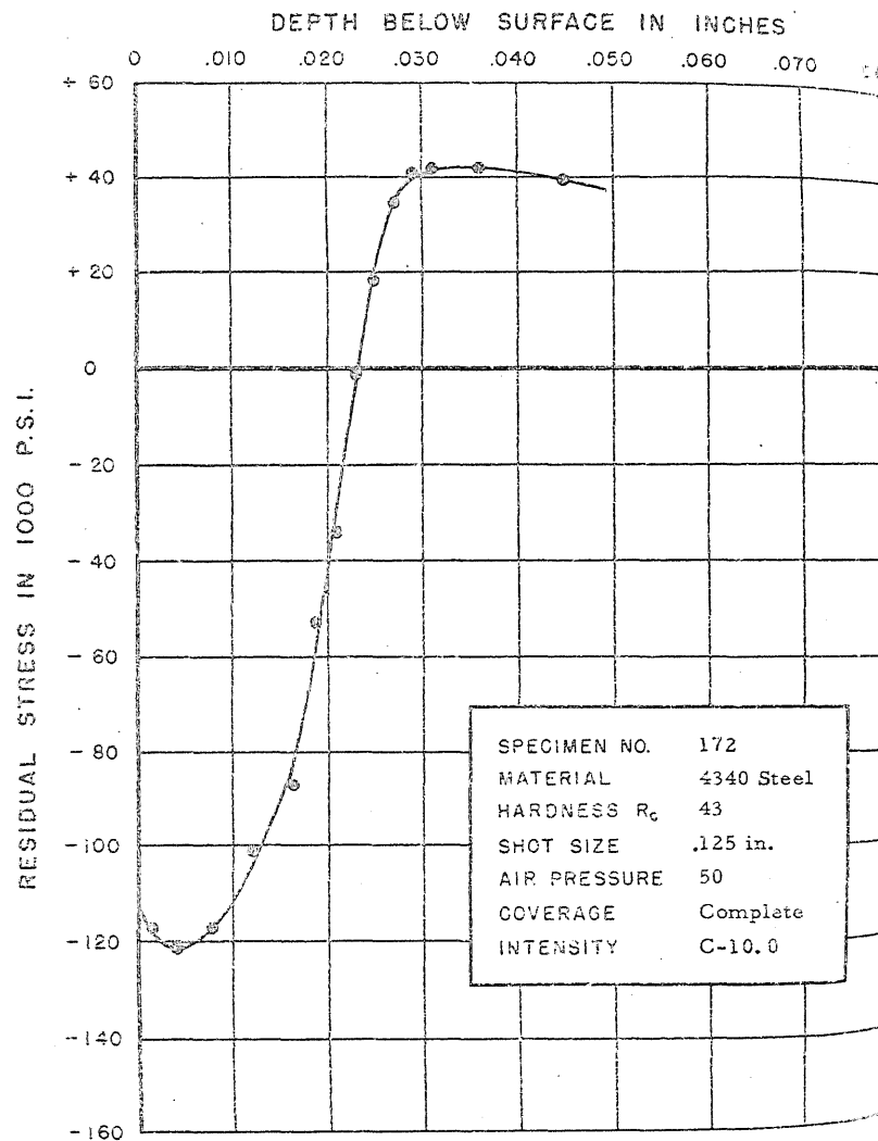
FIGURE 205. RESIDUAL STRESS DISTRIBUTION
