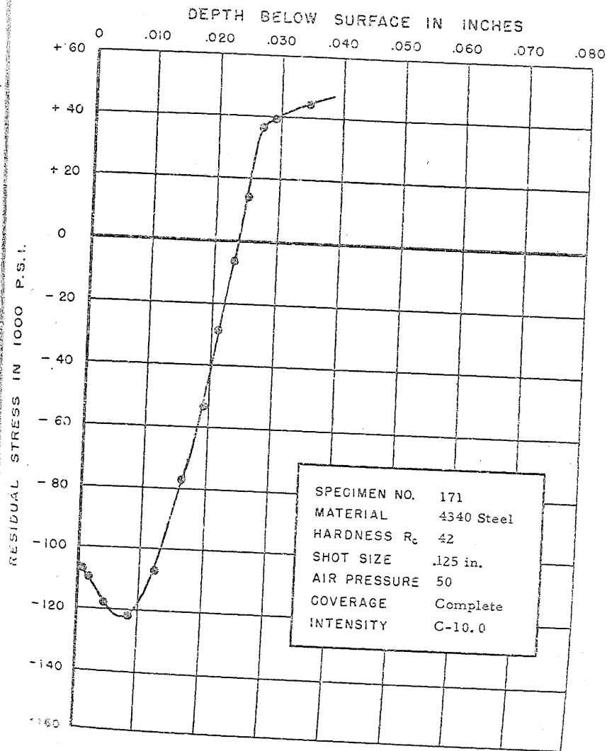
FIGURE 204. RESIDUAL STRESS DISTRIBUTION
