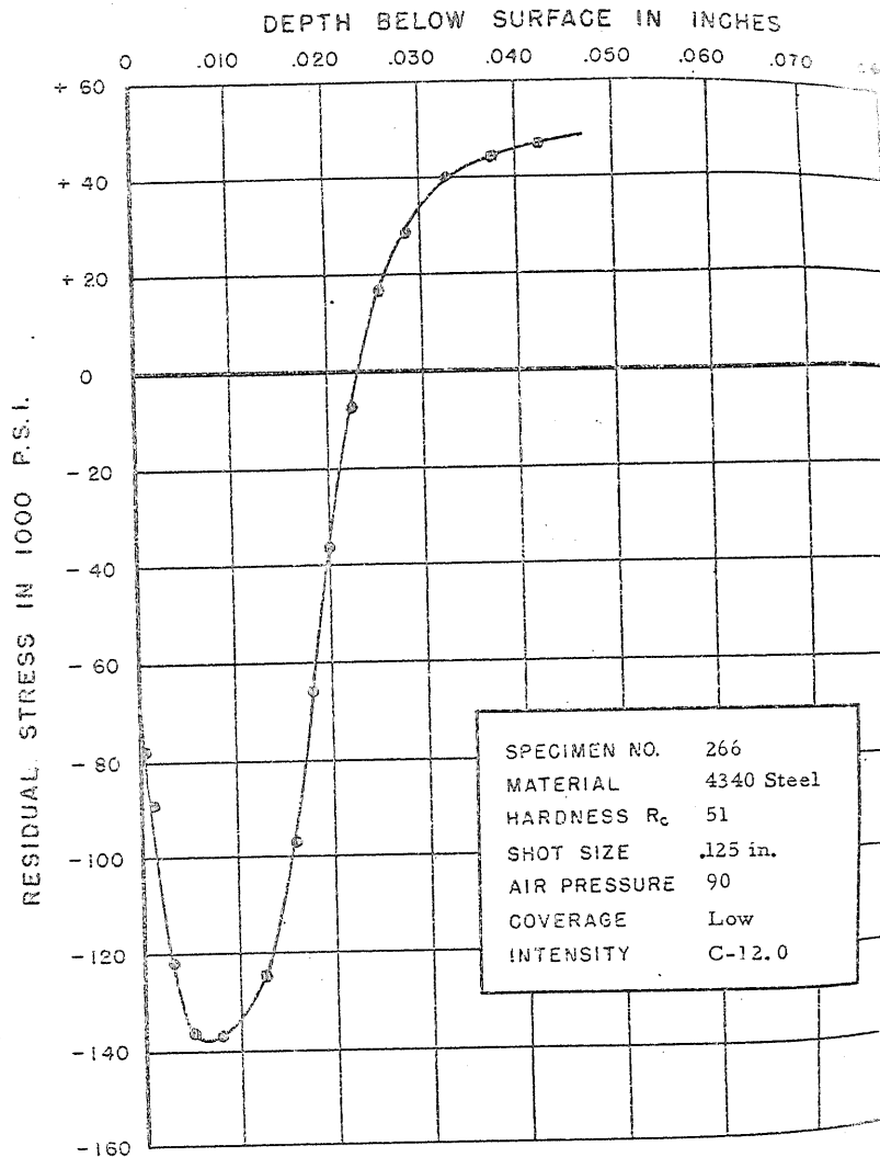
FIGURE 299. RESIDUAL STRESS DISTRIBUTION
