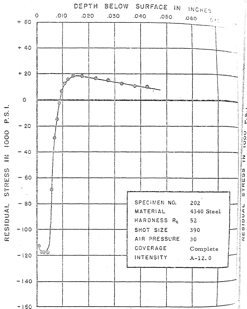
FIGURE 235. RESIDUAL STRESS DISTRIBUTION
