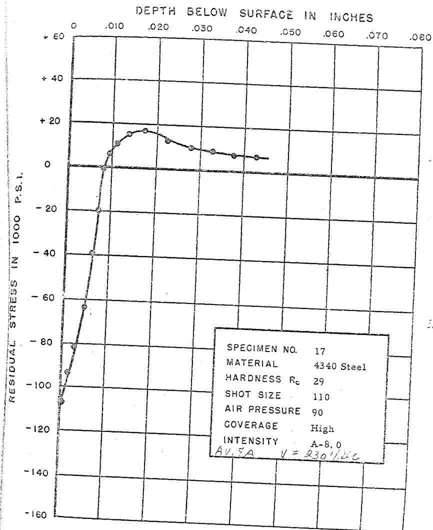
FIGURE 50. RESIDUAL STRESS DISTRIBUTION
