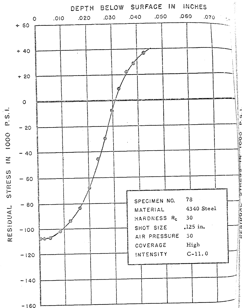
FIGURE III. RESIDUAL STRESS DISTRIBUTION
