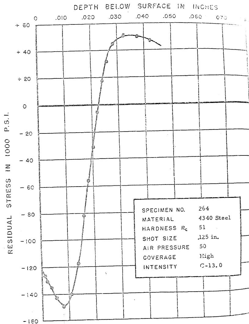
FIGURE 297. RESIDUAL STRESS DISTRIBUTION
