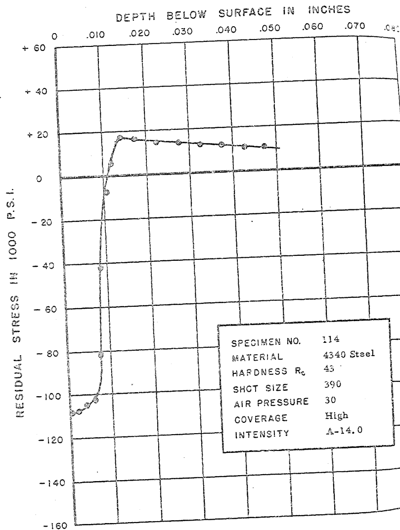
FIGURE 147. RESIDUAL STRESS DISTRIBUTION
