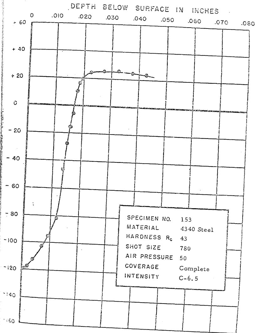
FIGURE 186. RESIDUAL STRESS DISTRIBUTION
