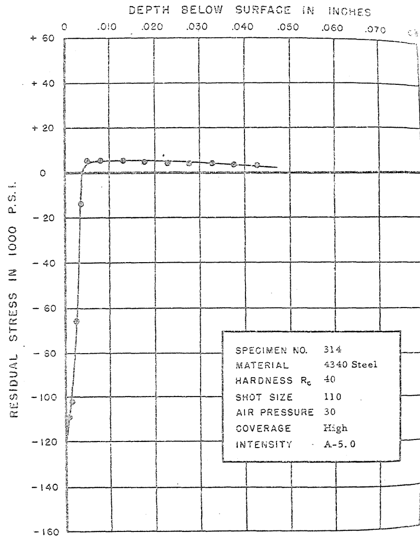
FIGURE 347. RESIDUAL STRESS DISTRIBUTION
