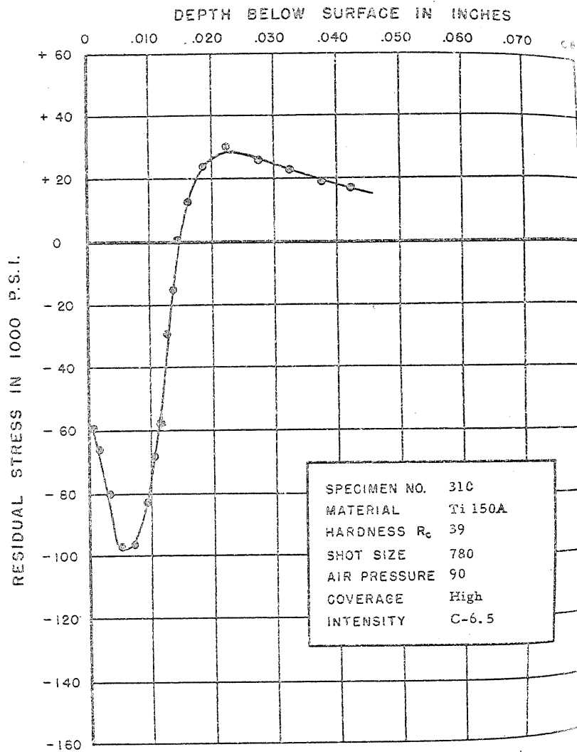
FIGURE 343. RESIDUAL STRESS DISTRIBUTION
