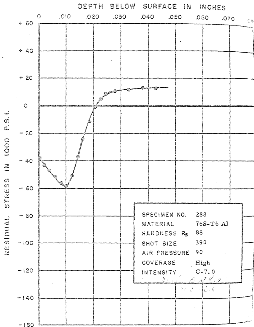
FIGURE 321. RESIDUAL STRESS DISTRIBUTION
