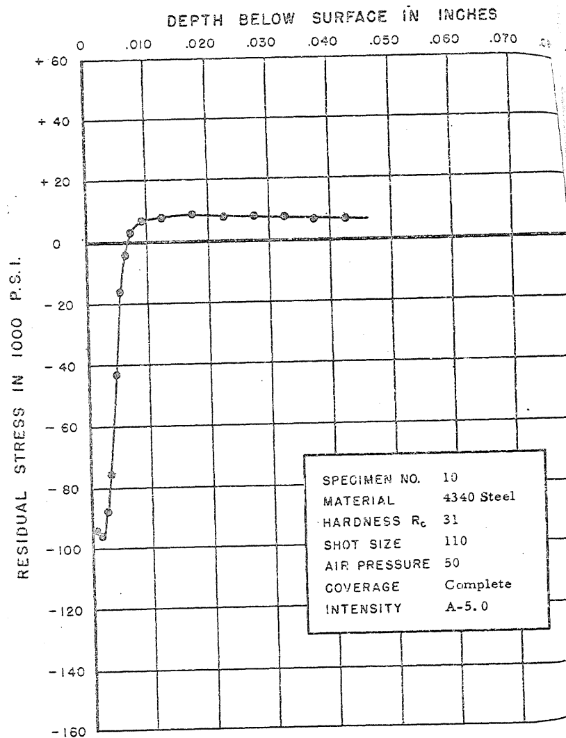
FIGURE 43. RESIDUAL STRESS DISTRIBUTION
