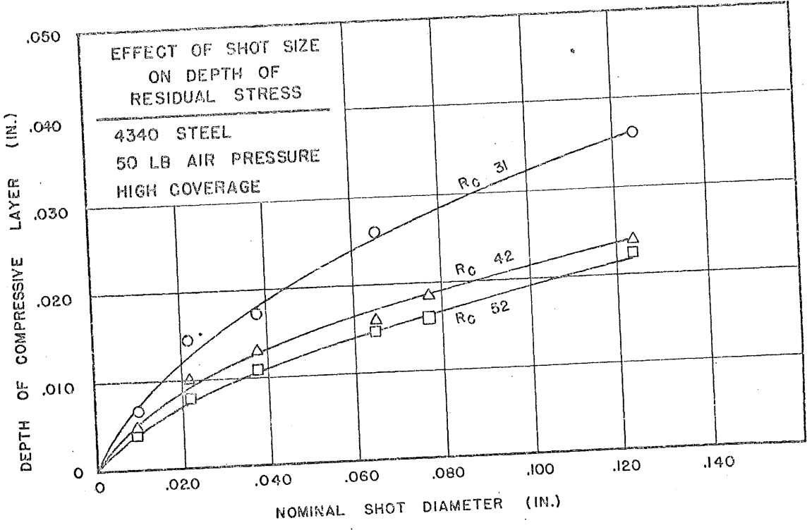
FIGURE 19. EFFECTIVE DEPTH OF PEENING
