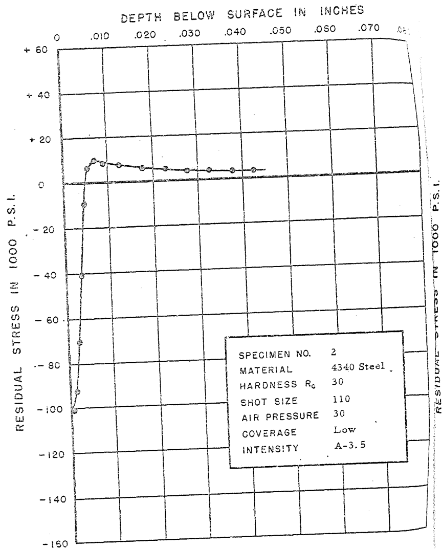
FIGURE 35. RESIDUAL STRESS DISTRIBUTION
