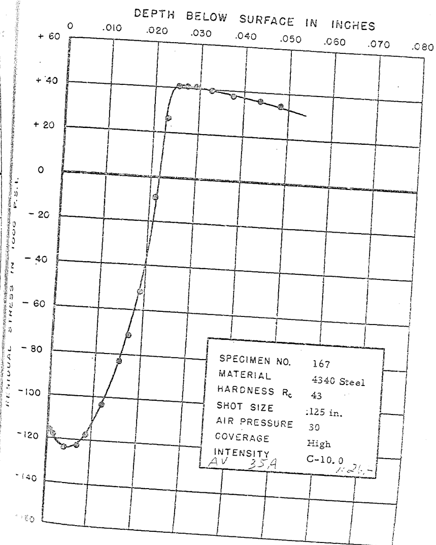
FIGURE 200. RESIDUAL STRESS DISTRIBUTION
