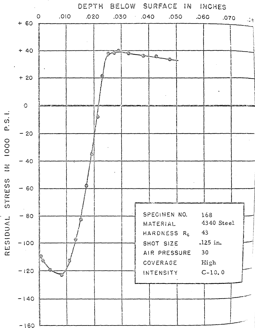
FIGURE 201. RESIDUAL STRESS DISTRIBUTION
