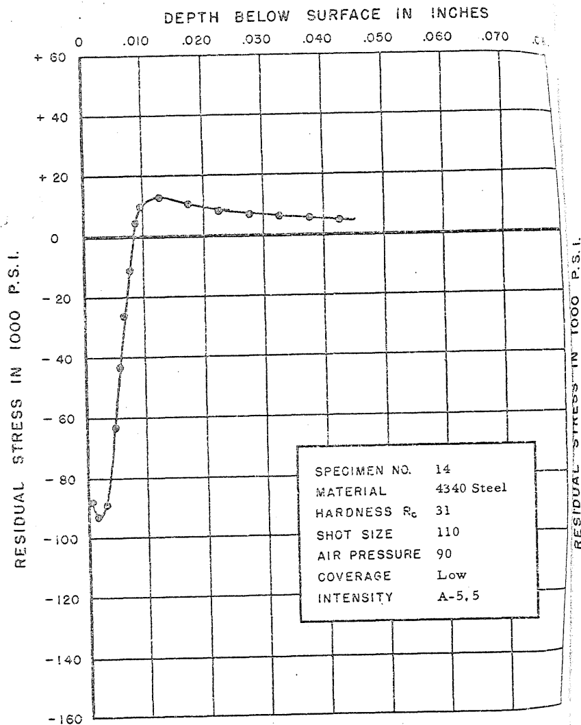
FIGURE 47. RESIDUAL STRESS DISTRIBUTION
