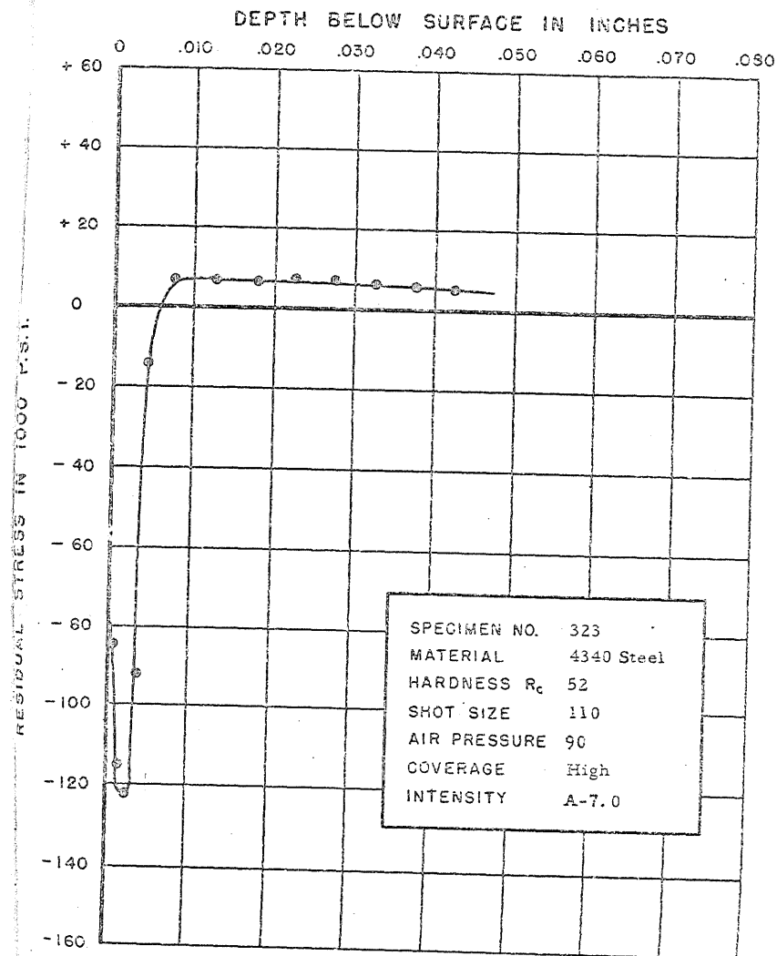
FIGURE 356. RESIDUAL STRESS DISTRIBUTION
