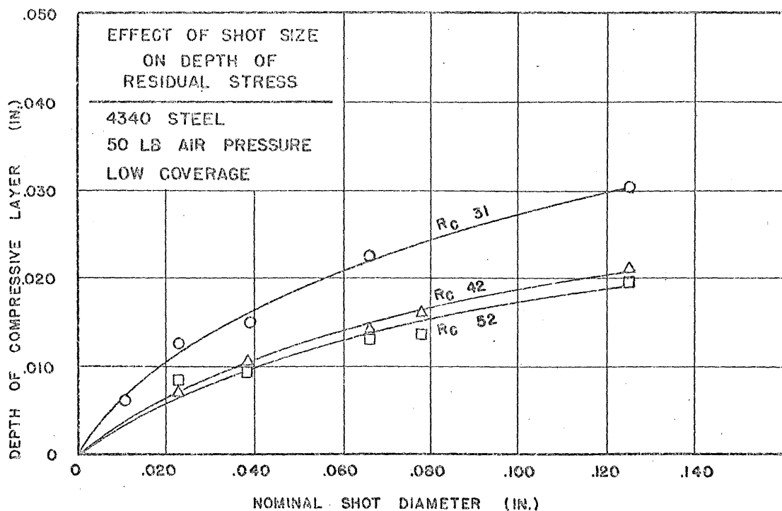
FIGURE 17. EFFECTIVE DEPTH OF PEENING
