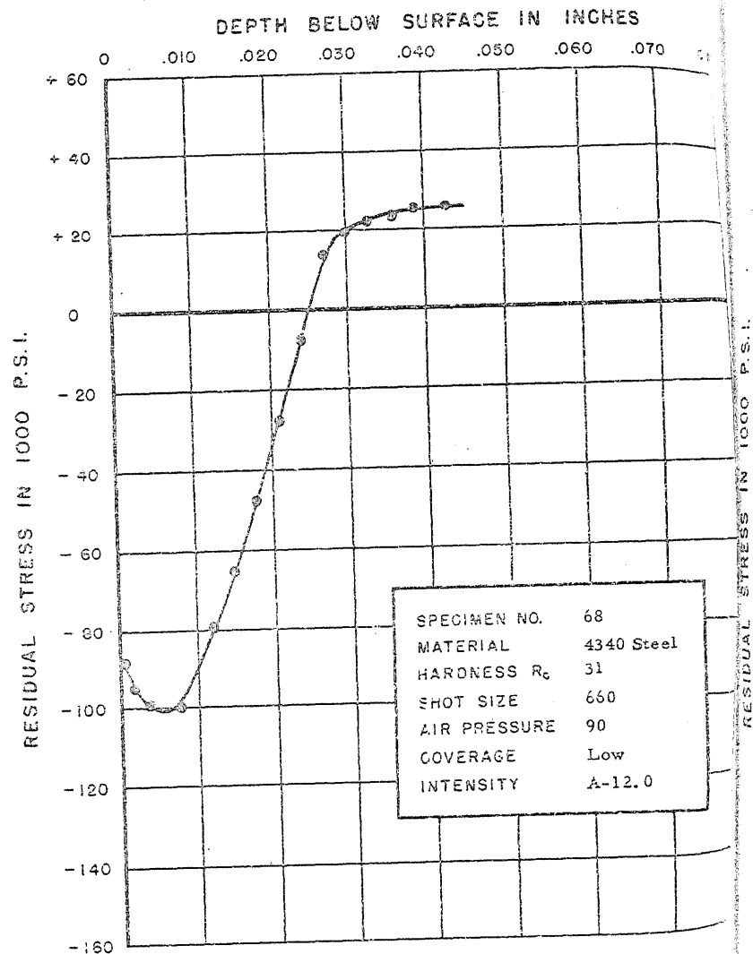
FIGURE 101. RESIDUAL STRESS DISTRIBUTION
