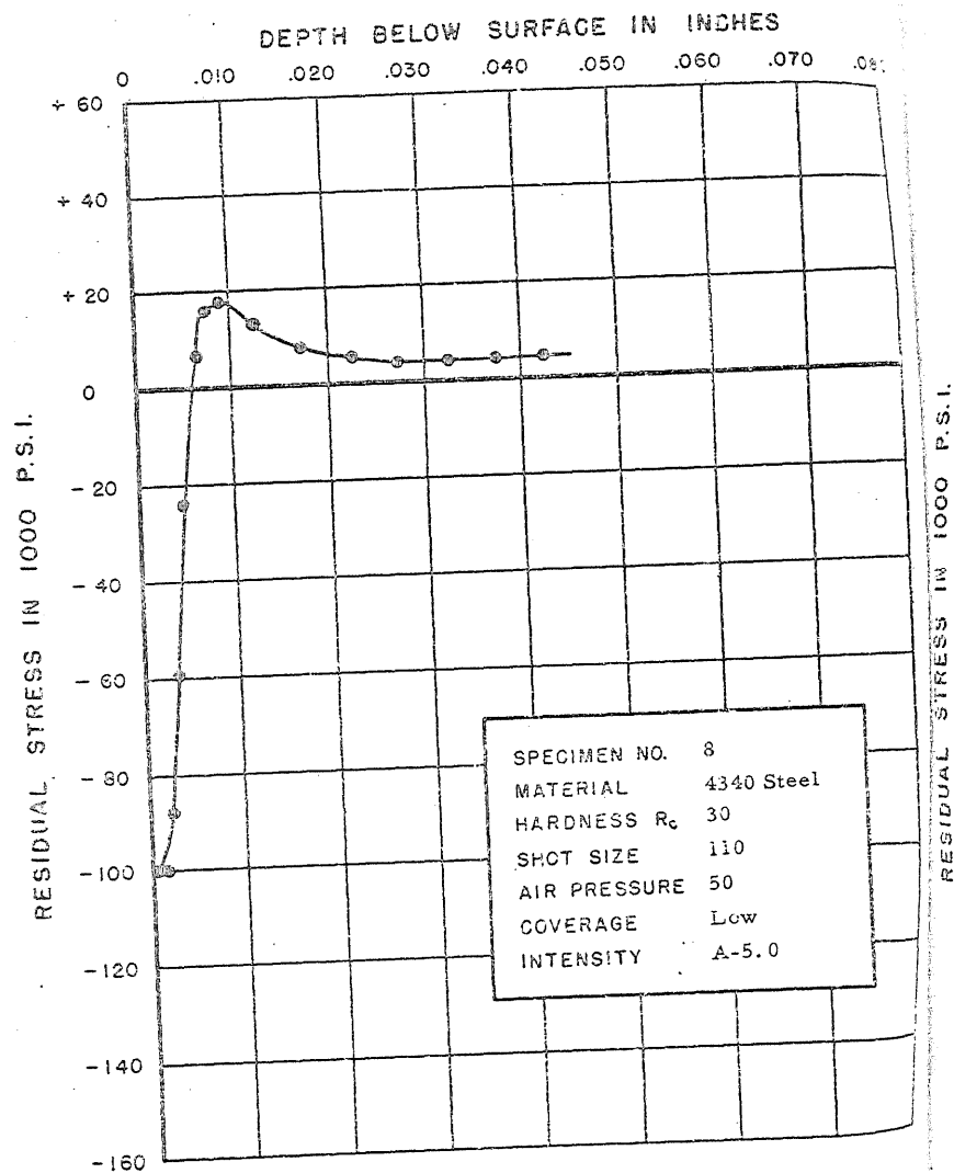
FIGURE 41. RESIDUAL STRESS DISTRIBUTION
