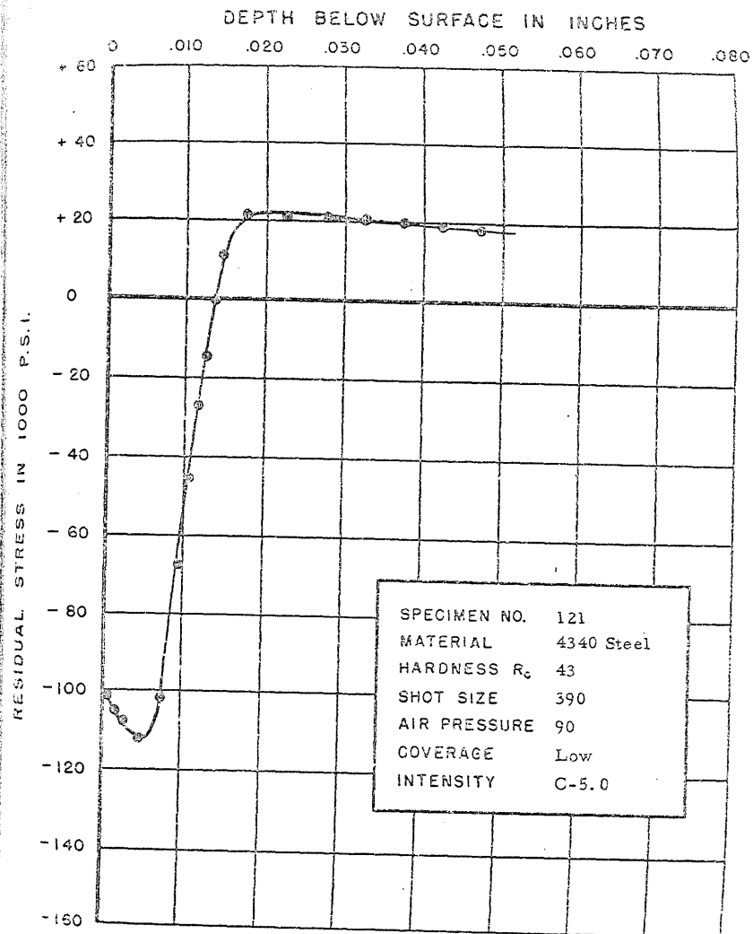
FIGURE 154. RESIDUAL STRESS DISTRIBUTION
