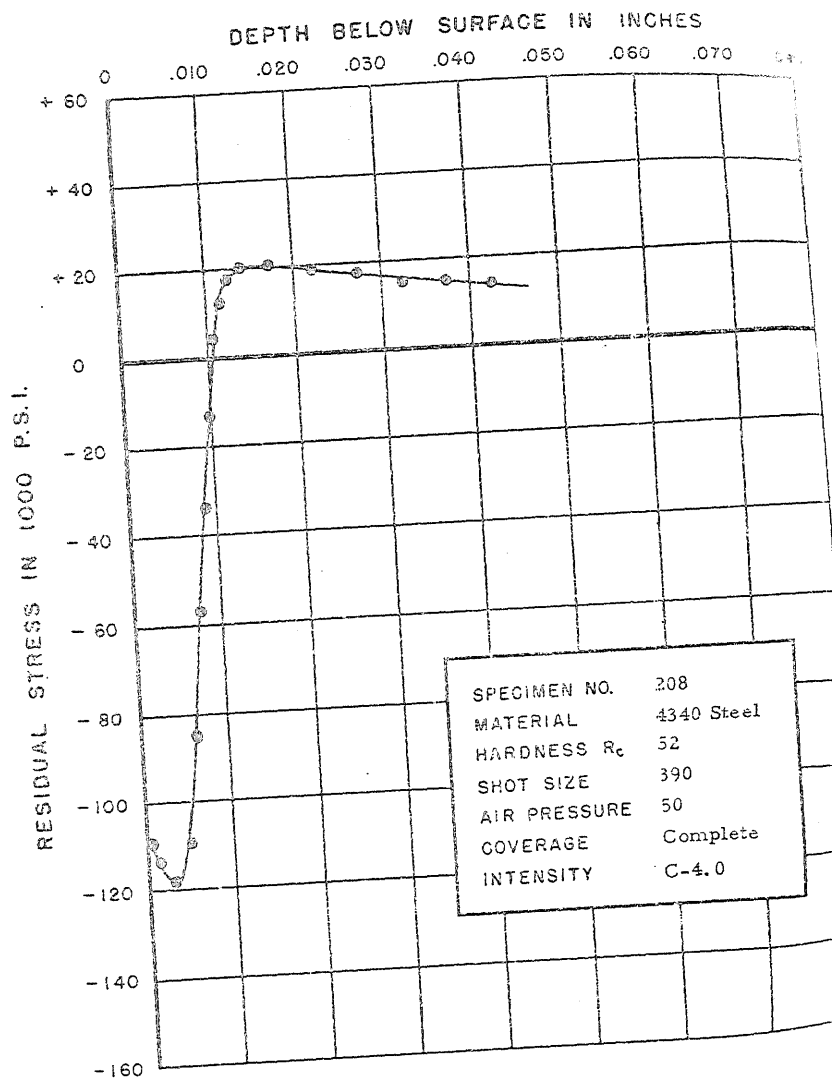
FIGURE 241. RESIDUAL STRESS DISTRIBUTION
