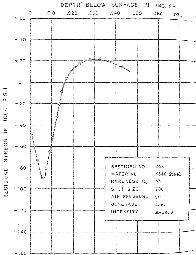
FIGURE 281. RESIDUAL STRESS DISTRIBUTION
