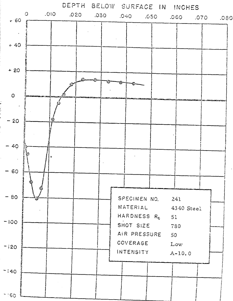
FIGURE 274. RESIDUAL STRESS DISTRIBUTION
