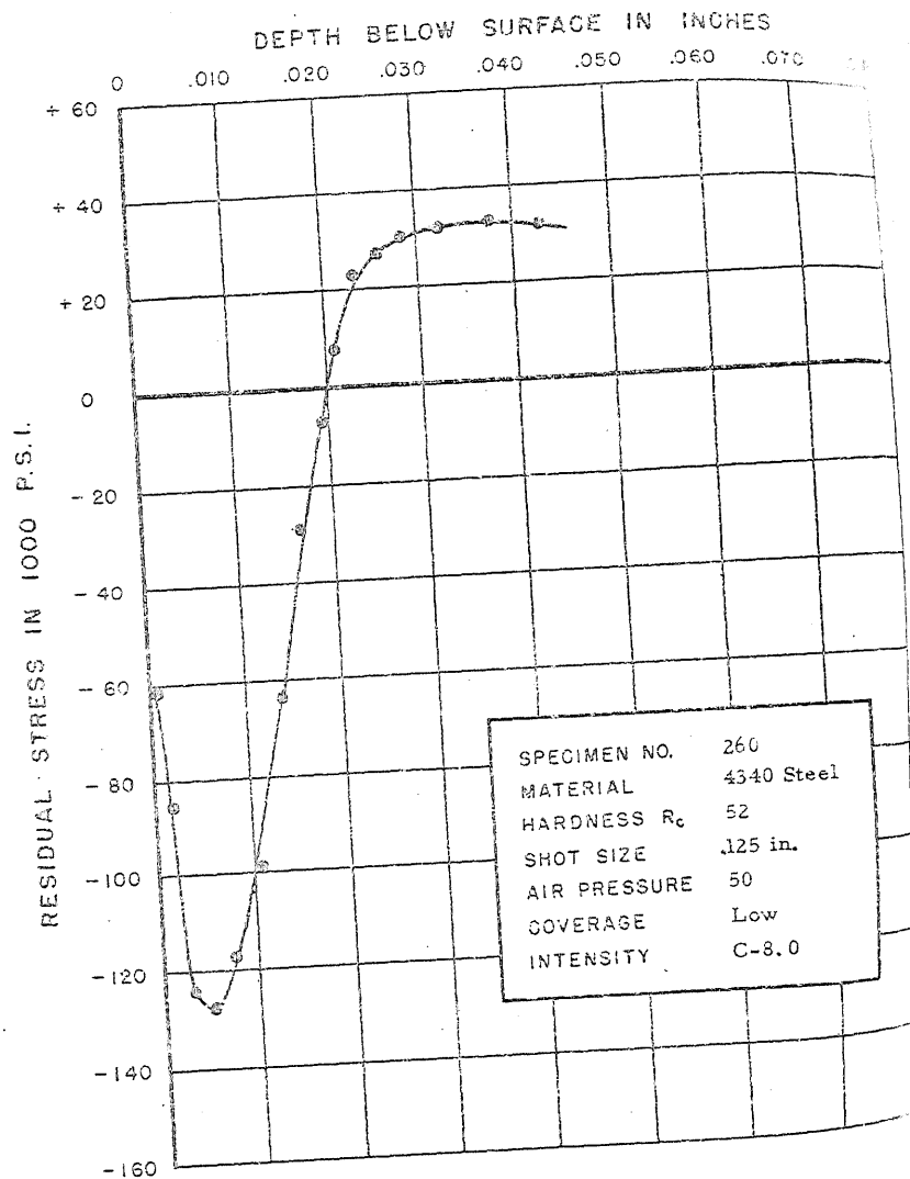
FIGURE 293. RESIDUAL STRESS DISTRIBUTION
