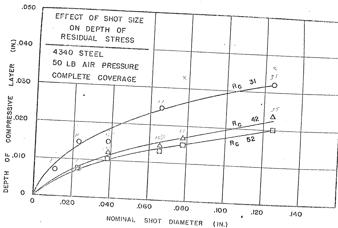
FIGURE 18. EFFECTIVE DEPTH OF PEENING
