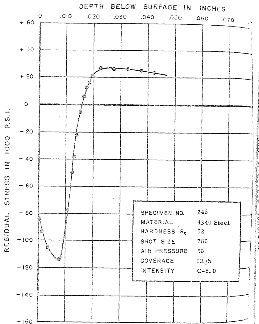
FIGURE 279. RESIDUAL STRESS DISTRIBUTION
