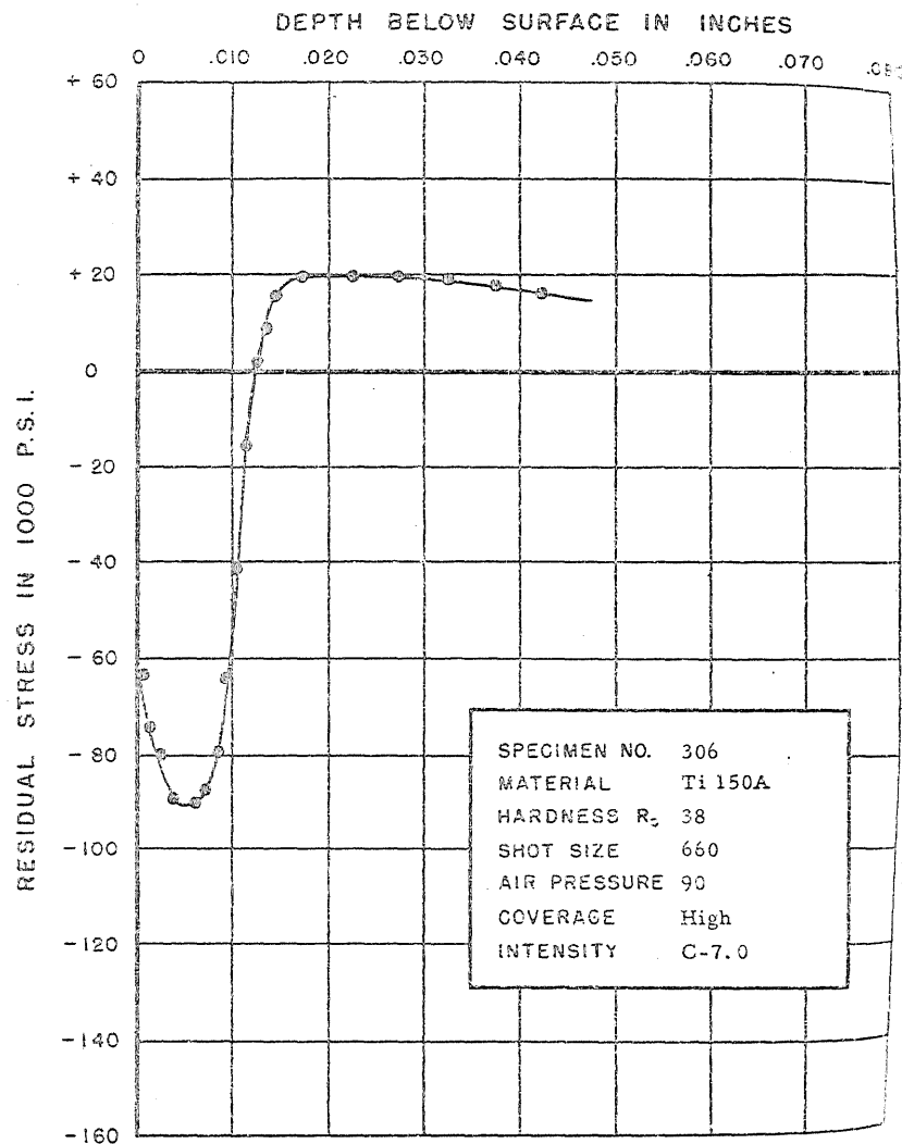
FIGURE 339. RESIDUAL STRESS DISTRIBUTION
