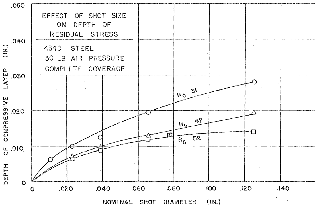
FIGURE 15. EFFECTIVE DEPTH OF PEENING
