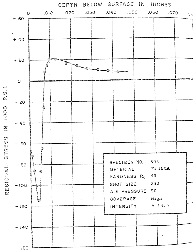
FIGURE 335. RESIDUAL STRESS DISTRIBUTION
