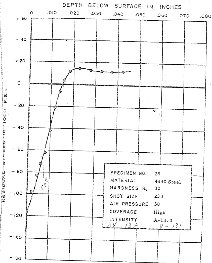
FIGURE 62. RESIDUAL STRESS DISTRIBUTION
