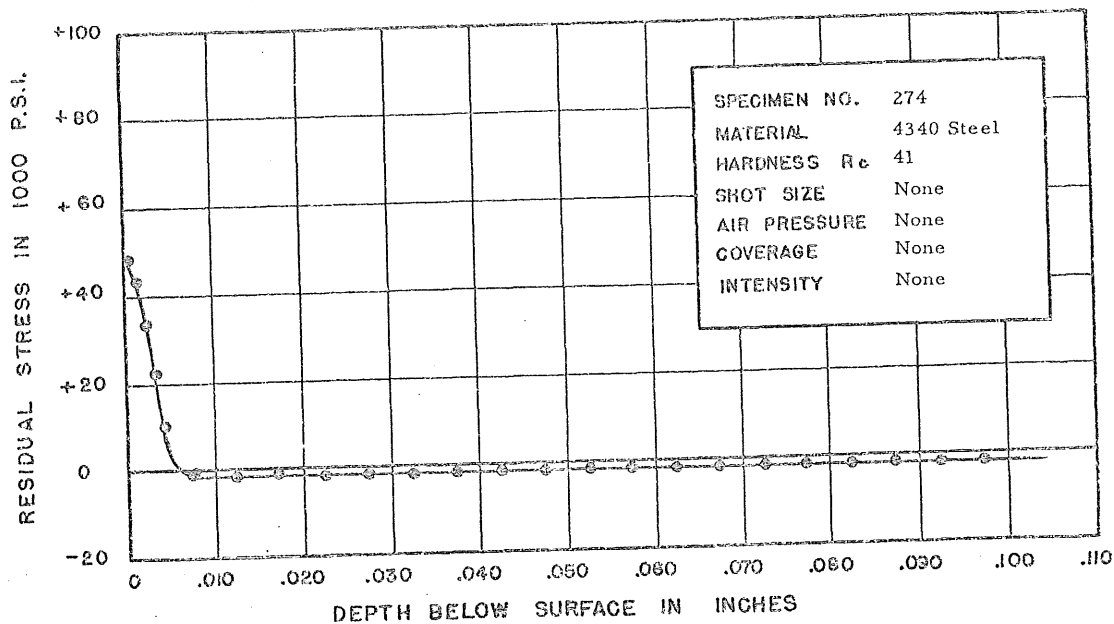
FIGURE 307. RESIDUAL STRESS DISTRIBUTION
