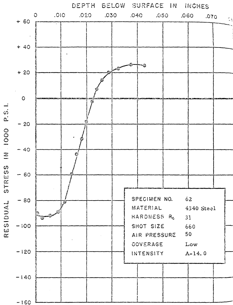
FIGURE 95. RESIDUAL STRESS DISTRIBUTION
