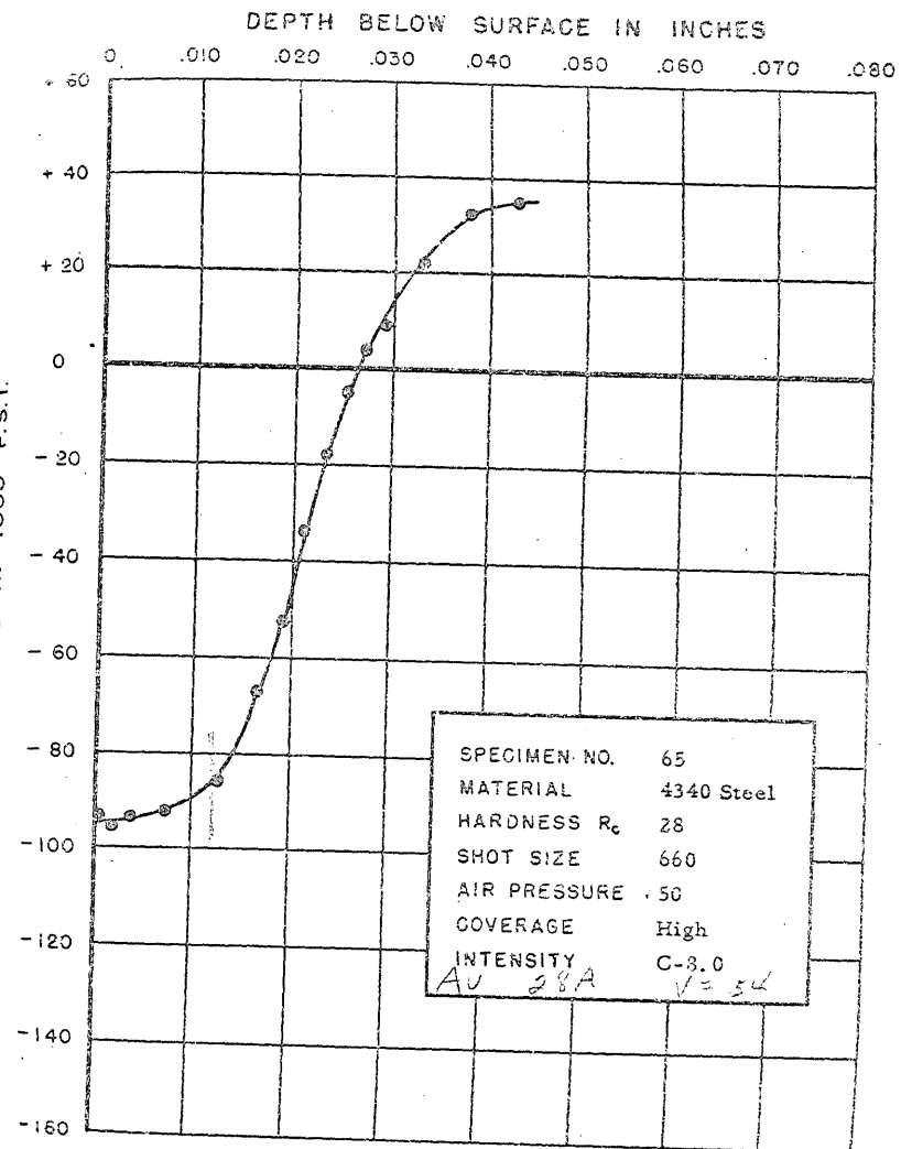
FIGURE 98. RESIDUAL STRESS DISTRIBUTION
