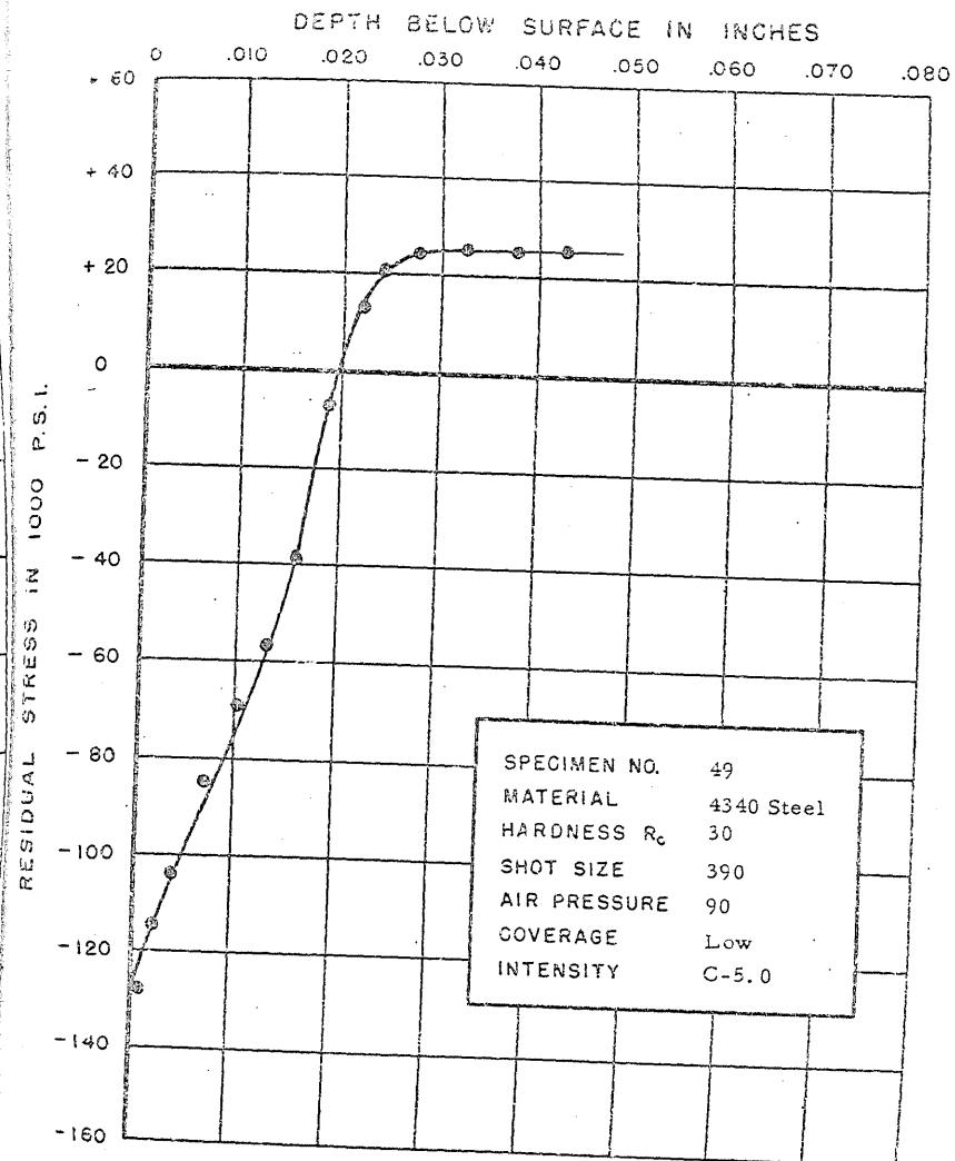
FIGURE 82. RESIDUAL STRESS DISTRIBUTION
