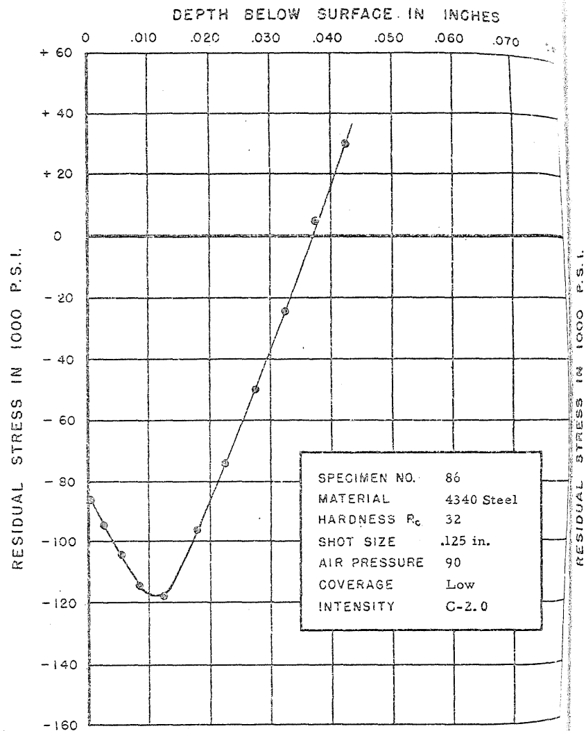
FIGURE 119. RESIDUAL STRESS DISTRIBUTION
