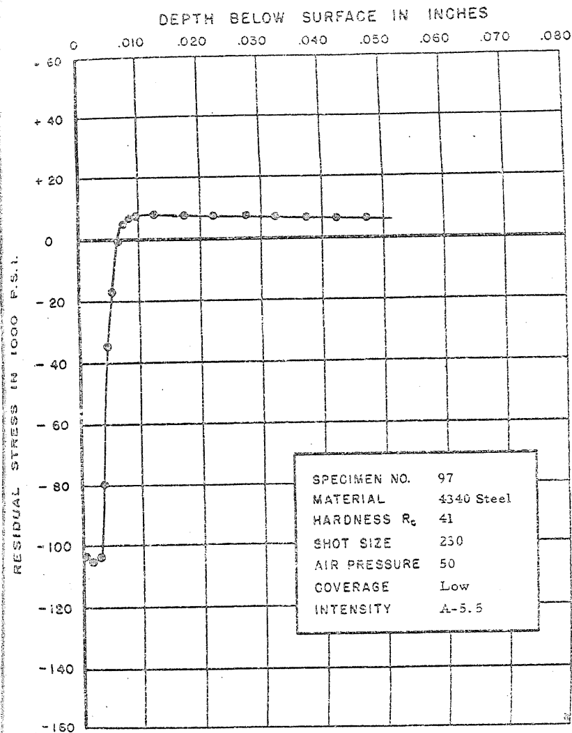
FIGURE 130. RESIDUAL STRESS DISTRIBUTION
