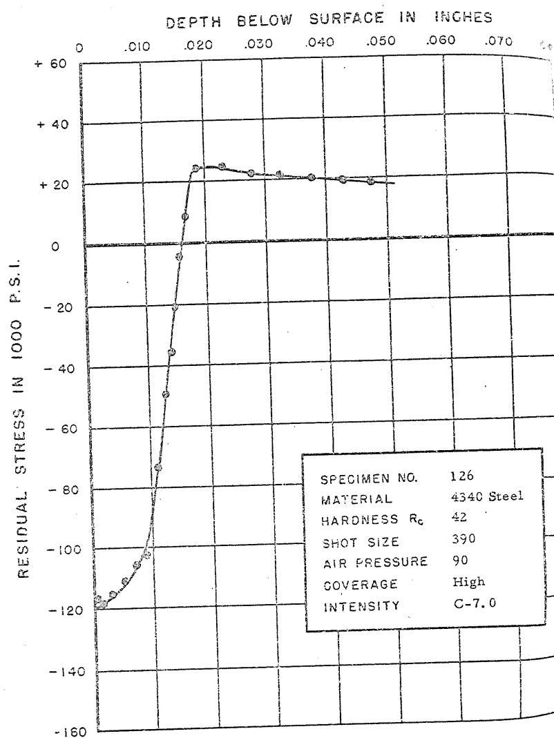
FIGURE 159. RESIDUAL STRESS DISTRIBUTION
