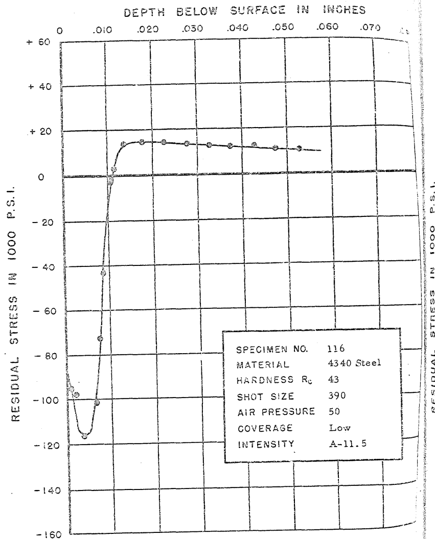
FIGURE 149. RESIDUAL STRESS DISTRIBUTION
