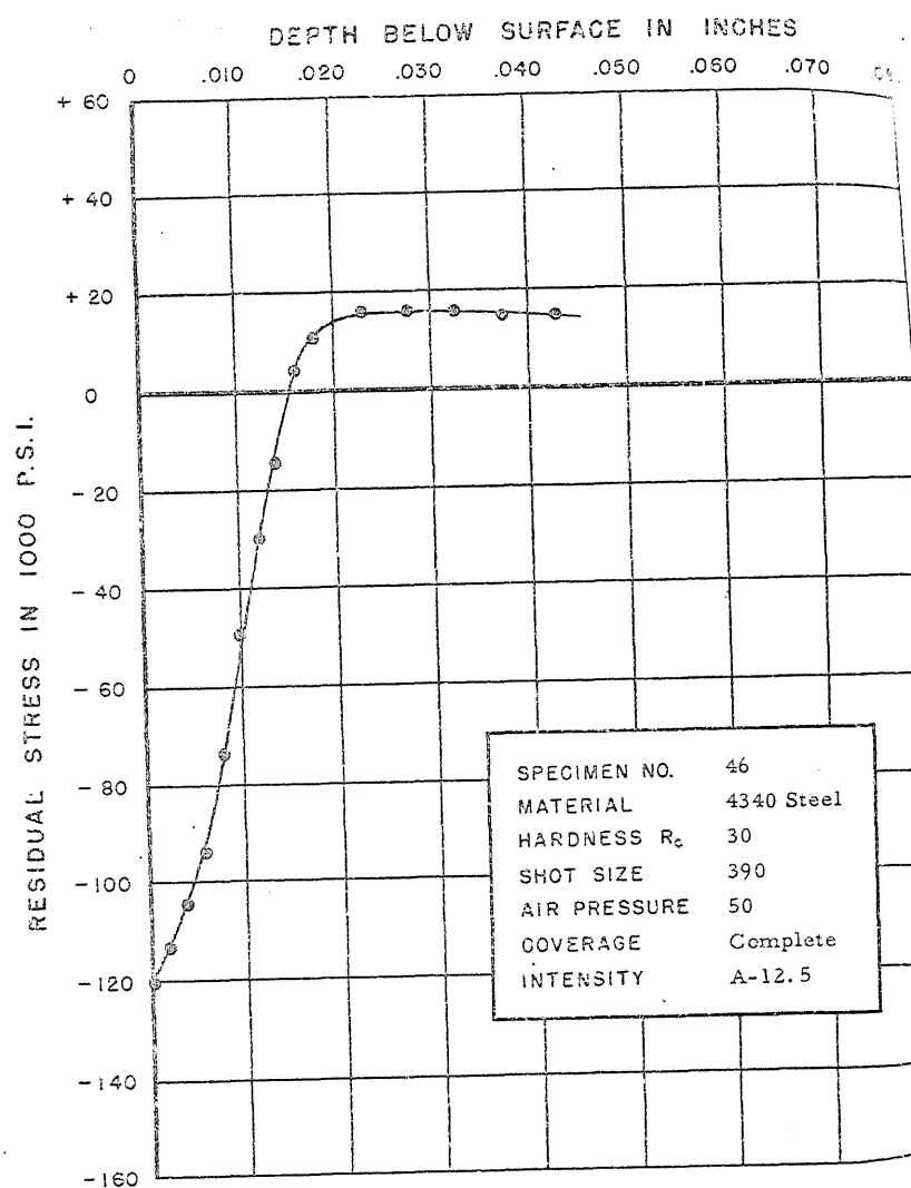
FIGURE 79. RESIDUAL STRESS DISTRIBUTION
