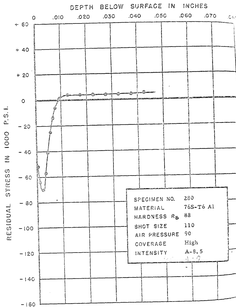
FIGURE 313. RESIDUAL STRESS DISTRIBUTION
