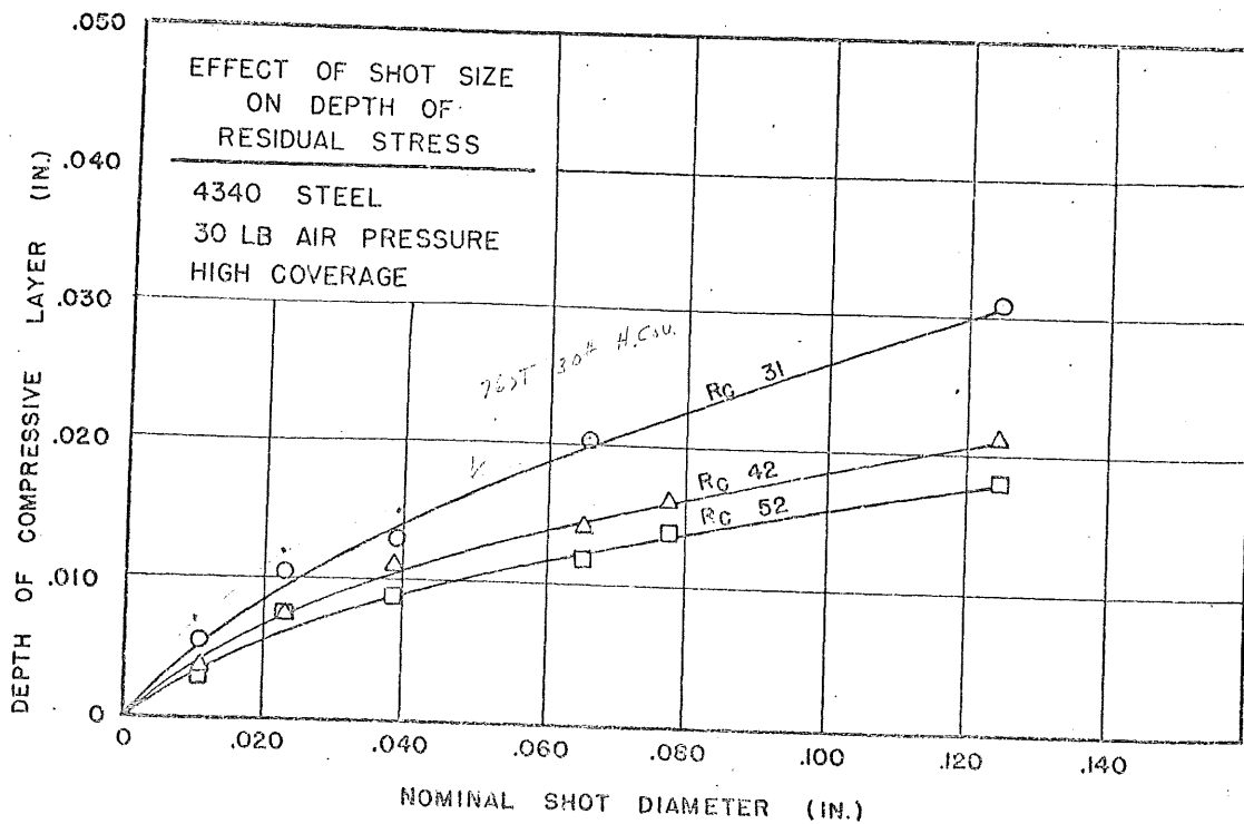
FIGURE 16. EFFECTIVE DEPTH OF PEENING
