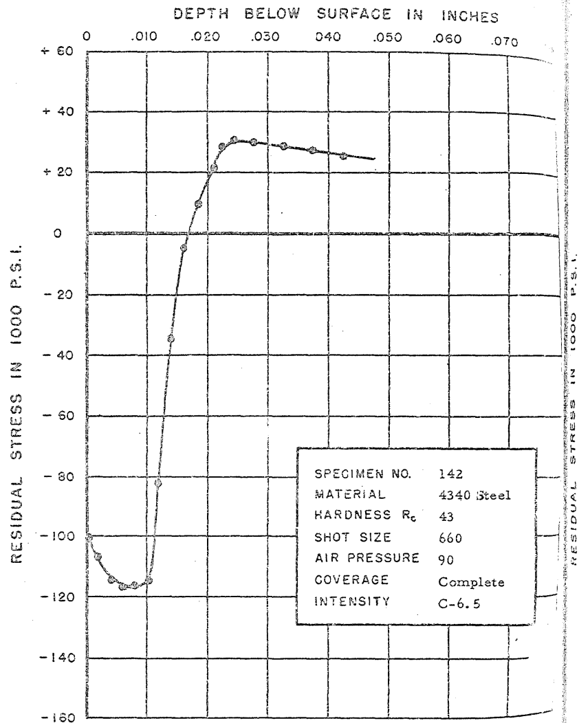
FIGURE 175. RESIDUAL STRESS DISTRIBUTION
