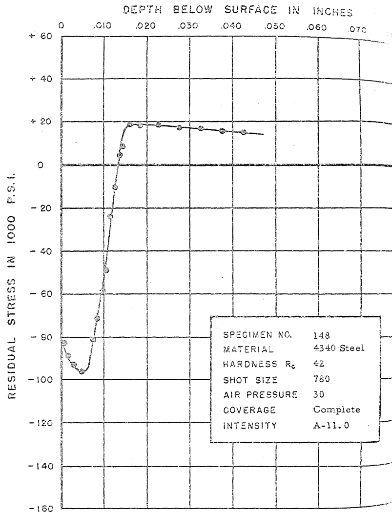
FIGURE 181. RESIDUAL STRESS DISTRIBUTION
