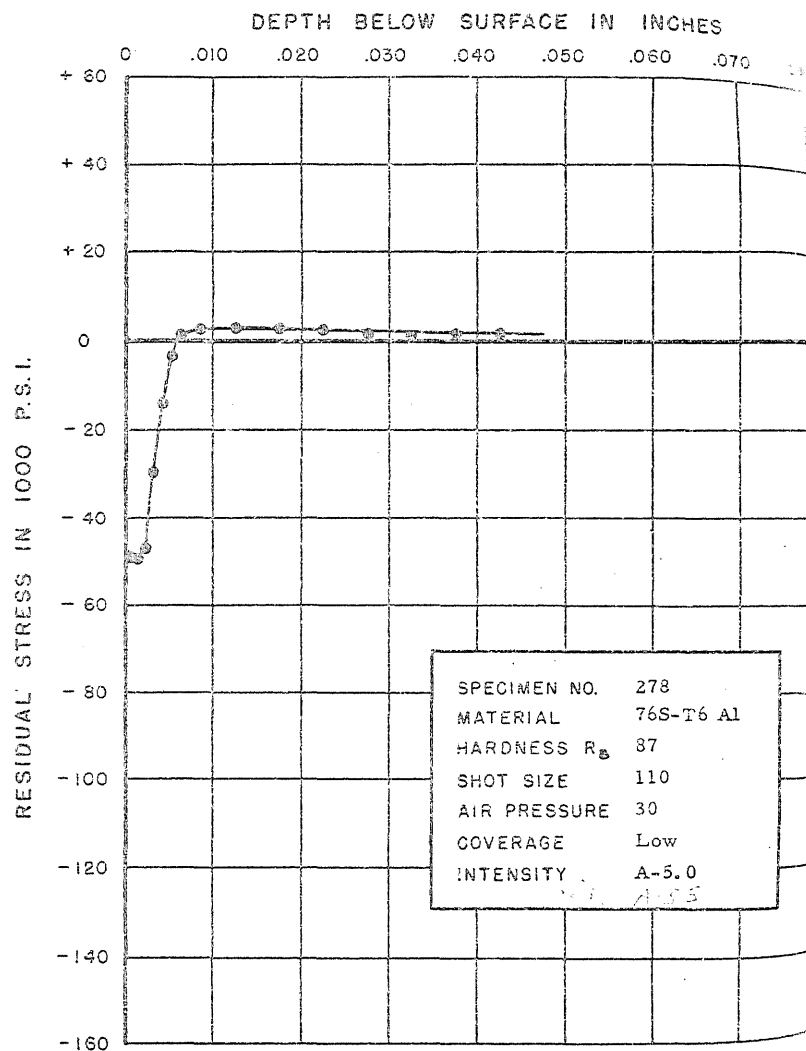
FIGURE 311. RESIDUAL STRESS DISTRIBUTION
