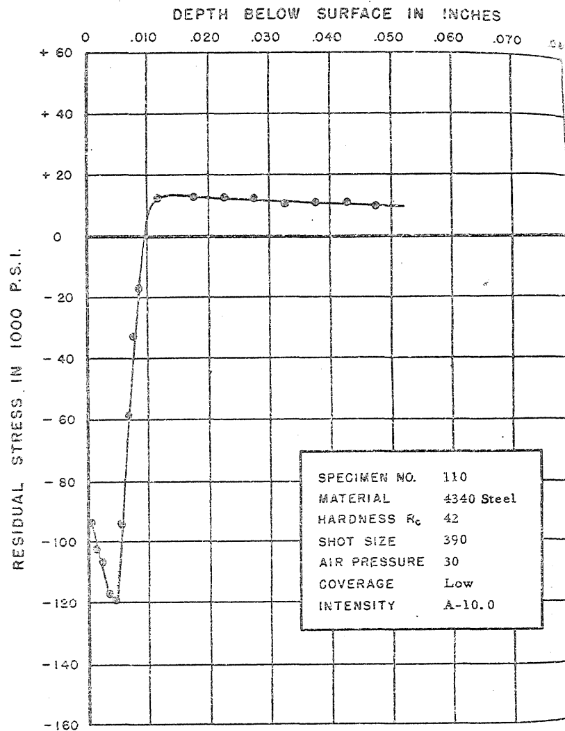
FIGURE 143. RESIDUAL STRESS DISTRIBUTION
