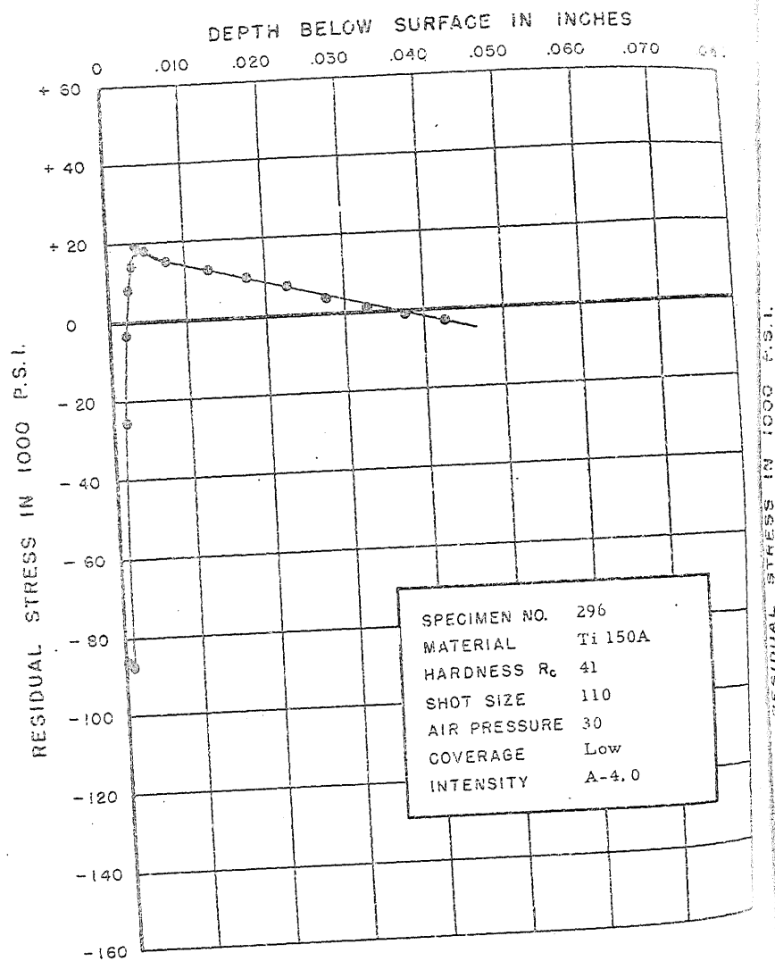
FIGURE 329. RESIDUAL STRESS DISTRIBUTION
