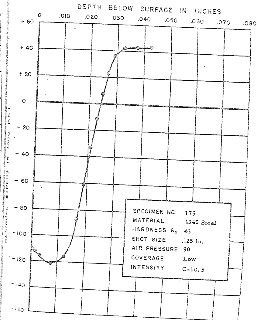
FIGURE 208. RESIDUAL STRESS DISTRIBUTION
