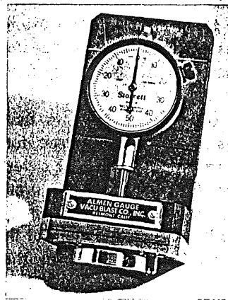
(Above) Distortion of Almen test strips is directly read on a standard gage. (Below) A double helical reduction gear for a large steam turbine is being shot peened to increase fatigue life of the gear teeth. The gear rotates as the blast gun automatically indexes across the front. The machine is a standard Senior Model Vacu-Blaster equipped with a special work table
