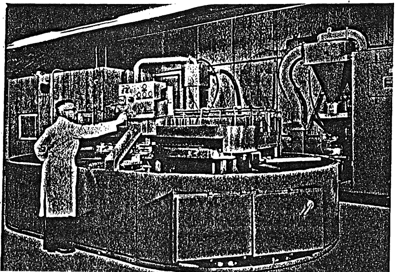
Automatic blast cleaning and shot blasting of jet engine blades was made possible by this new machine developed by Vacu-Blast for United Airlines maintenance headquarters in San Francisco. An automatic transfer line moves the blades from a blast cleaning station into a shot peening area where an automatic adjustment mechanism compensates for different sizes of blades and provides different peening intensities on different sections of each blade. All variables are pre-set at a central control
