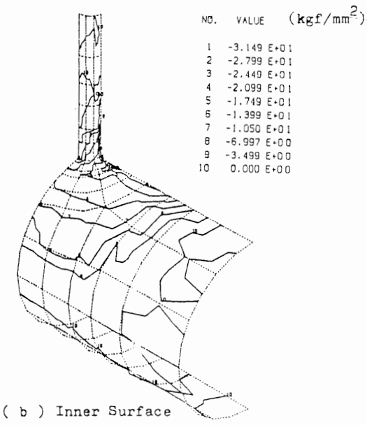
Fig. 15. Residual stress contour for IHSI.
