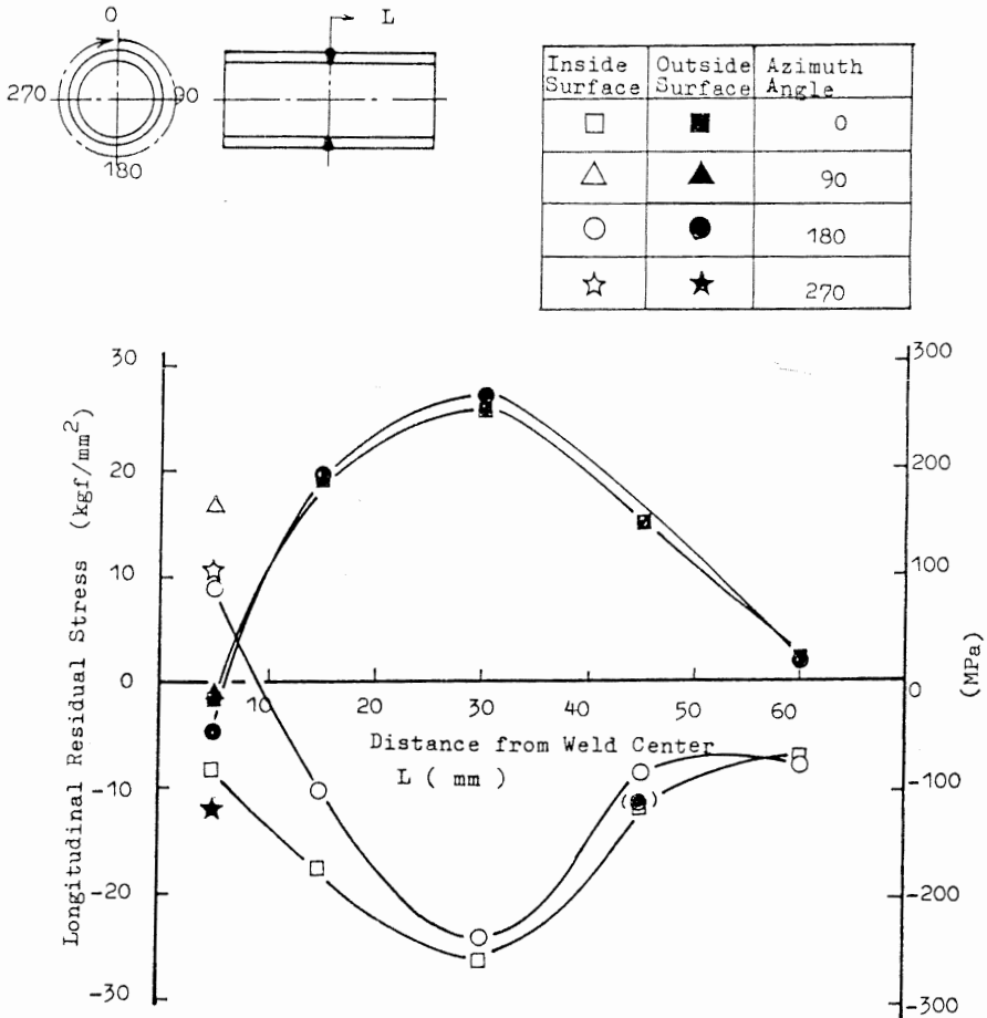
Fig. 5. Longitudinal residual stress distribution (conventional welding).
