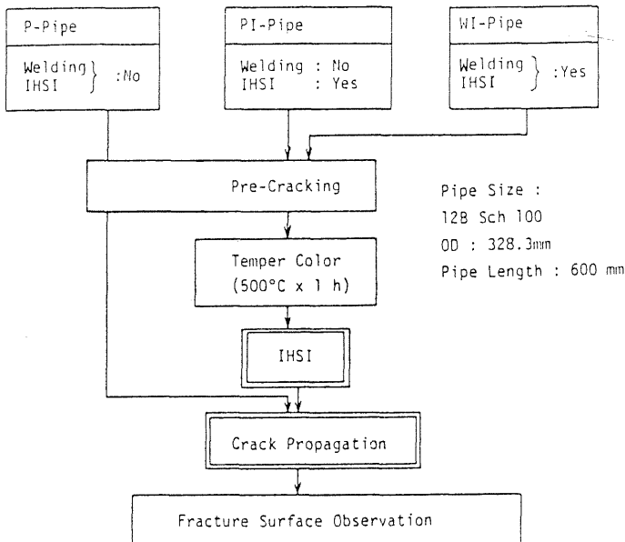
Fig. 10. Experimental procedure.
