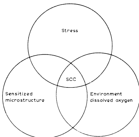
Fig. 1. Parameters influencing IGSCC in type 304 stainless steel.
