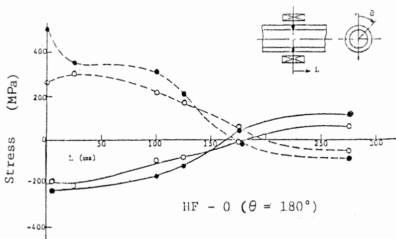
Fig. 9. Residual stress distributions along pipe axis.
