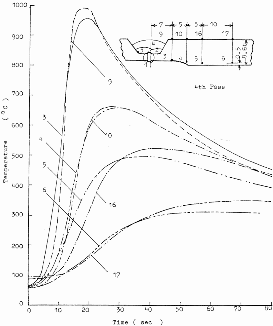
Fig. 3. Temperature profiles along the inside and outside surface of 4B Sch80 pipe (conventional welding).
