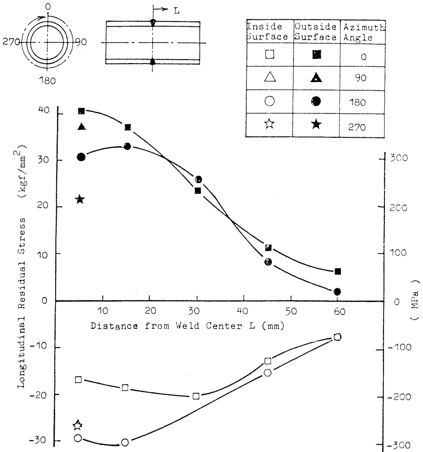
Fig. 6. Longitudinal residual stress distribution (HSW).
