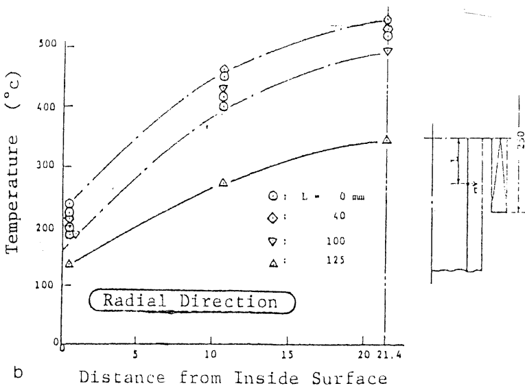
Fig. 8. Temperature distribution of IHSI'd Pipe HF-1.
