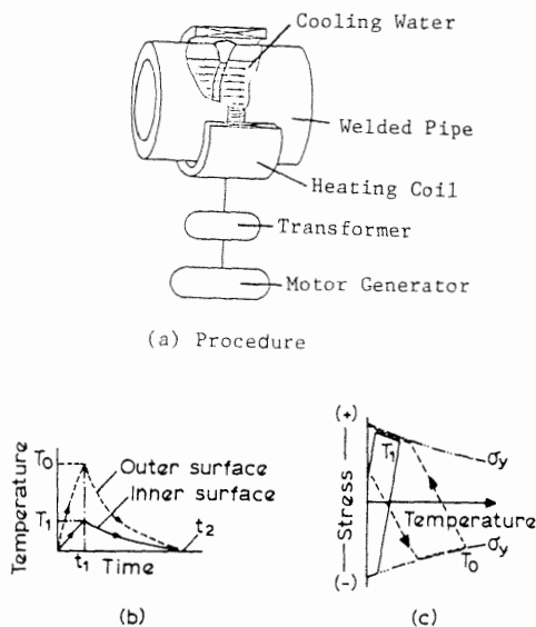
Fig. 7. Induction Heating Stress Improvement (IHSI).
