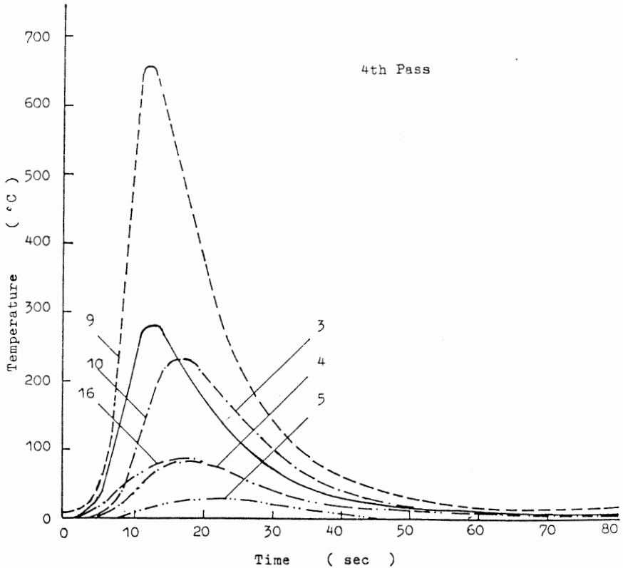
Fig. 4. Temperature profiles along the inside and outside surface of 4B Sch80 pipe (HSW).
