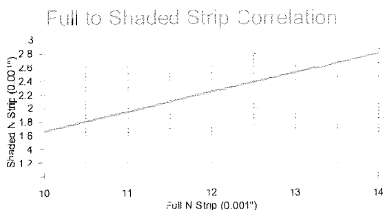
Figure 27. Chart showing correlation between full N Strip readings for shaded N strips
