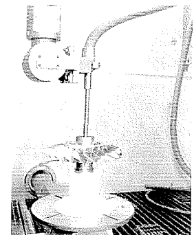
Figure 14. A deflector used for peening a blisk bore
