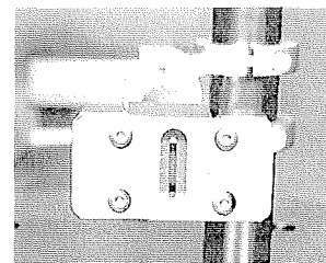
Figure 26. Almen Block with hardened steel mask. Opening simulates the hole diameter
