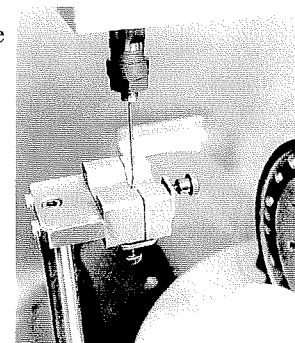
Figure 29. PROGRESSIVE's small hole Almen tooling. A range of hole sizes are available
