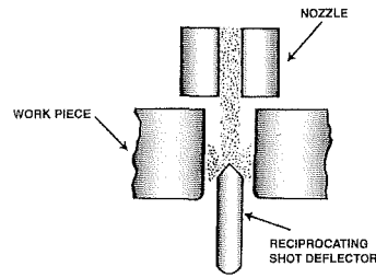
Figure 11. Setup for peening hole ID with nozzle and deflector pin.
