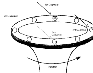
Figure 4. Schematic showing method for quadrant peening bolt holes on a rotating flange. Each nozzle position targets 1/4 of the hole diameter, shown as different colors for each position
