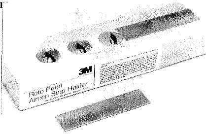
Figure 7. Special Almen Fixture for Roto Peening
