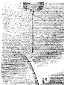
Figure 22. Peening a turbine shaft oil hole (0.140" diameter)
