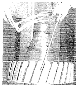
Figure 17. Rotary Lance peening of a fan hub dovetail slot
