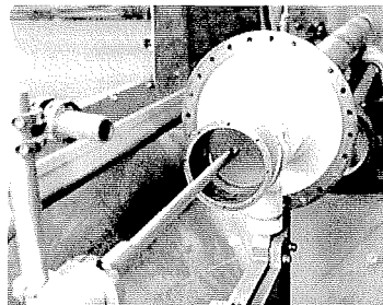
Figure 13. Peening a turbine shaft bearing journal using a deflector lance. Note that the part must rotate to provide proper coverage
