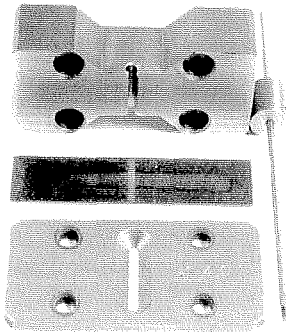
Figure 30. Mask plate for 0.14" hole, simulated hole fixture, peened strip and small rotary lance
