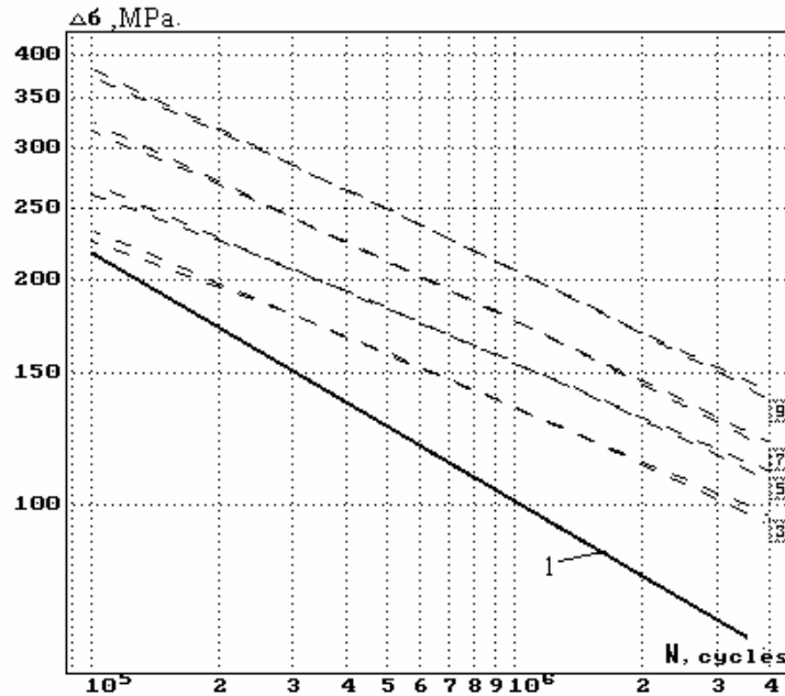
Figure 5. Fatigue curves of non-load-carrying fillet welded joint:
