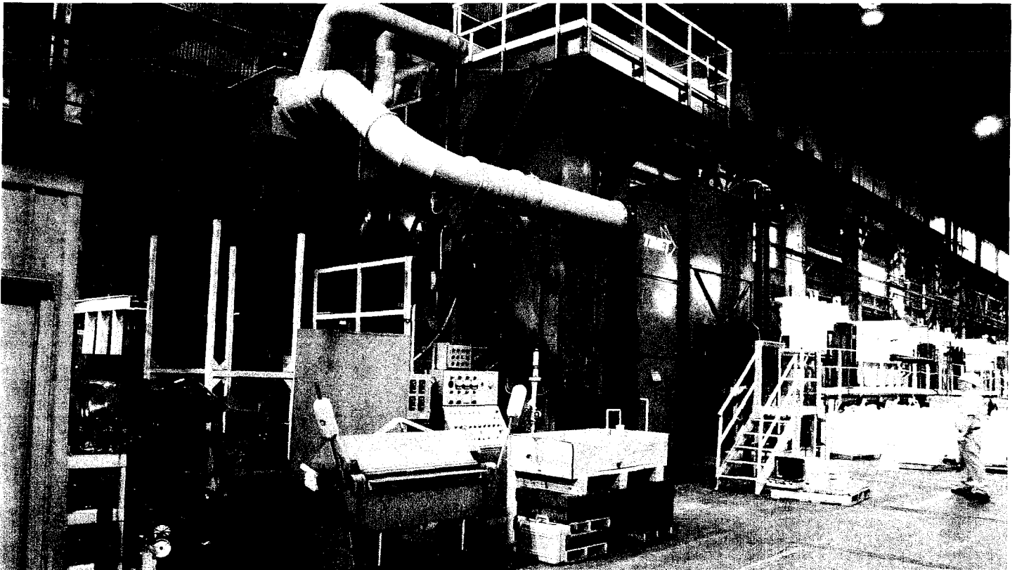
The retrofitted blast cleaning machine at Timet descales coils of titanium.
