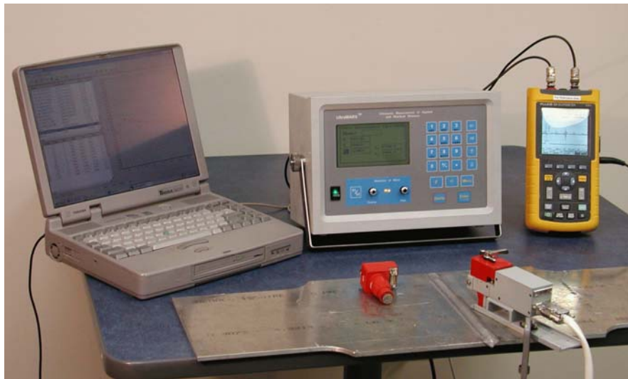
Figure 3. The Ultrasonic Computerized Complex for measurement of residual and applied stresses
